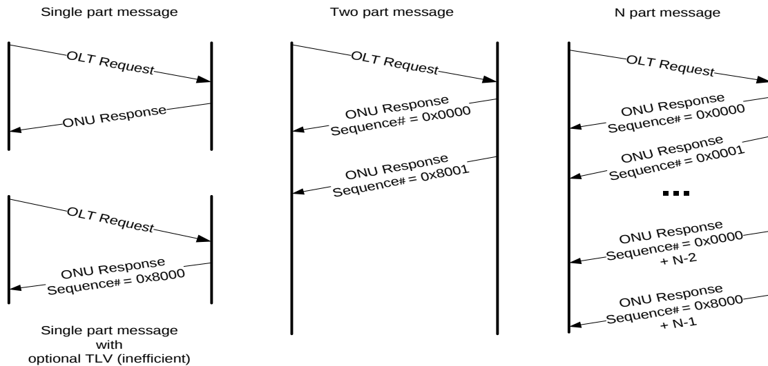
Figure 6 - Sample Message Exchange
