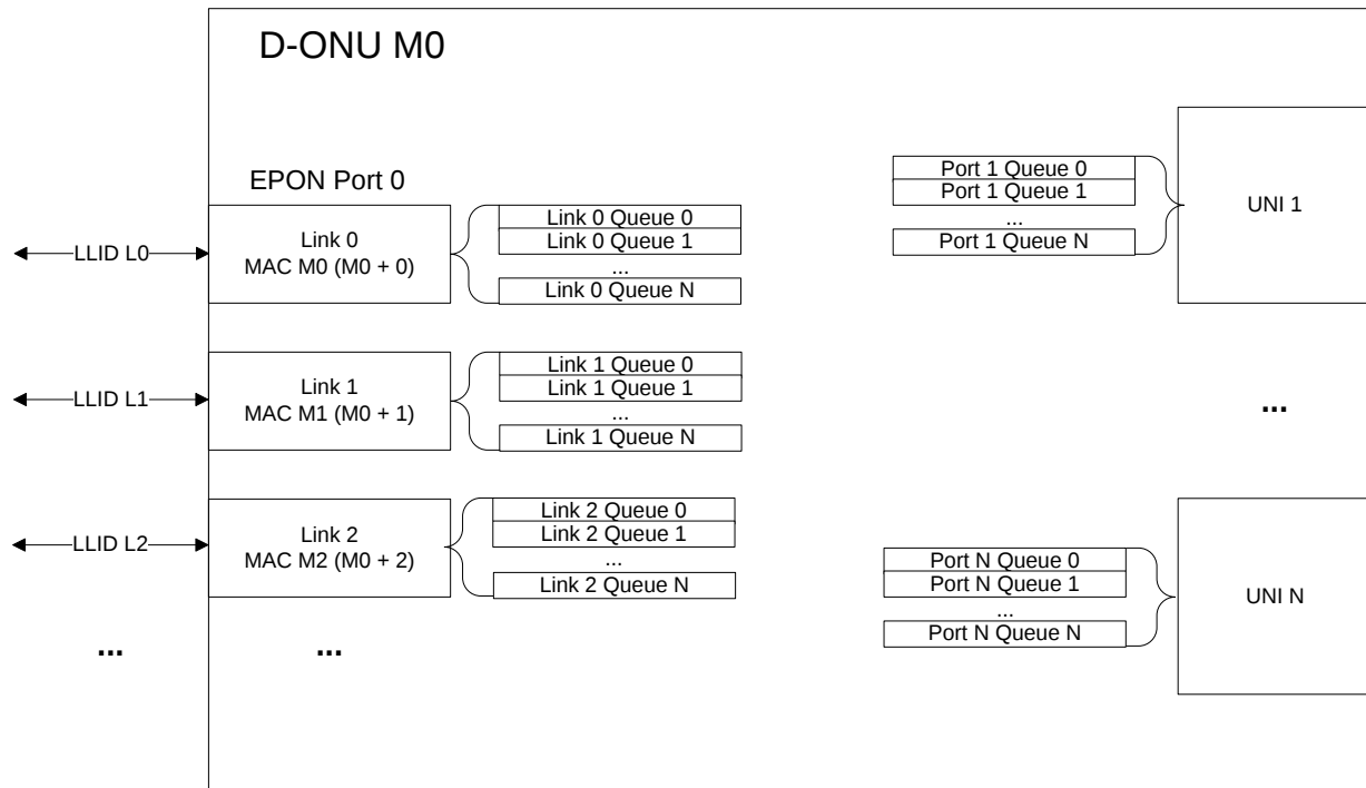
Figure 5 - D-ONU Model
