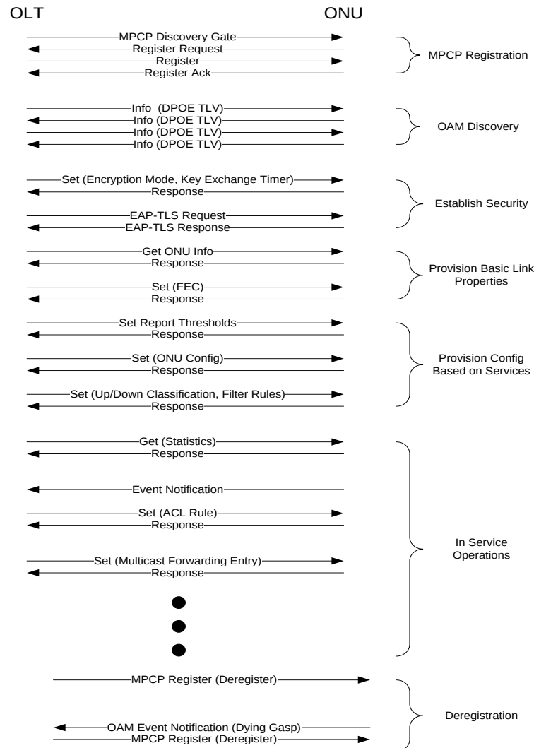
Figure 27 - Unicast Logical Link Life Cycle
