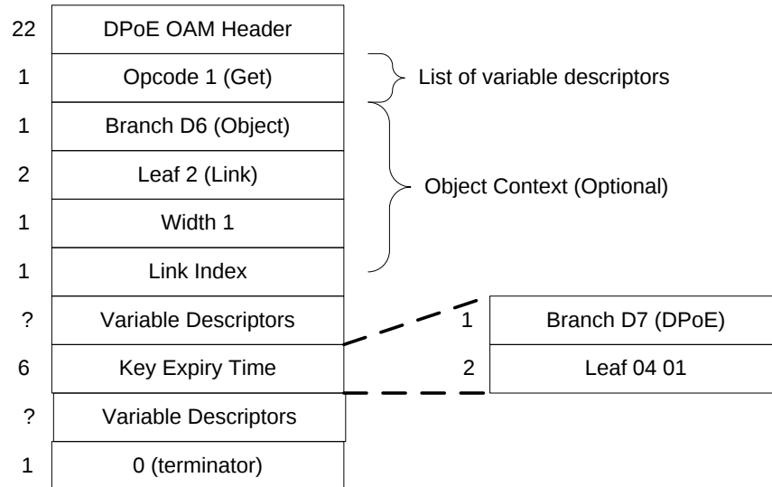
Figure 25 - Get Key Exchange Timer PDU
