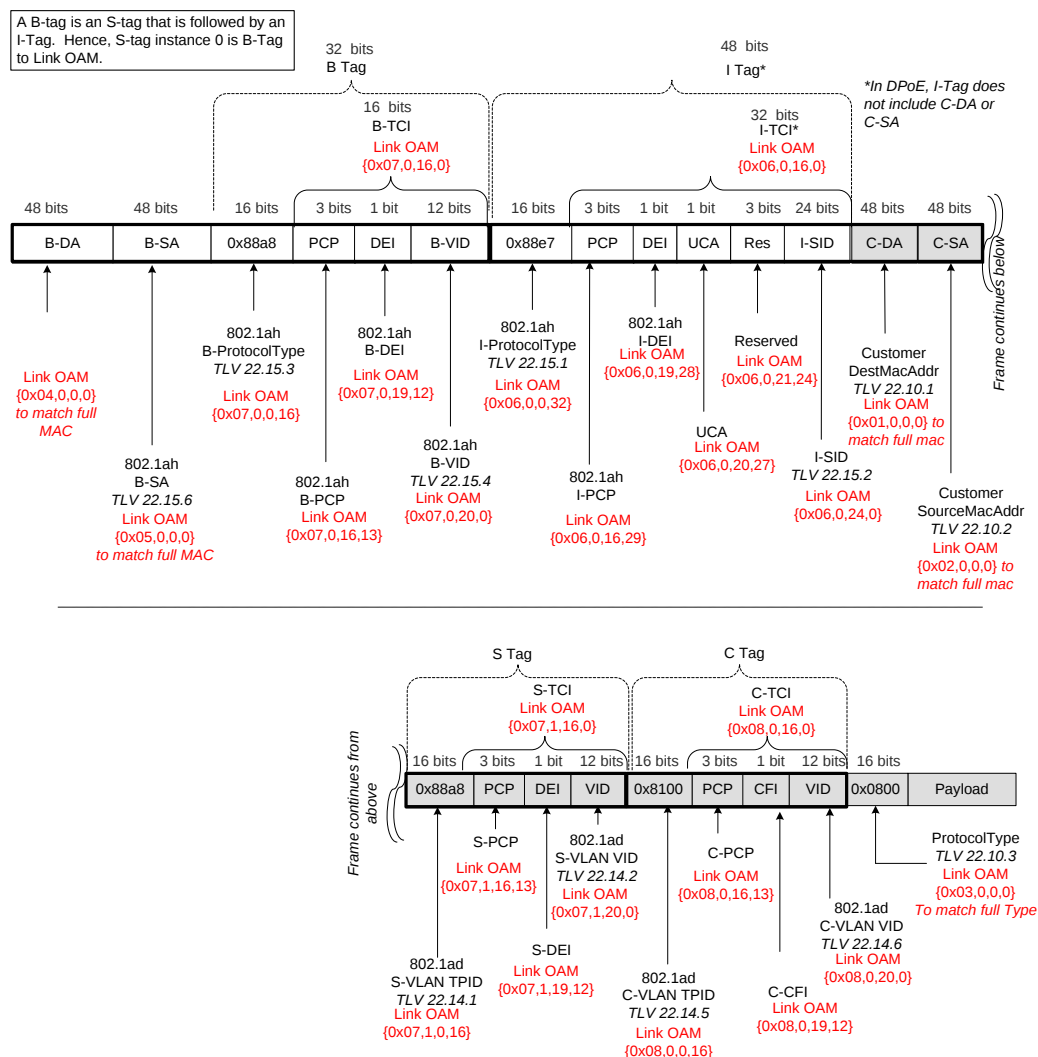
Figure 31 - Field Masking Example for 802.1ah Encapsulated 802.1ad Tagged Frame
