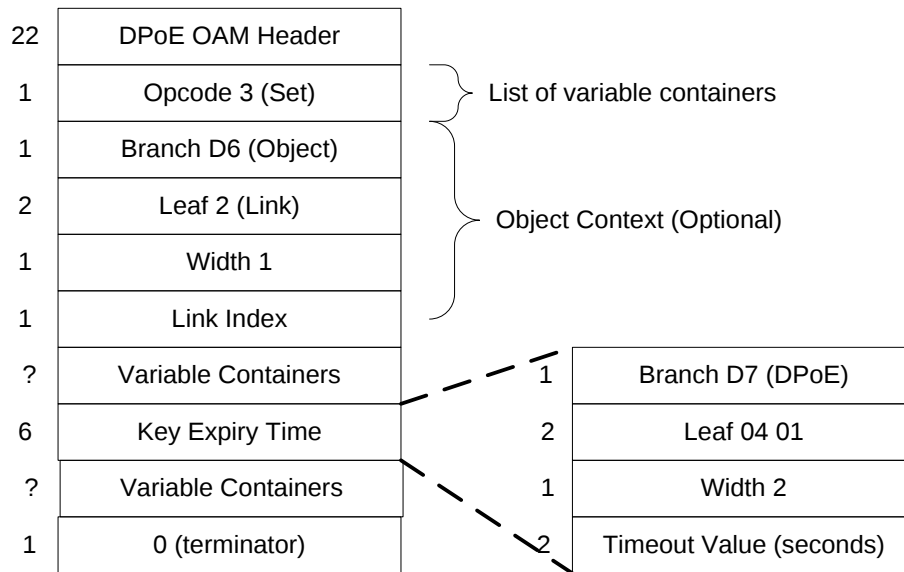
Figure 23 - Set Key Exchange Timer Request PDU
