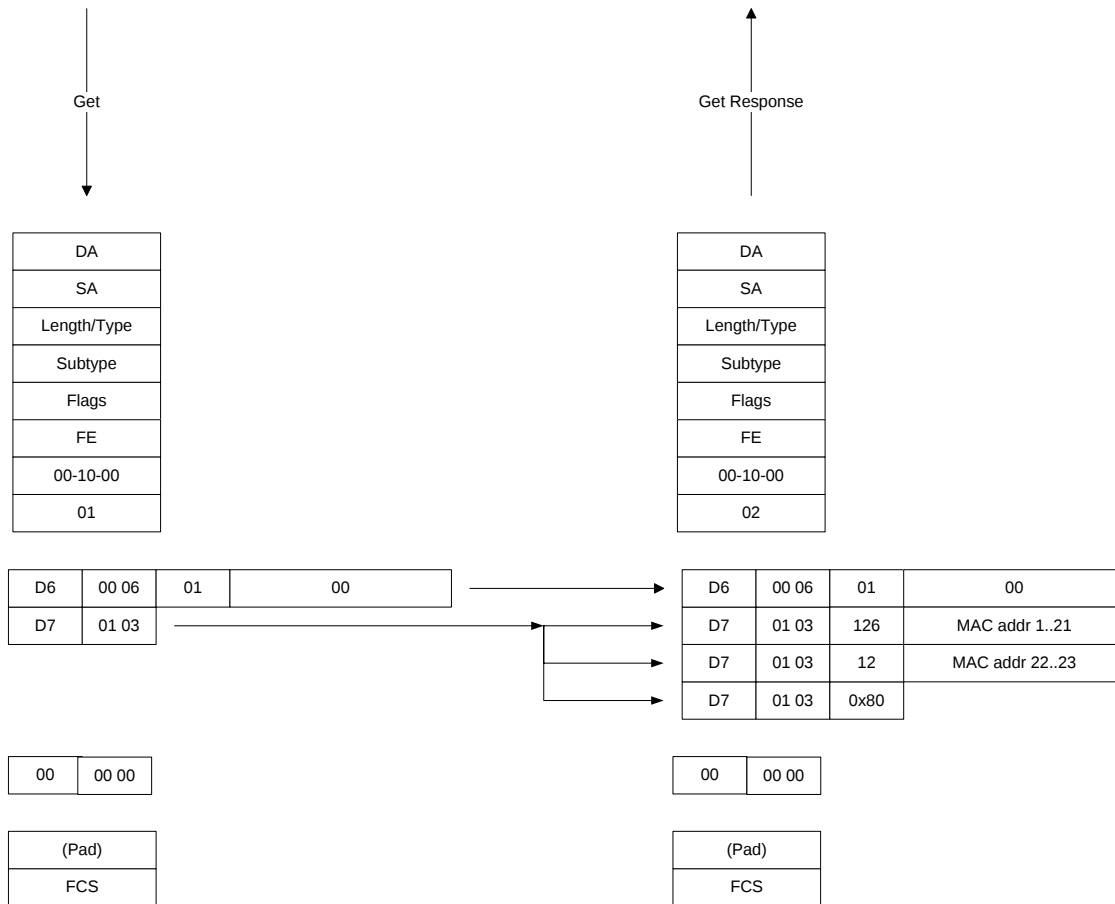
Figure 21 - Large Attribute Values
