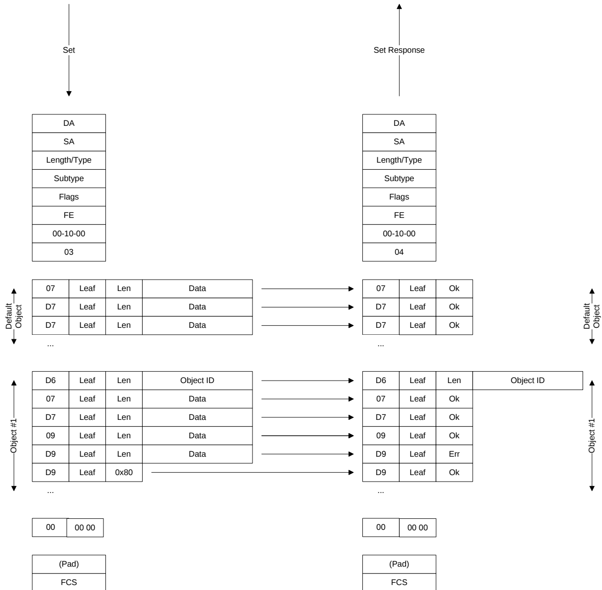
Figure 20 - Set and Set Response
