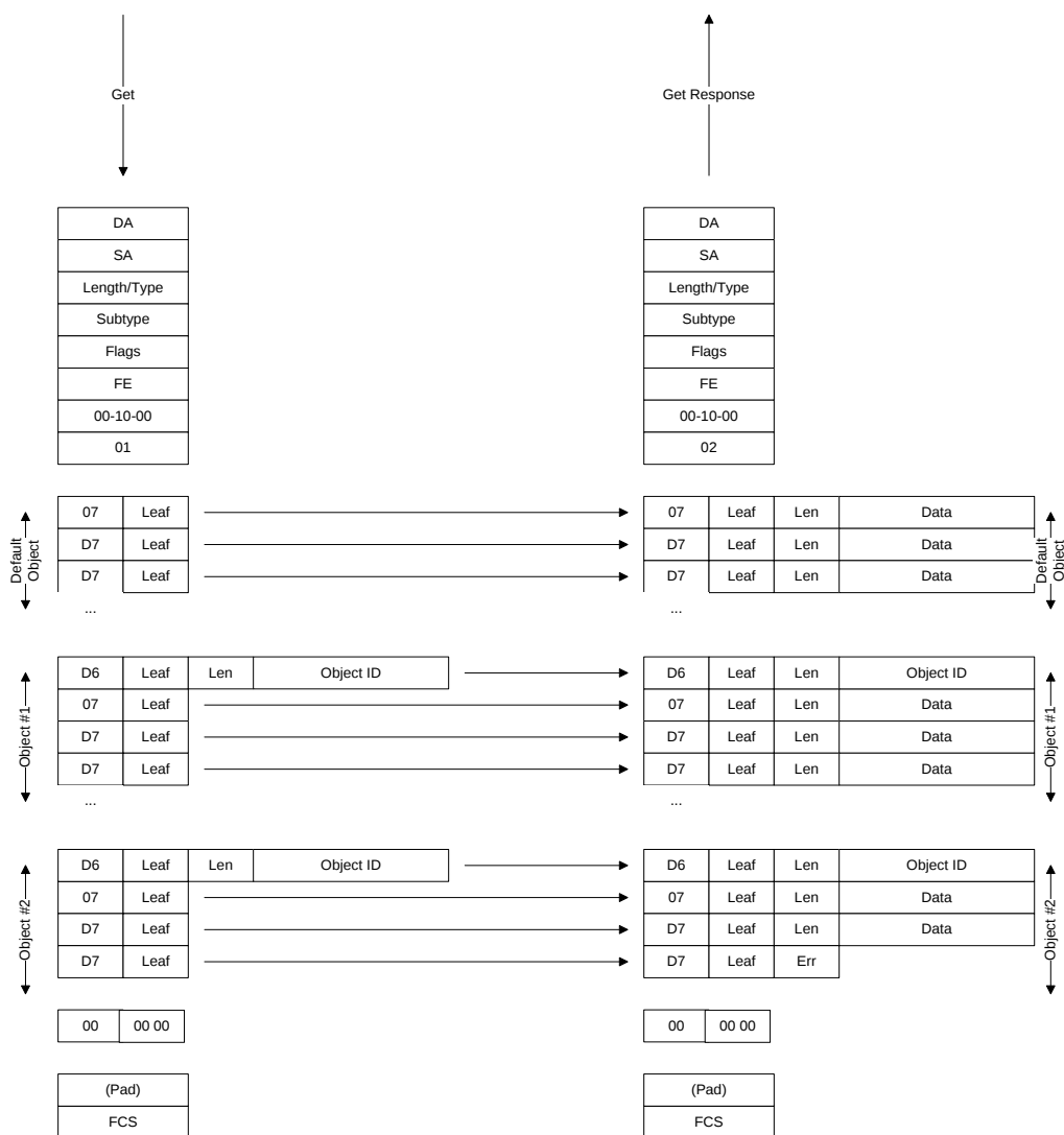
Figure 19 - Get and Get Response
