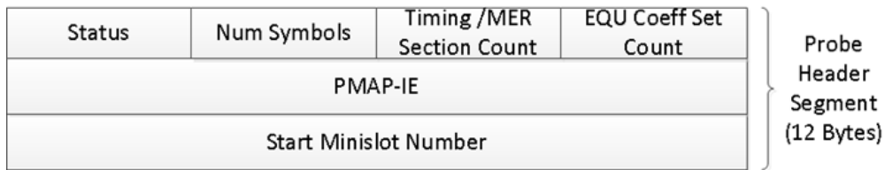
Figure 20 - UEPI Probe Pseudowire Header Segment
