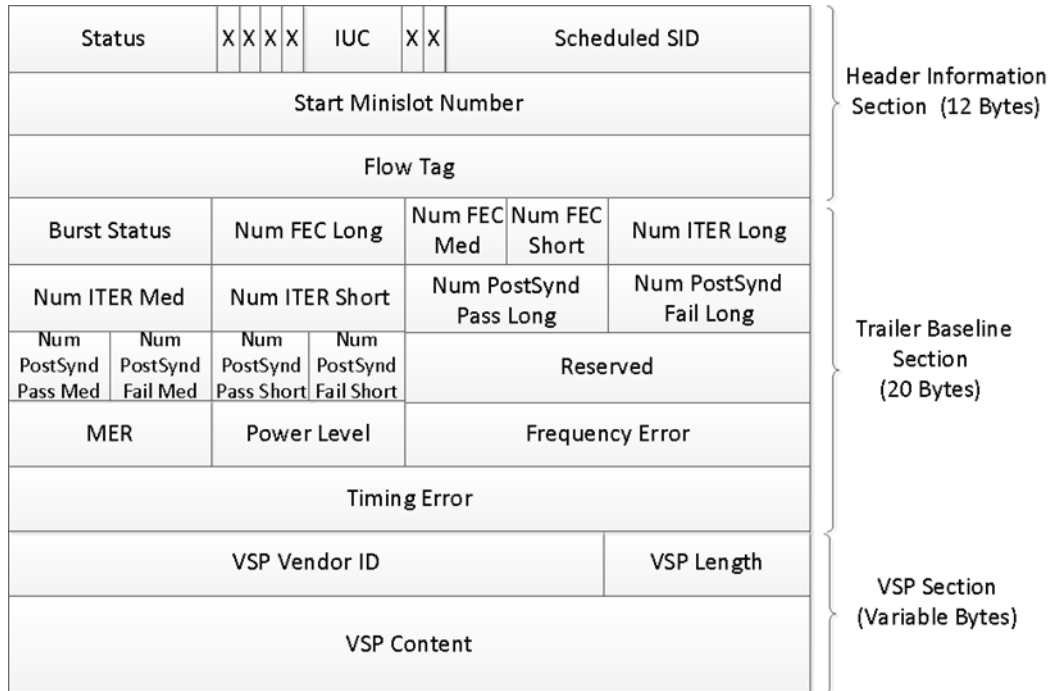
Figure 11 - UEPI Trailer Segment Format
