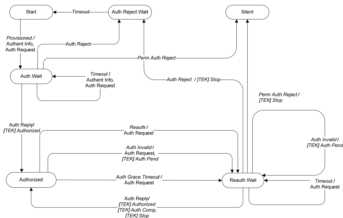
Figure 4–1 - Authorization State Machine Flow Diagram
