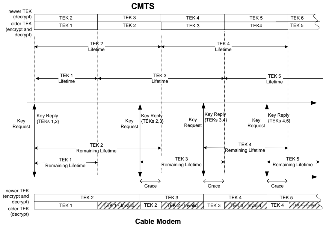
Figure 6-2 - TEK Management in CMTS and CM
