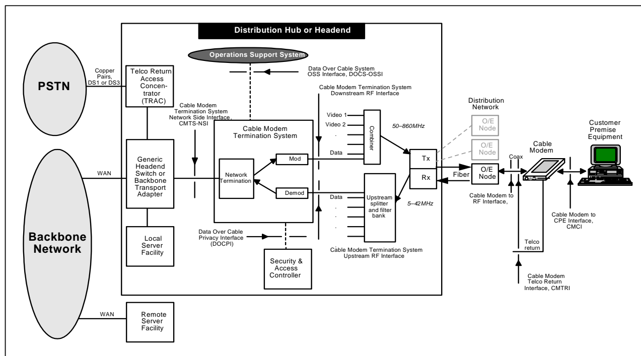
Figure 1-2 - Data-over-Cable Reference Architecture
