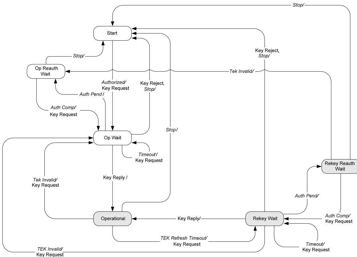
Figure 4–2 - TEK State Machine Flow Diagram
