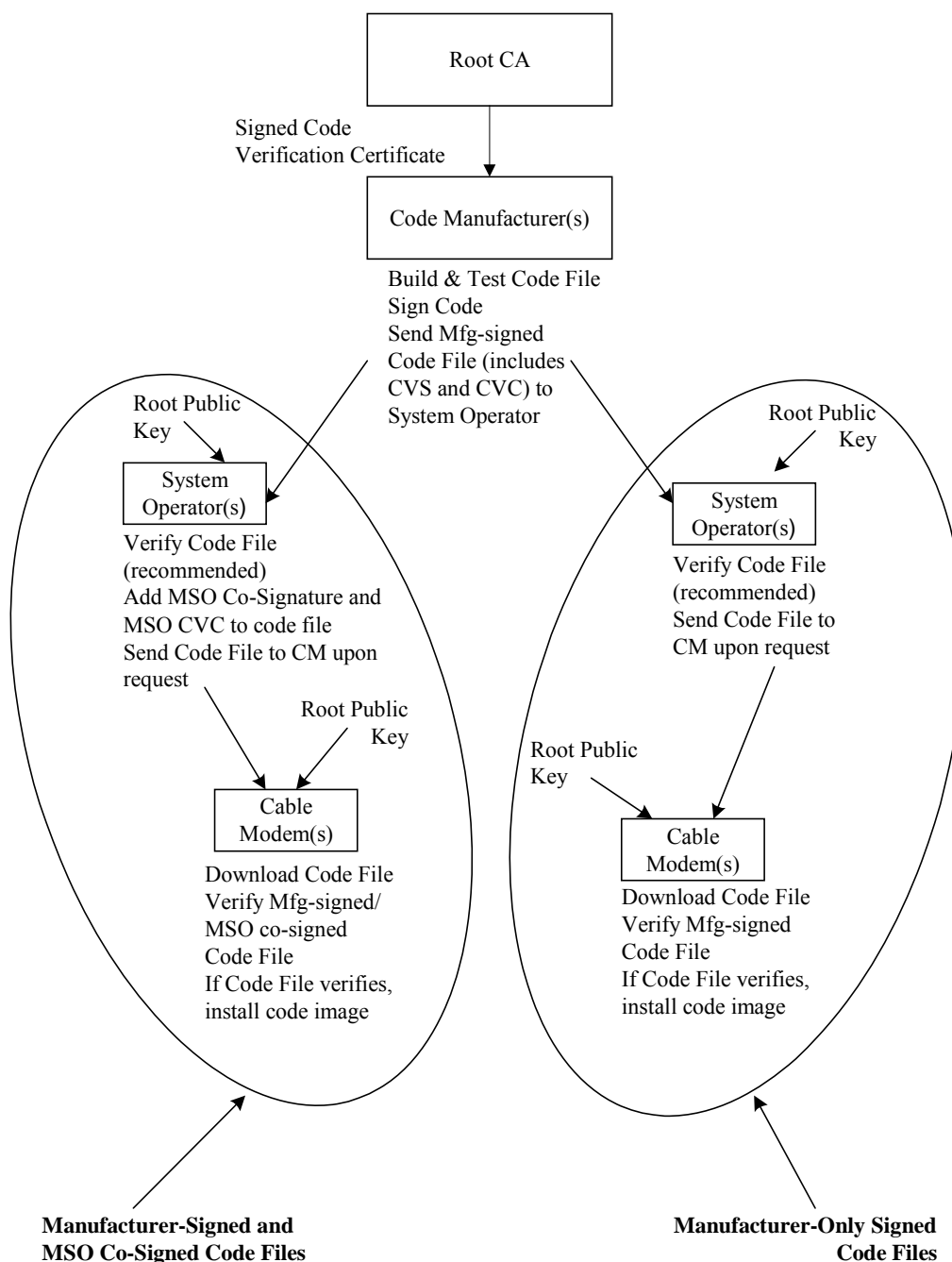
Figure D-1 - Typical Code Validation Hierarchy
