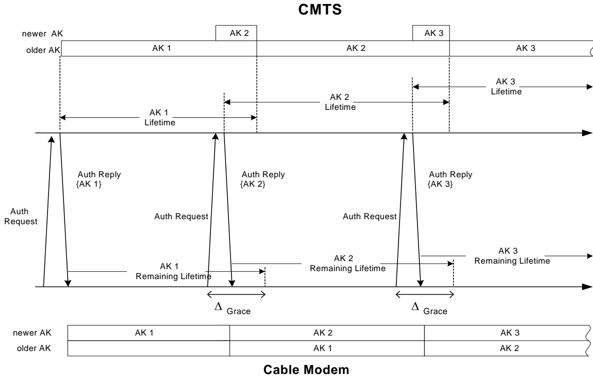
Figure 6-1 - Authorization Key Management in CMTS and CM
