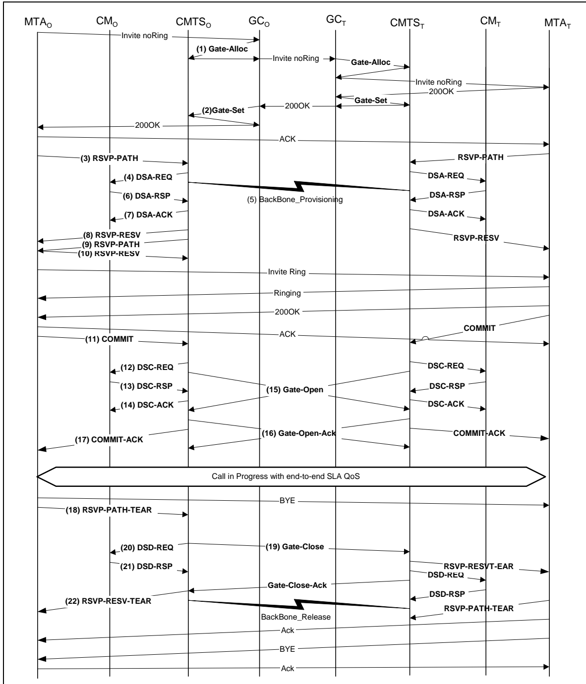
Figure 34. Basic Call Flow – Embedded MTA
