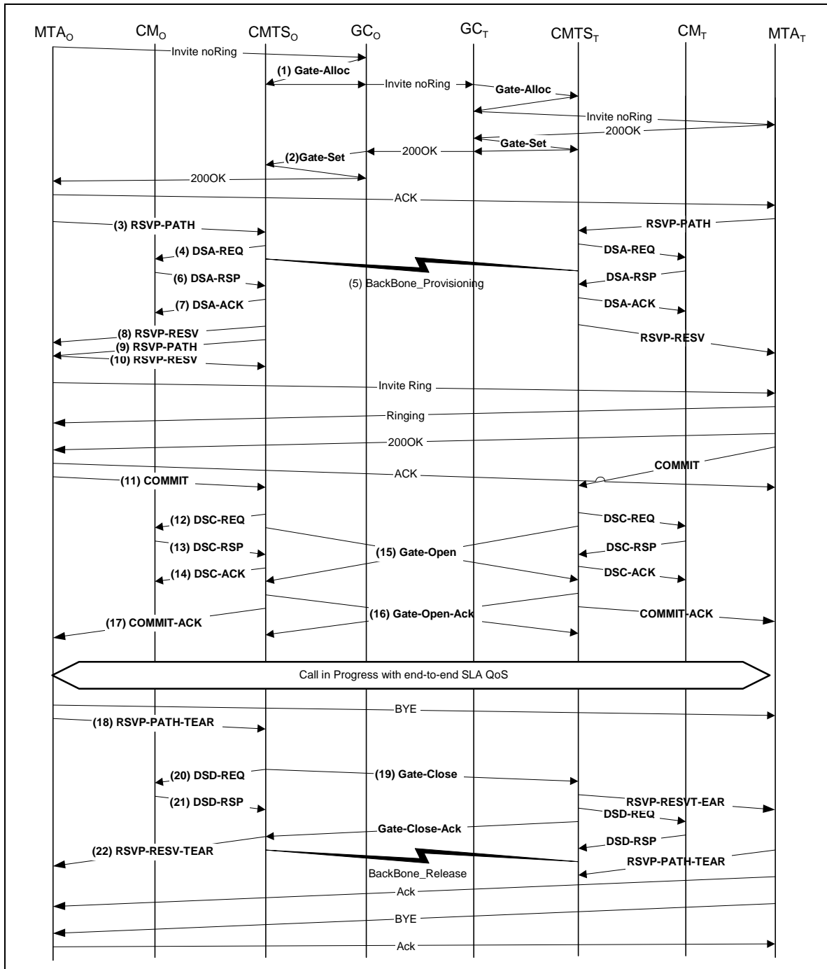
Figure 28. Basic Call Flow - DCS Signaling
