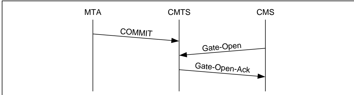
Figure 26. Gate Coordination at Time of COMMIT
