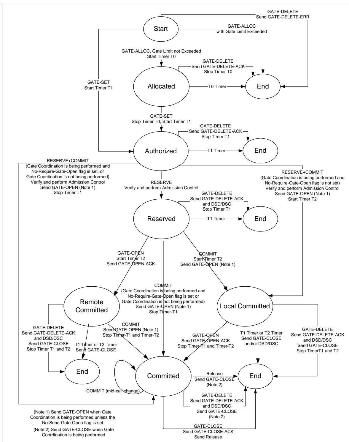
Figure 14. Gate State Transition Diagram 56
