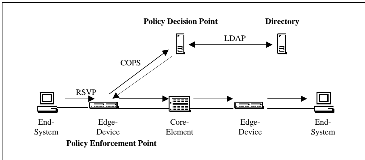
Figure 40. COPS and LDAP model
