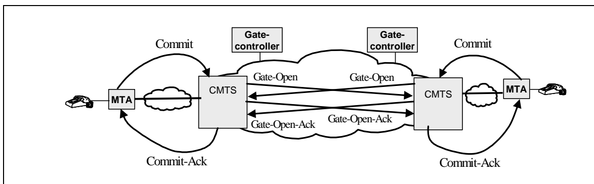
Figure 22. End-to-End Gate Coordination
