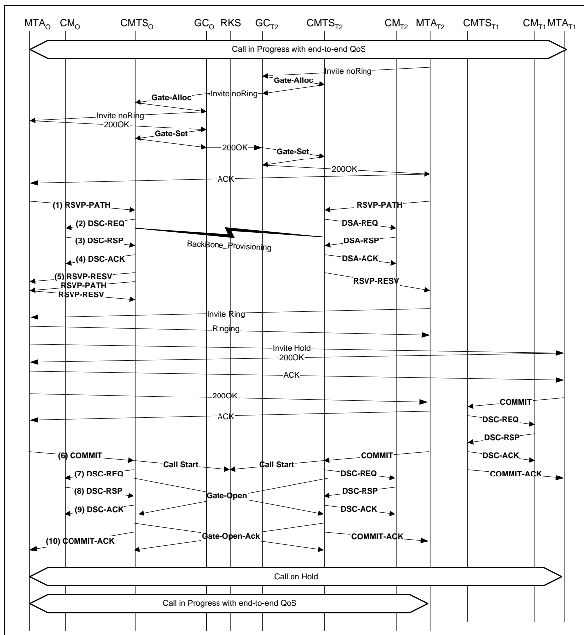
Figure 32. QoS Signaling for Call Waiting
