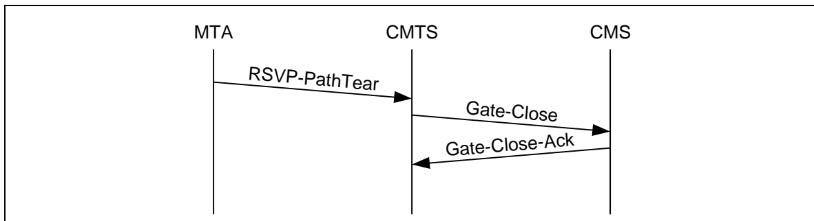
Figure 27. Gate Coordination on Release
