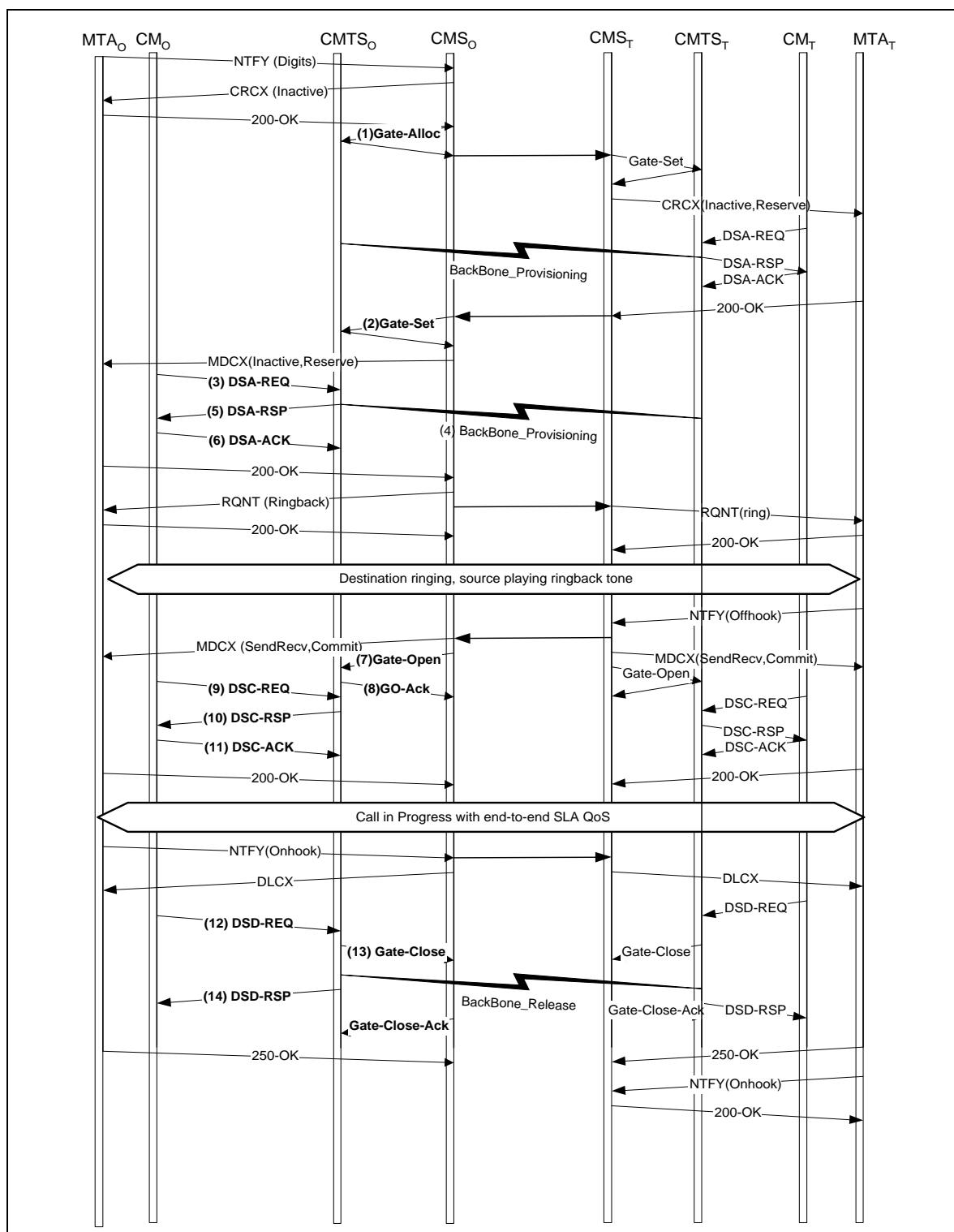
Figure 35. On-Net to On-Net Embedded NCS Call
