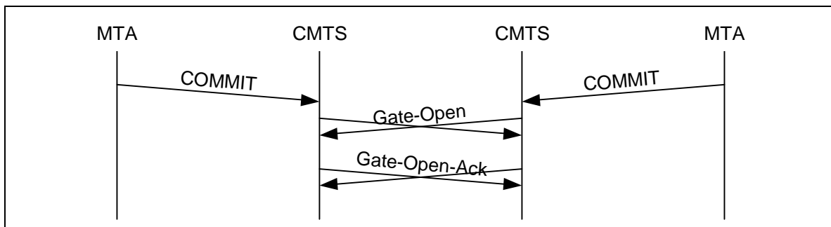
Figure 24. Gate Coordination at Time of COMMIT
