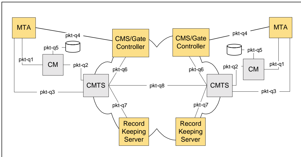
Figure 1. QoS Signaling Interfaces in PacketCable Network
