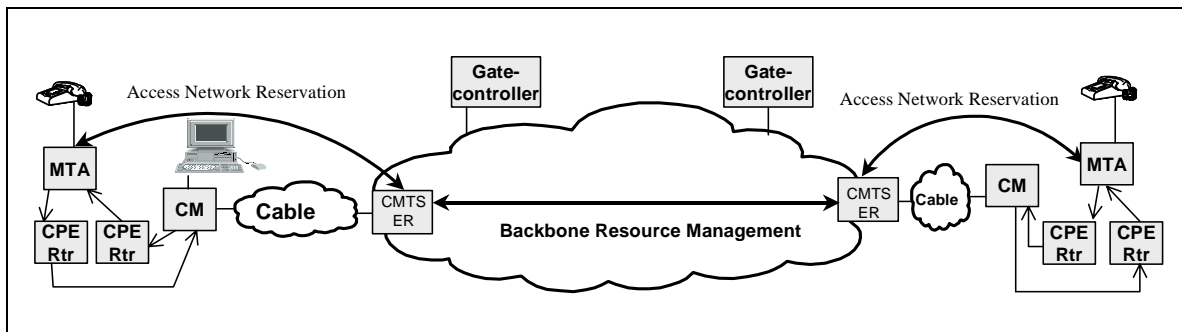
Figure 2. Session Framework
