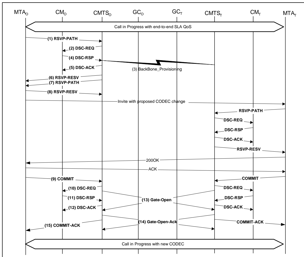
Figure 30. QoS Signaling for Codec Change
