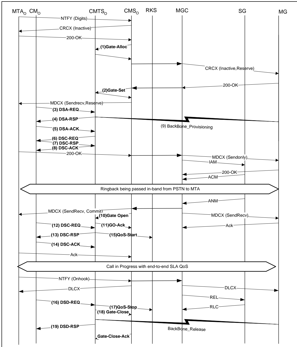
Figure 36. On-net to Off-net Embedded NCS
