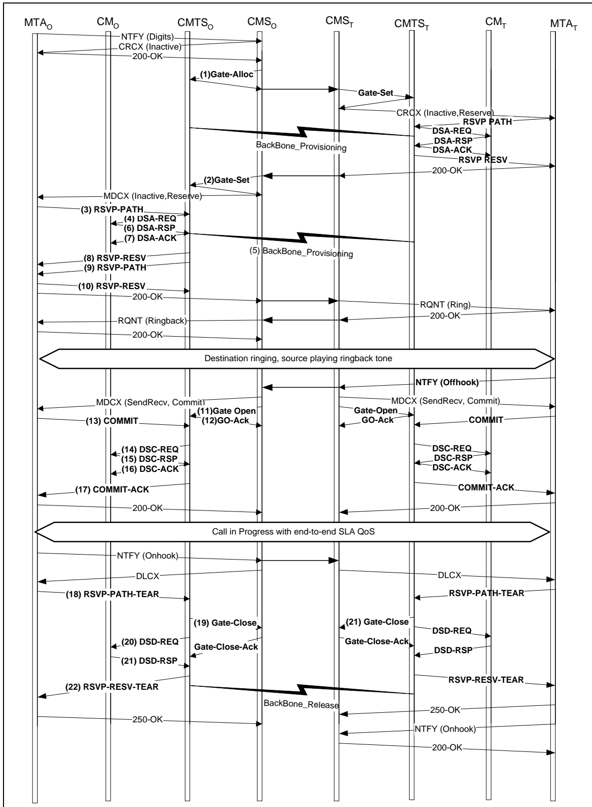
Figure 29. Basic Call Flow – On-net to On-net using NCS and RSVP
