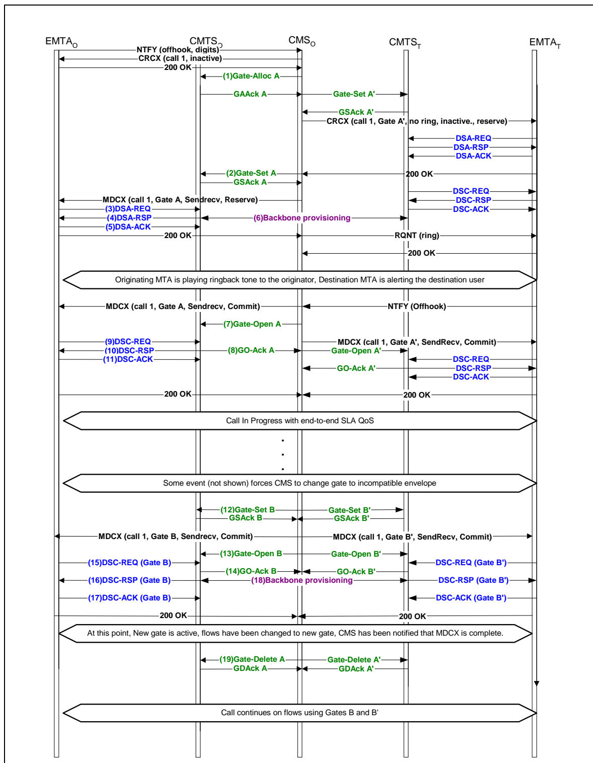
Figure 37. On-Net to On-Net Embedded NCS Call
