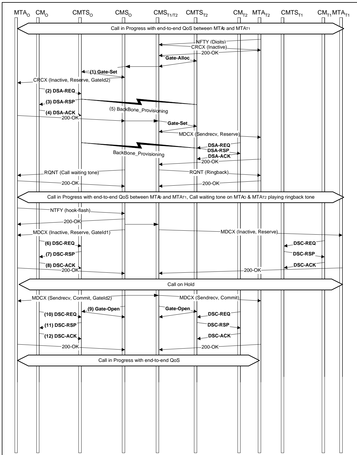
Figure 33. Call Waiting using NCS
