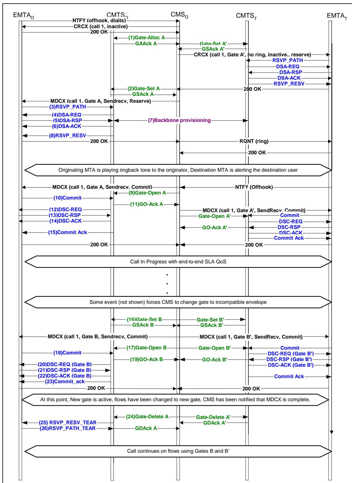
Figure 38. On-Net to On-Net Embedded NCS Call Using RSVP
