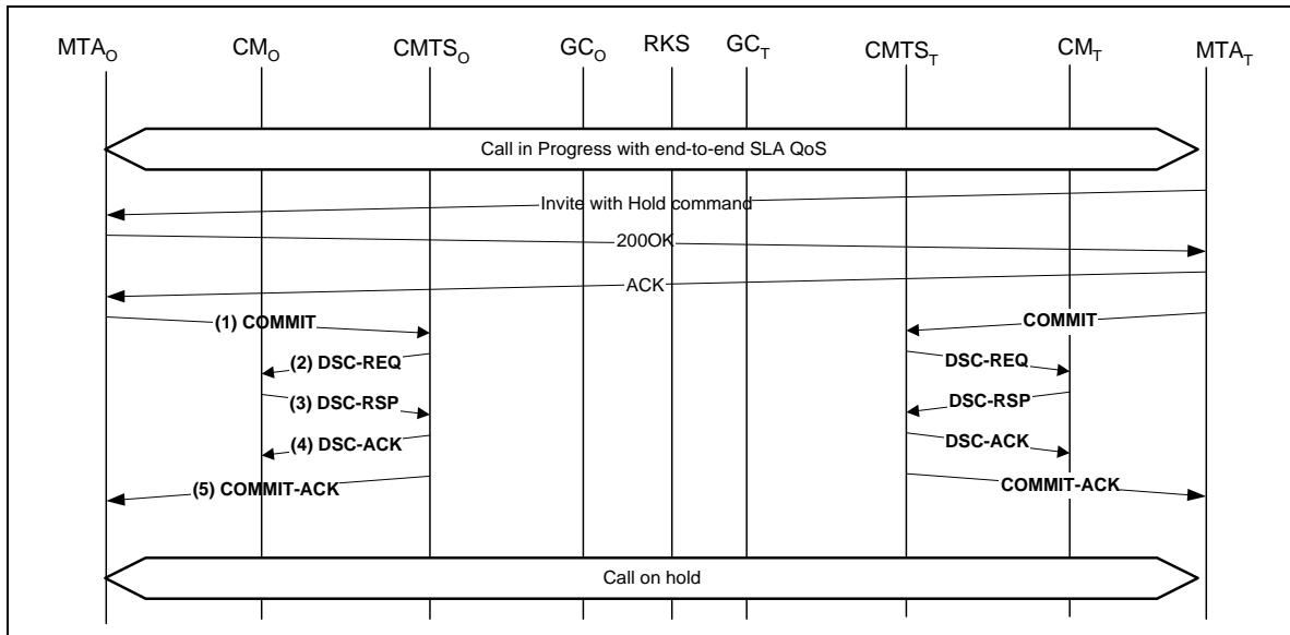
Figure 31. QoS Signaling for Call Hold
