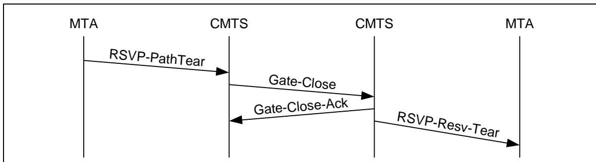
Figure 25. Gate Coordination on Release
