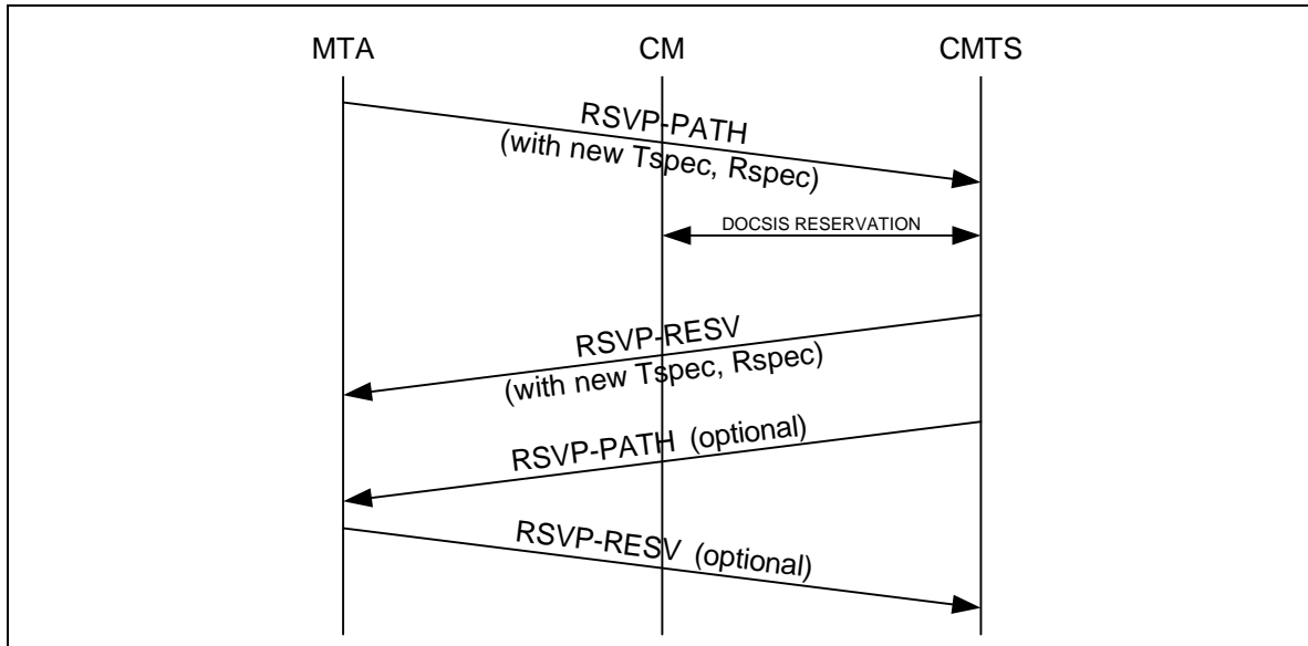
Figure 9. Reservation Change
