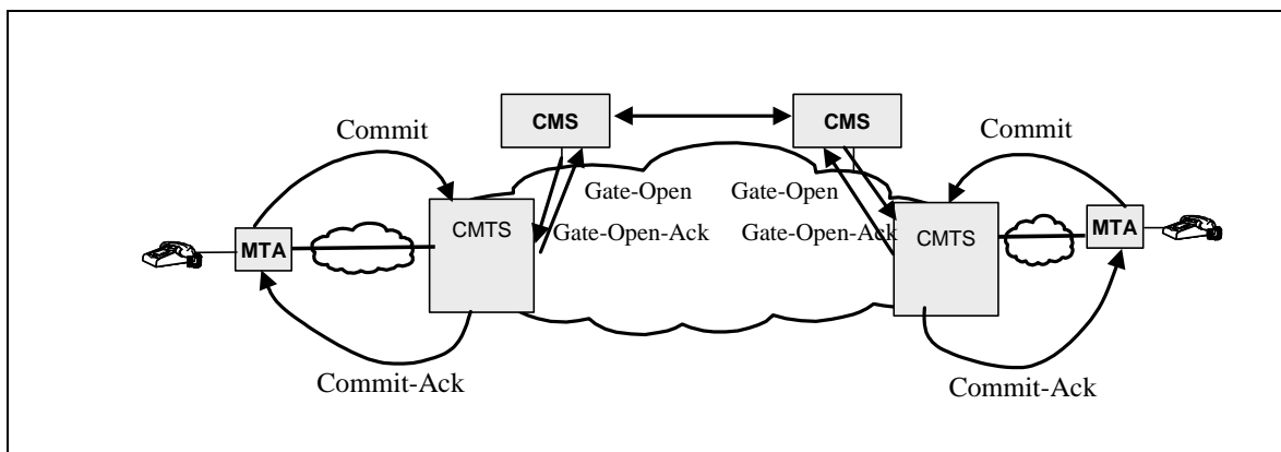
Figure 23. CMS-Proxied Gate Coordination
