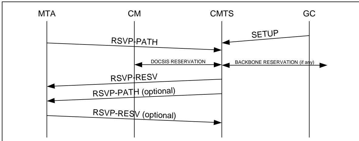
Figure 8. Reservation Establishment
