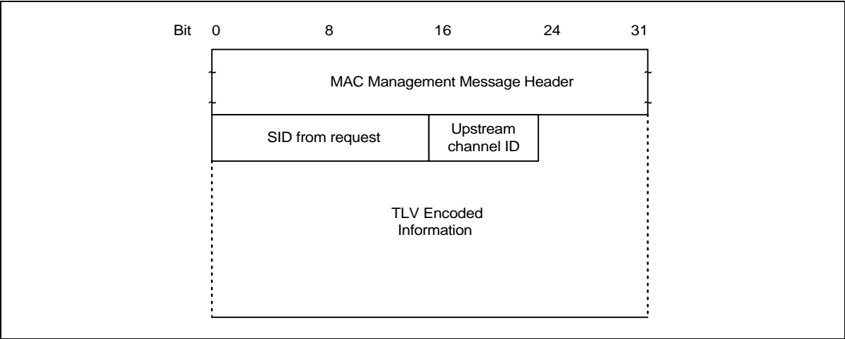
Figure 6-21. Ranging Response
