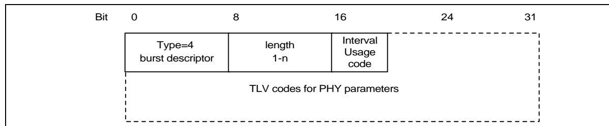
Figure 6-16. Top-Level Encoding for a Burst Descriptor
