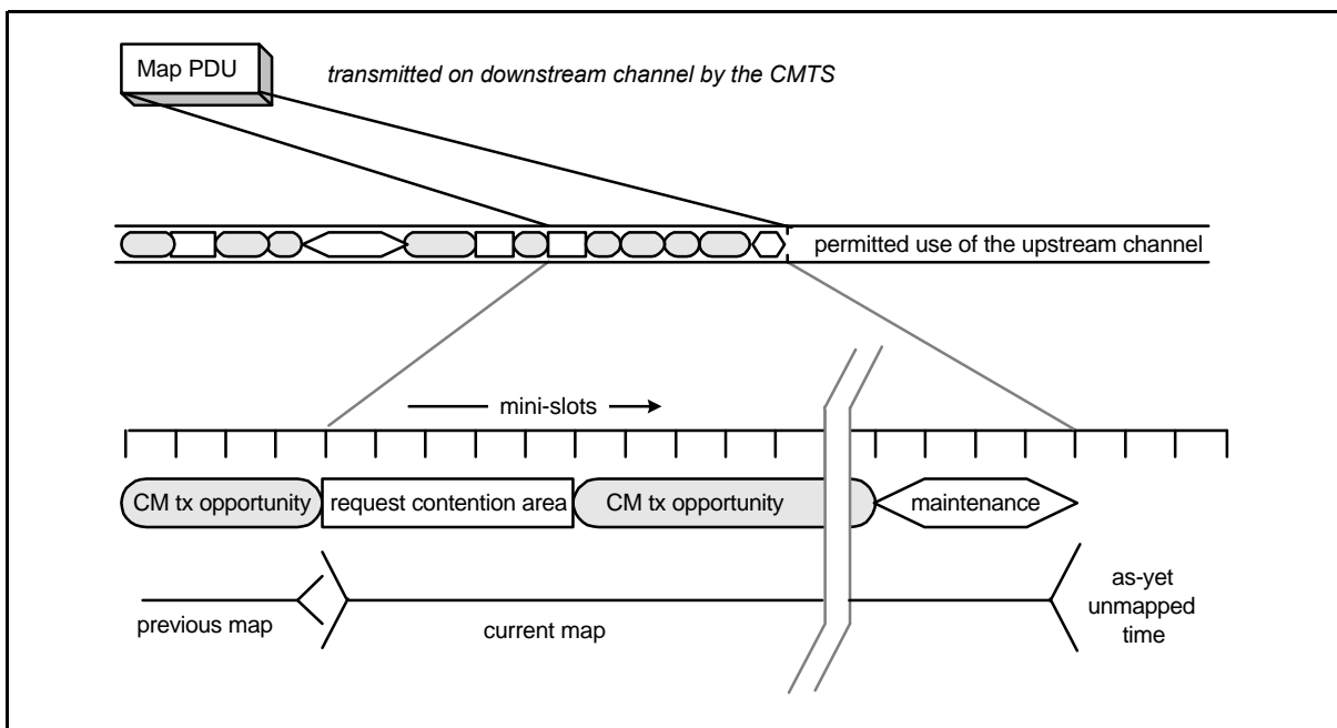
Figure 6-31. Allocation Map
