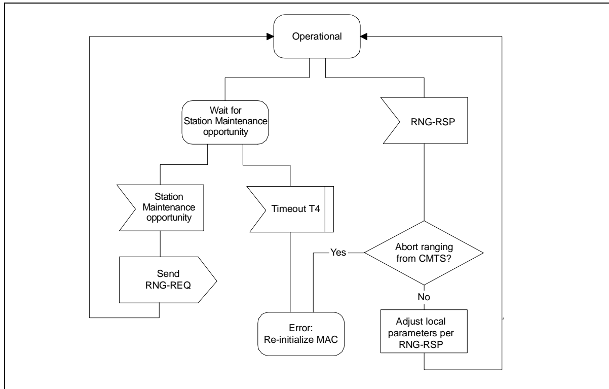
Figure 7-13. Periodic Ranging - CM View
