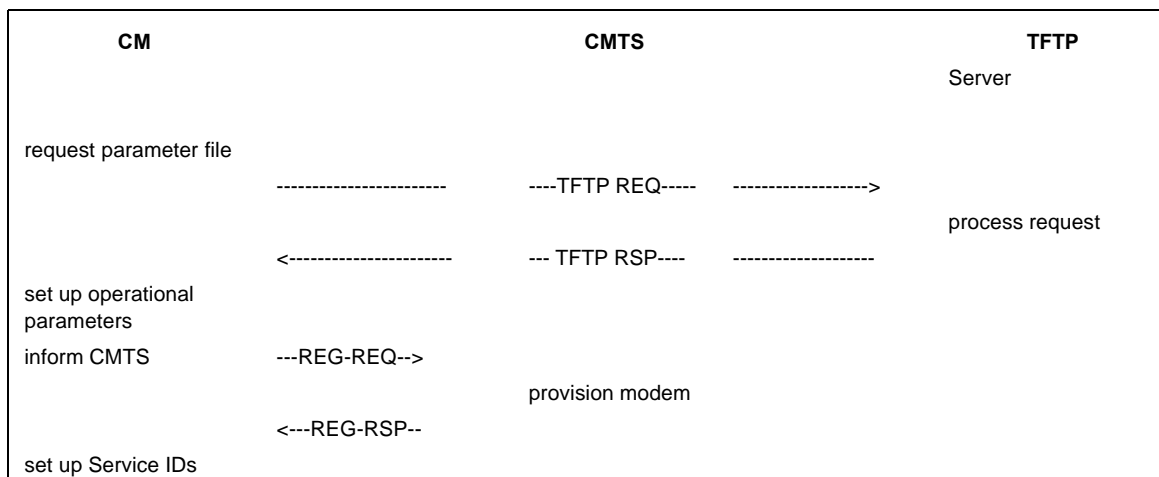
Figure 7-11. Transferring Operational Parameters and Registration
