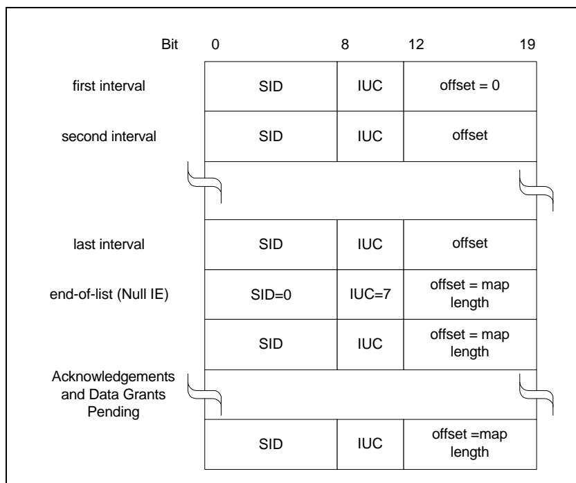
Figure 6-19. MAP Information Element Structure
