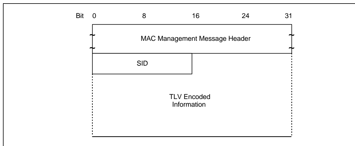
Figure 6-25. Registration Request
