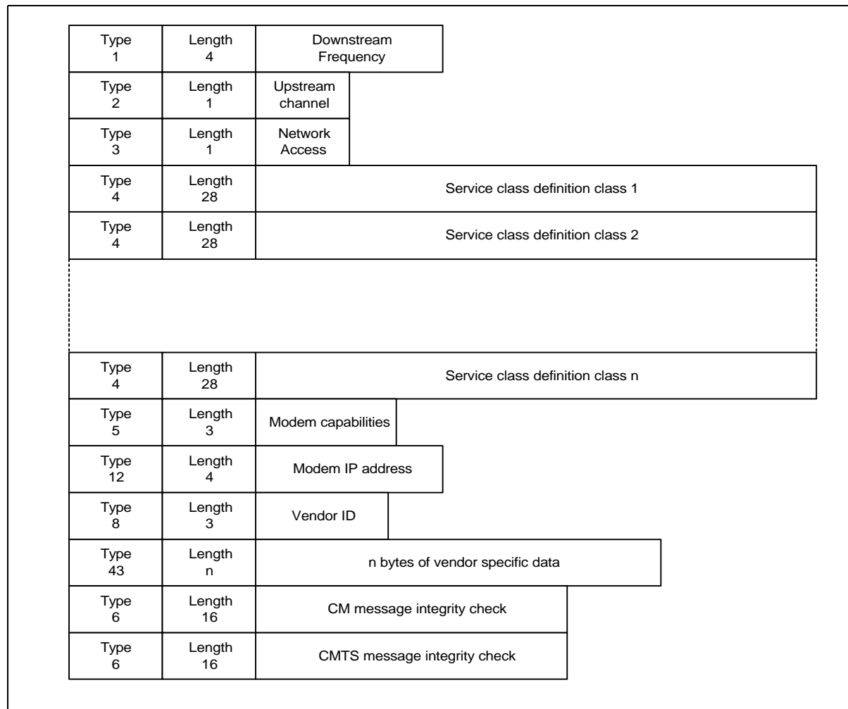
Figure 6-26. Example of Registration Request Type Value Encodings
