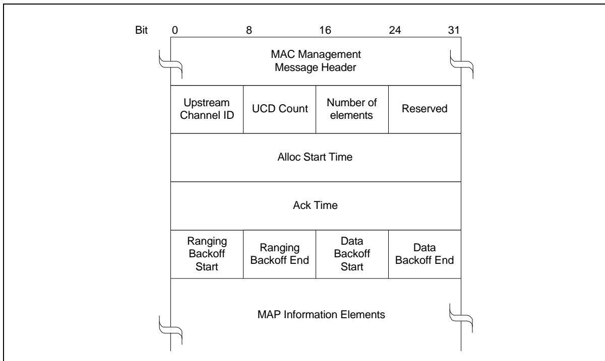
Figure 6-18. MAP Format
