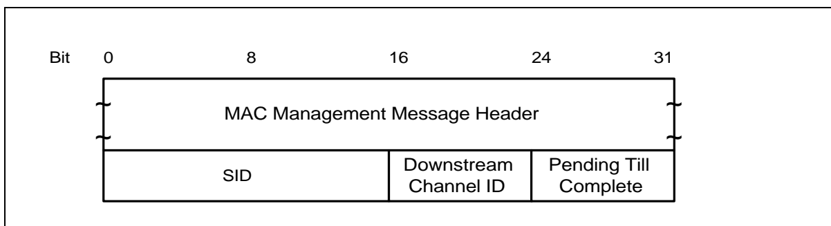
Figure 6-20. Packet PDU Following the Timing Header
