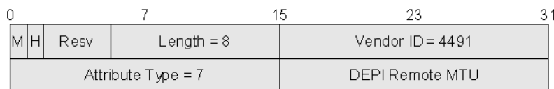
Figure 42 - DEPI Remote MTU Max Payload AVP
