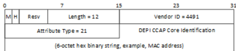
Figure 37 - DEPI CCAP Core Identification AVP
