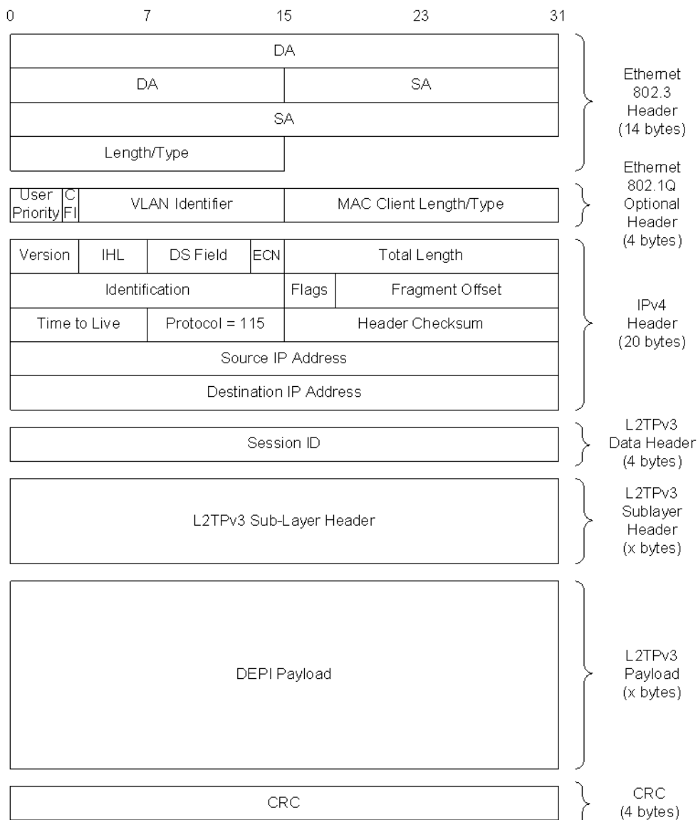
Figure 52 - L2TPv3 Data Packet Outer Encapsulation (without UDP)
