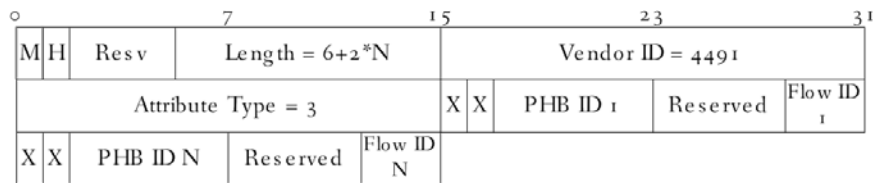
Figure 40 - DEPI Resource Allocation Reply AVP
