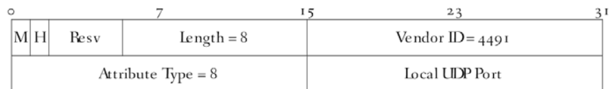
Figure 43 - DEPI Local UDP Port AVP
