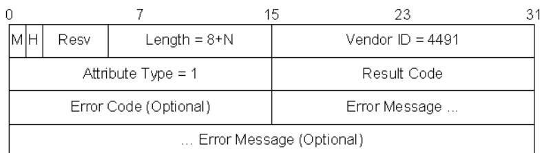
Figure 38 - DEPI Result and Error Code AVP
