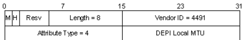
Figure 41 - DEPI Local MTU AVP
