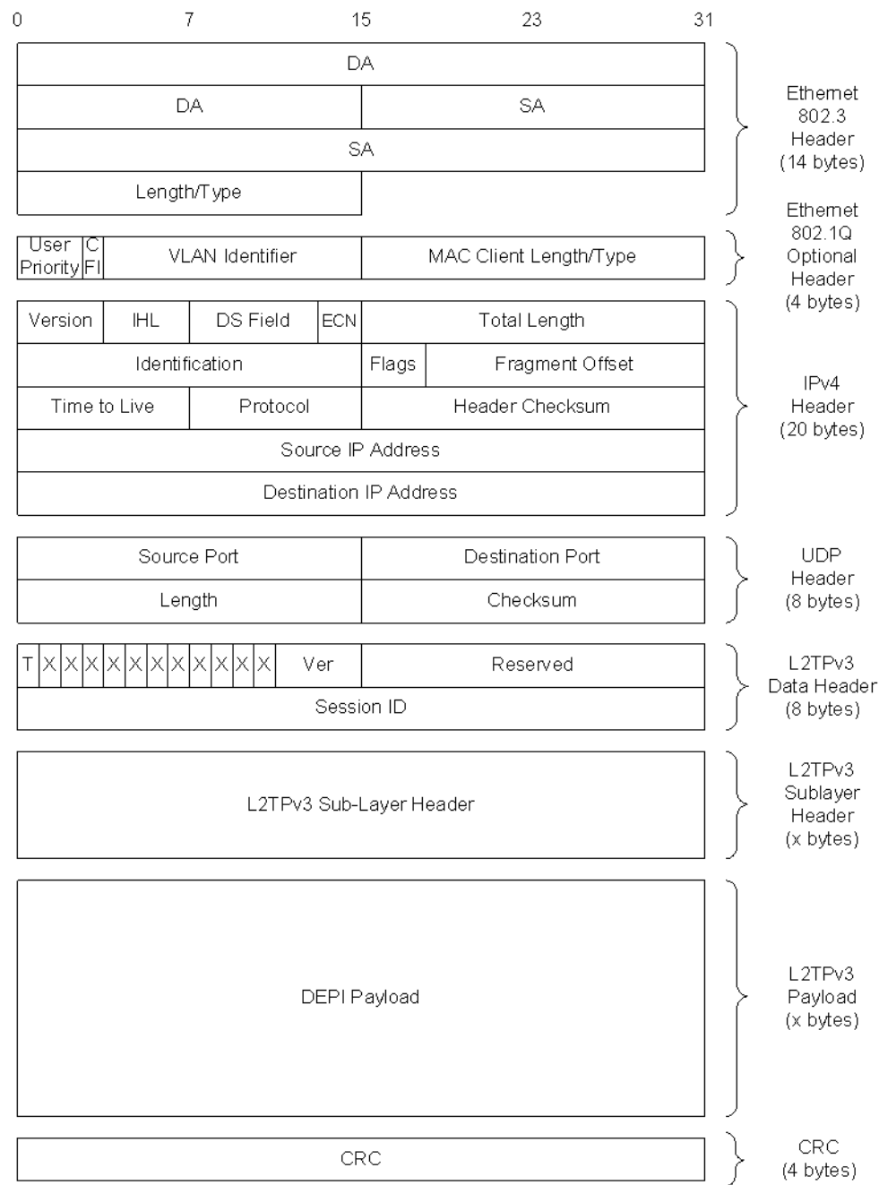
Figure 53 - L2TPv3 Data Packet Outer Encapsulation with UDP Header
