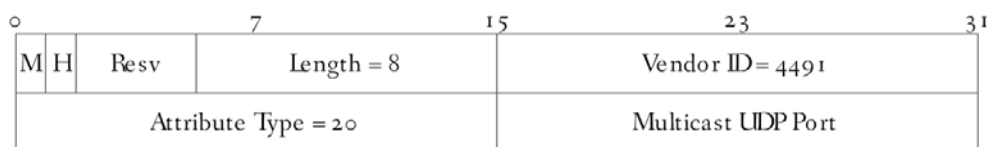
Figure 51 - DEPI Multicast UDP Port AVP
