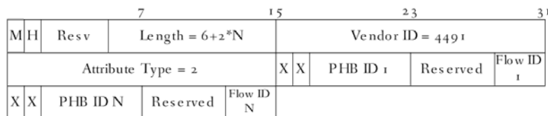
Figure 39 - DEPI Resource Allocation Request AVP
