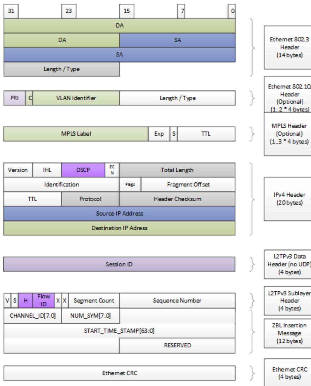
Figure 63 - L2TPv3 Packet Format for ZBL Insertion Message
