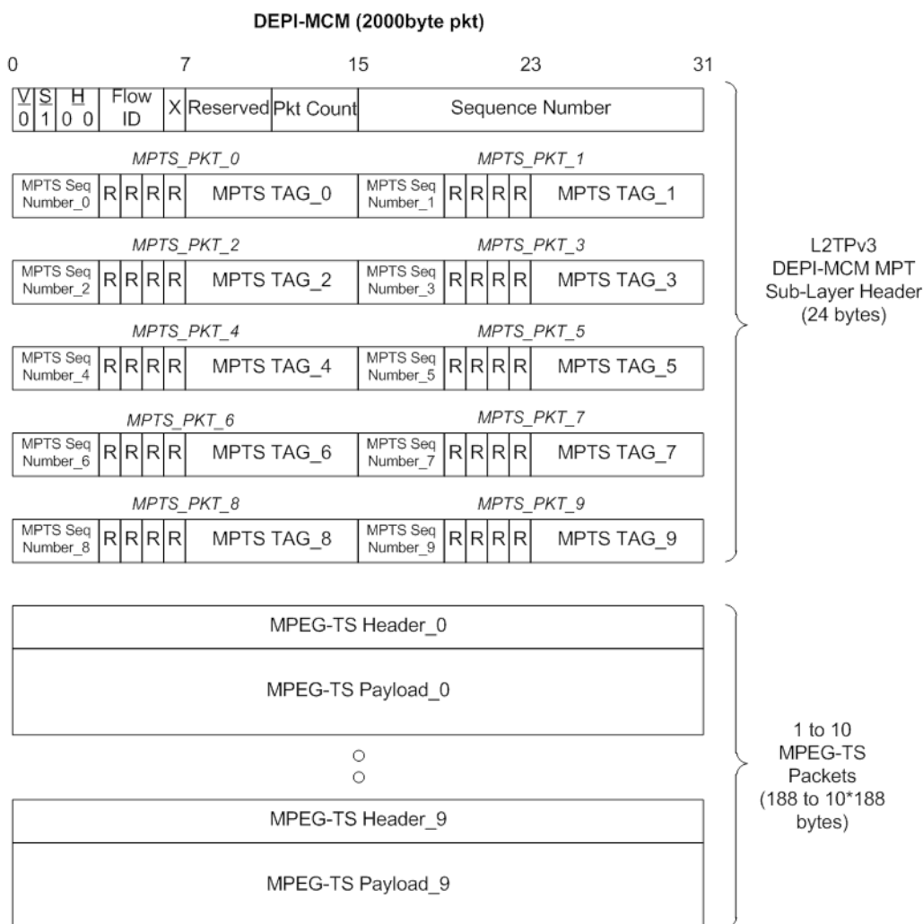
Figure 55 - MCM Sublayer Header and Payload
