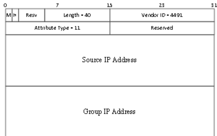
Figure 44 - DEPI Remote Multicast Join AVP
