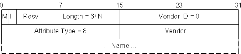
Figure 21 - Vendor Name AVP
