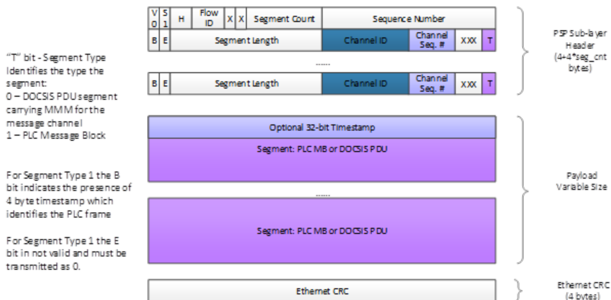
Figure 58 - Use of DEPI PSP Sublayer Header for PLC Subchannel
