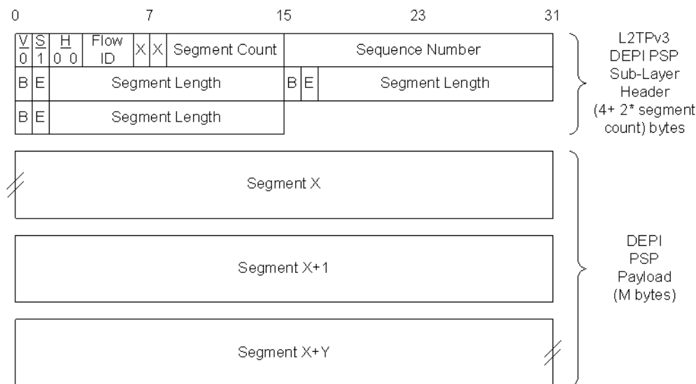
Figure 56 - DEPI Legacy PSP Sublayer Header and Payload
