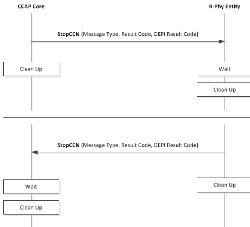
Figure 13 - R-PHY L2TP Control Connection Teardown
