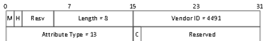
Figure 45 - DEPI Multicast Capability AVP
