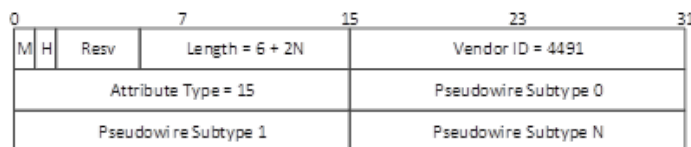
Figure 36 - DEPI Pseudowire Subtype Capabilities List AVP
