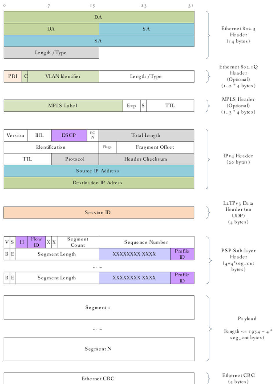
Figure 59 - Example of a Complete DEPI Packet Format (IPv4) with Extras
