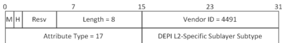
Figure 48 - DEPI L2-Specific Sublayer Subtype AVP
