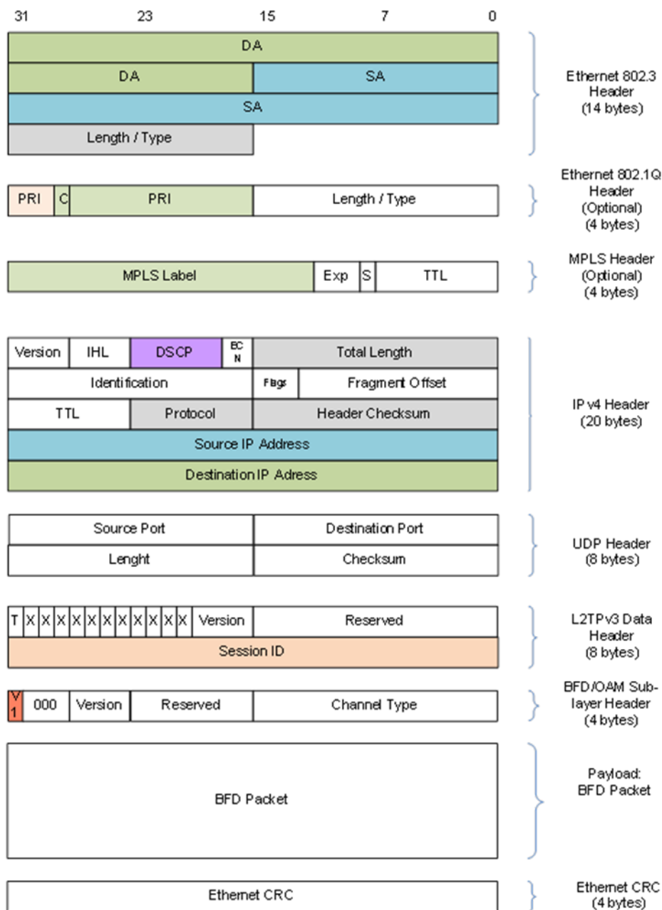
Figure 62 - BFD Sublayer (with UDP)
