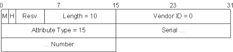
Figure 22 - Serial Number AVP
