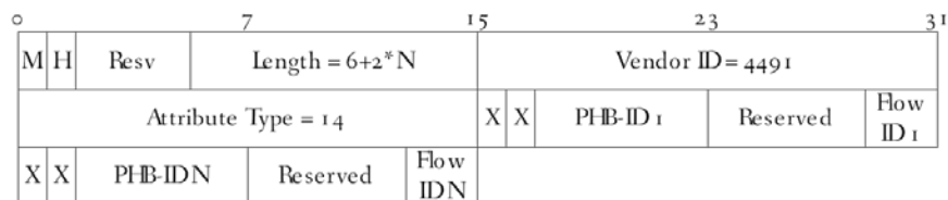
Figure 46 - Upstream Flow AVP
