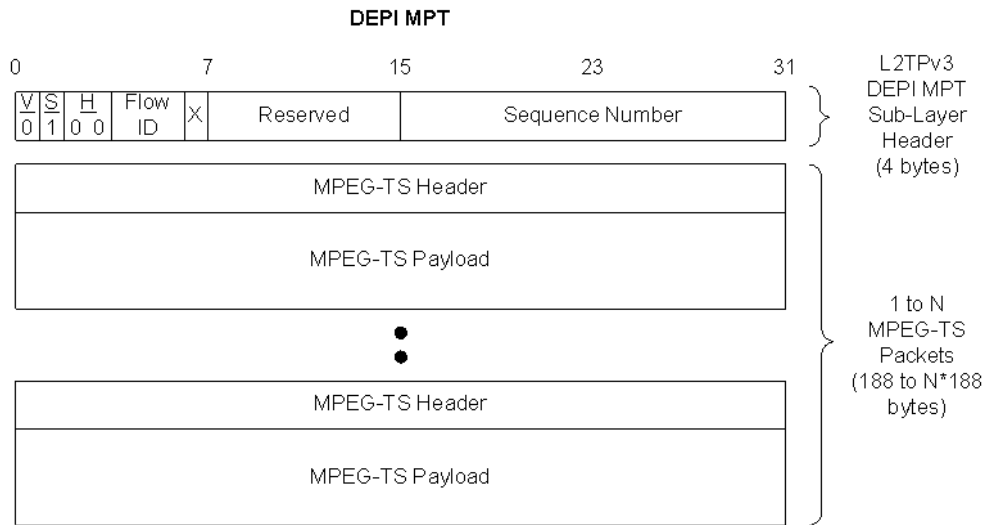
Figure 54 - DEPI MPT Sublayer Header and Payload
