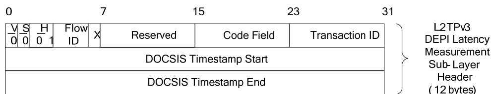
Figure 8–5 - DLM Sub-Layer Header 56
