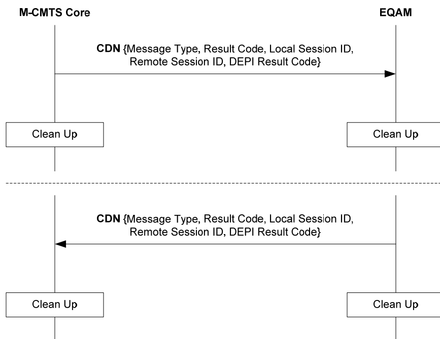
Figure 7–10 - DEPI Session Teardown
