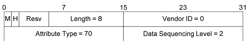
Figure 7-25 - Data Sequencing AVP
