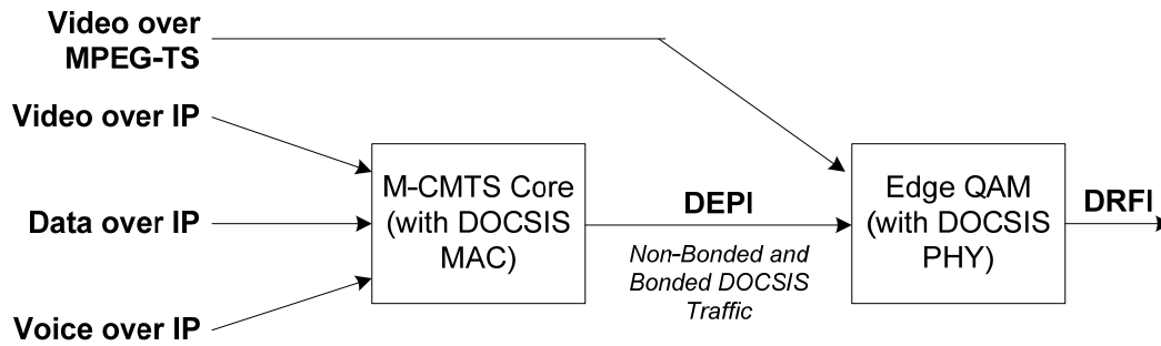
Figure 5-4 - Multi-Service Mode
