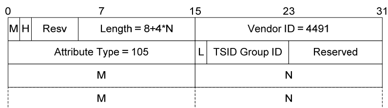
Figure 7–40 - Symbol Rate AVP
