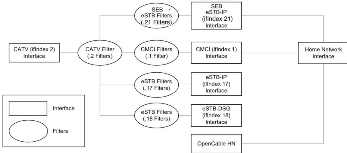
Figure 5-21 - eSTB Interface 28
