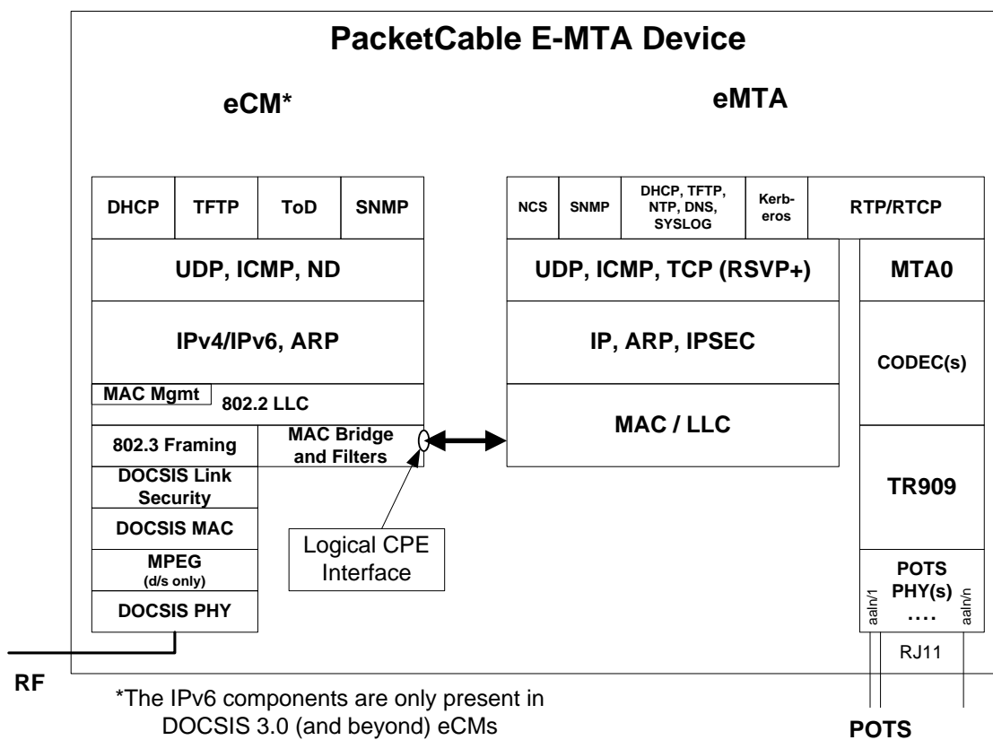
Figure 5–5 - eCM - eMTA Protocol Stacks 9
