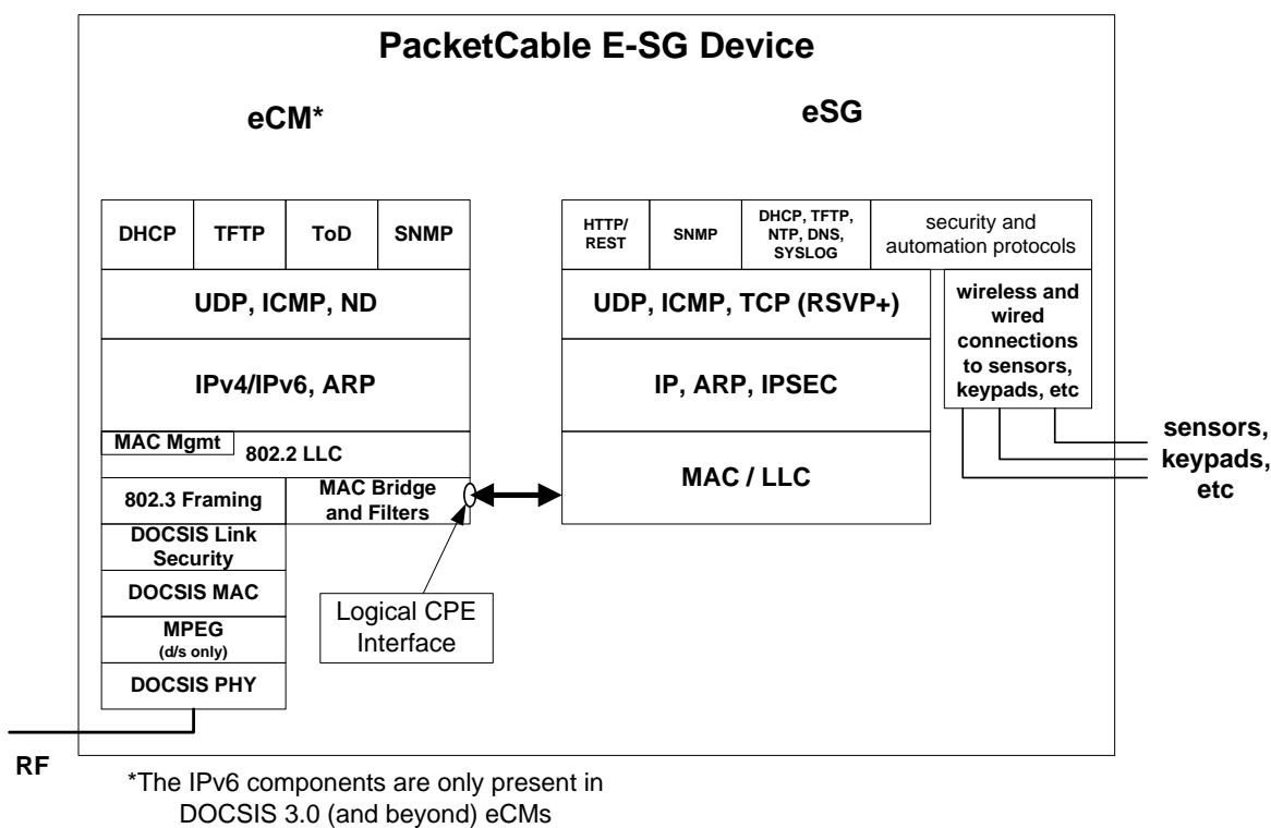
Figure 5–20 - eCM – eSG Protocol Stacks
