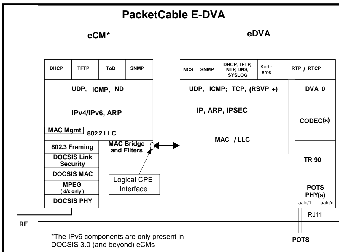
Figure 5–18 - eCM - eDVA Protocol Stacks 20
