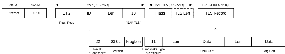
Figure 18 - EAP-TLS Frame Format 2 6
