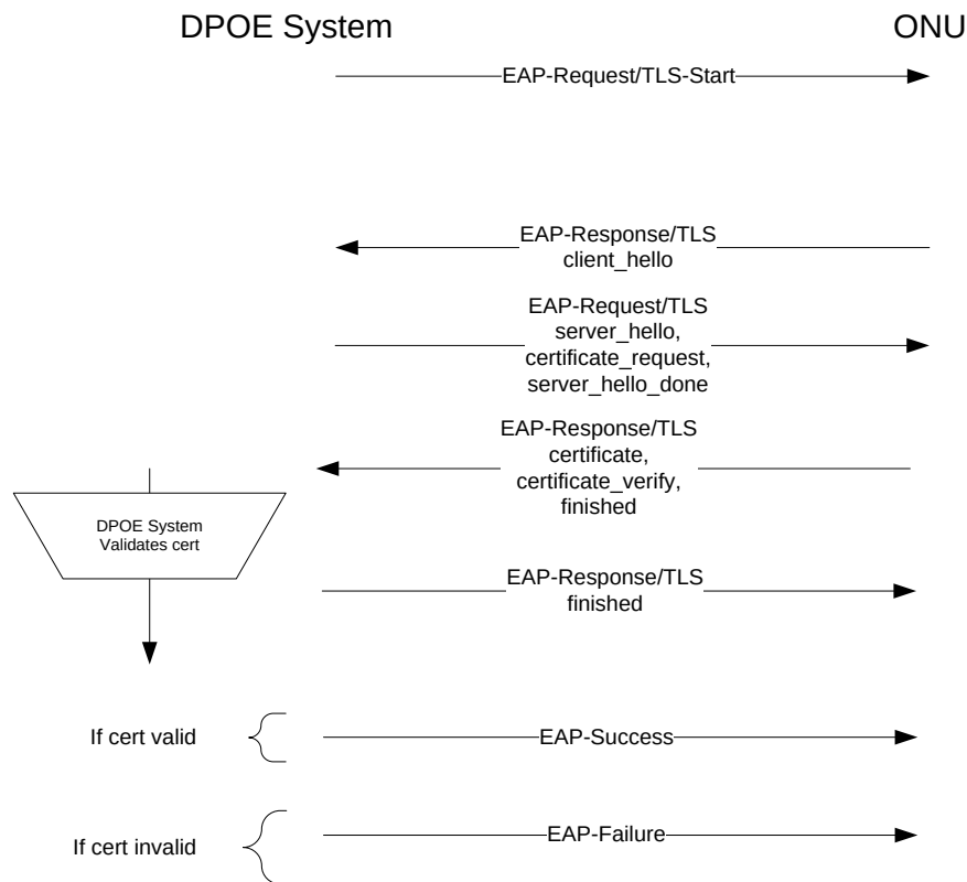
Figure 16 - EAP-TLS Message Sequence
