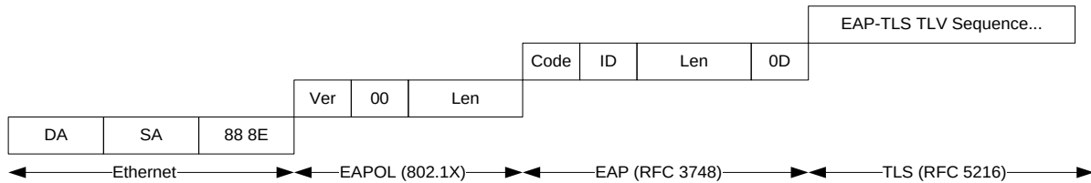
Figure 17 - EAP-TLS Frame Format
