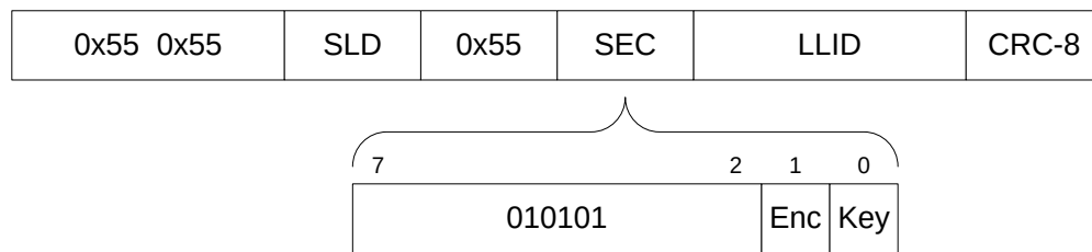
Figure 5 - Security Octet (1Down)
