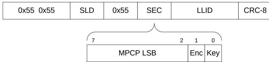
Figure 6 - Security Octet (10G Zero Overhead)
