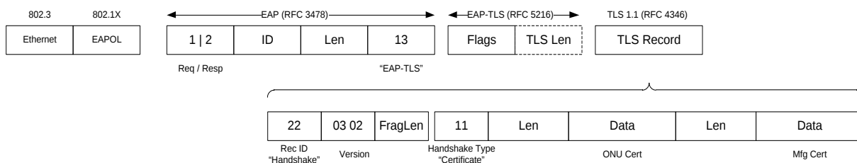
Figure 18 - EAP-TLS Frame Format 2 11
