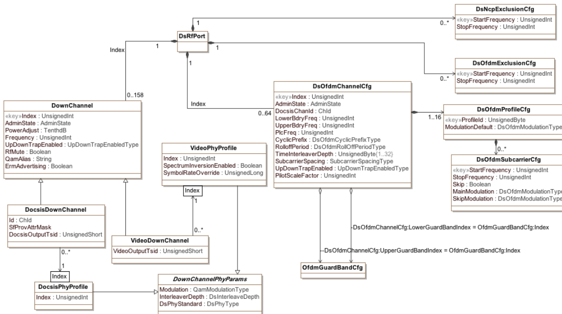
Figure 6 - Downstream DOCSIS Configuration Objects
