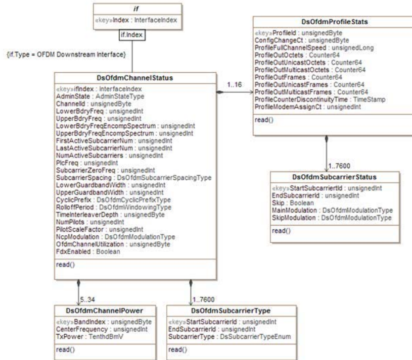
Figure 5 - DsOfdmChannelStatus Object
