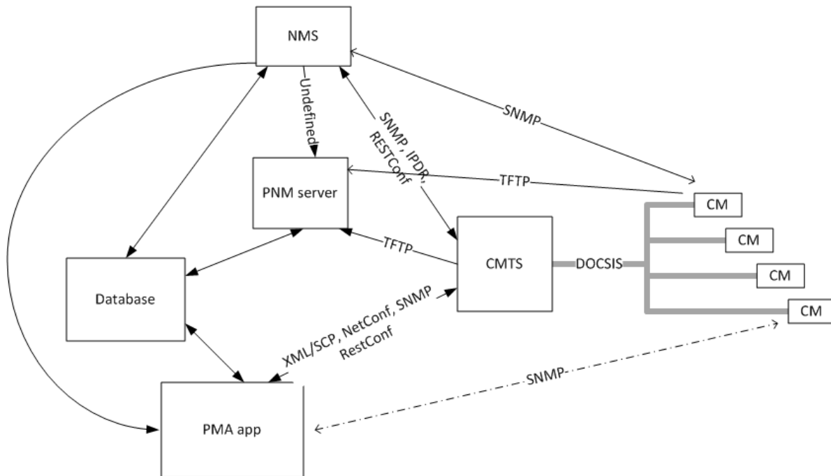
Figure 19 - PMA Data Backend and Protocols
