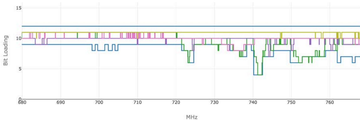
Figure 20 – DS Profile definitions (sample OFDM profiles for a 96 MHz downstream)
