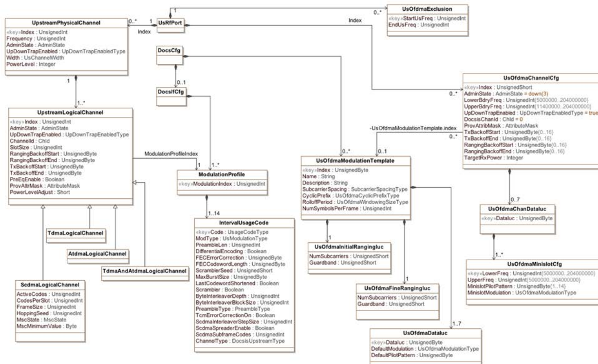
Figure 11 - DOCSIS Upstream Interface Configuration Model from [CCAP-OSSIV3.1]
