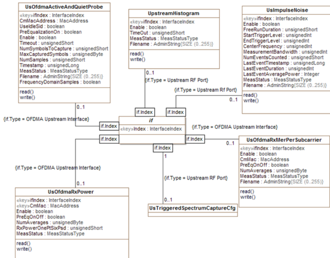
Figure 10 - UsOfdmaRxMerPerSubcarrier UML Model [CCAP-OSSIV3.1]
