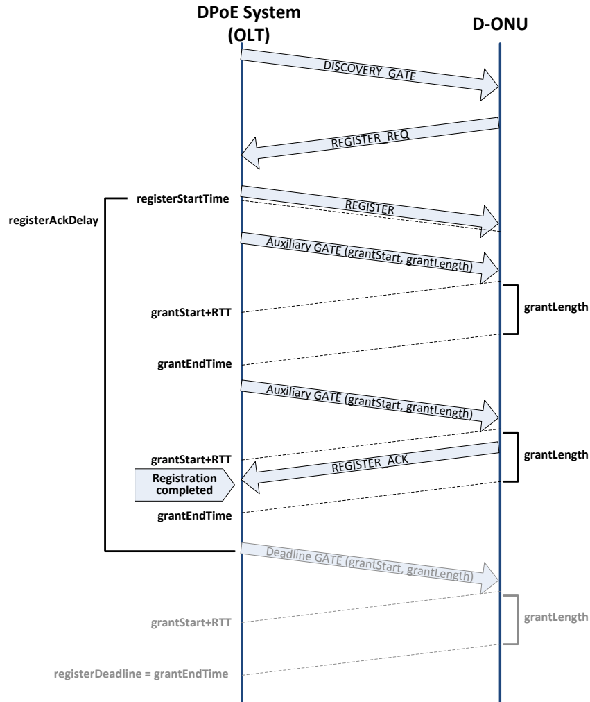
Figure 25 - DPoE MPCP Discovery Process Using Multiple Auxiliary GATE Messages, REGISTER_ACK Message Arrived in Grant from Auxiliary GATE Message.
