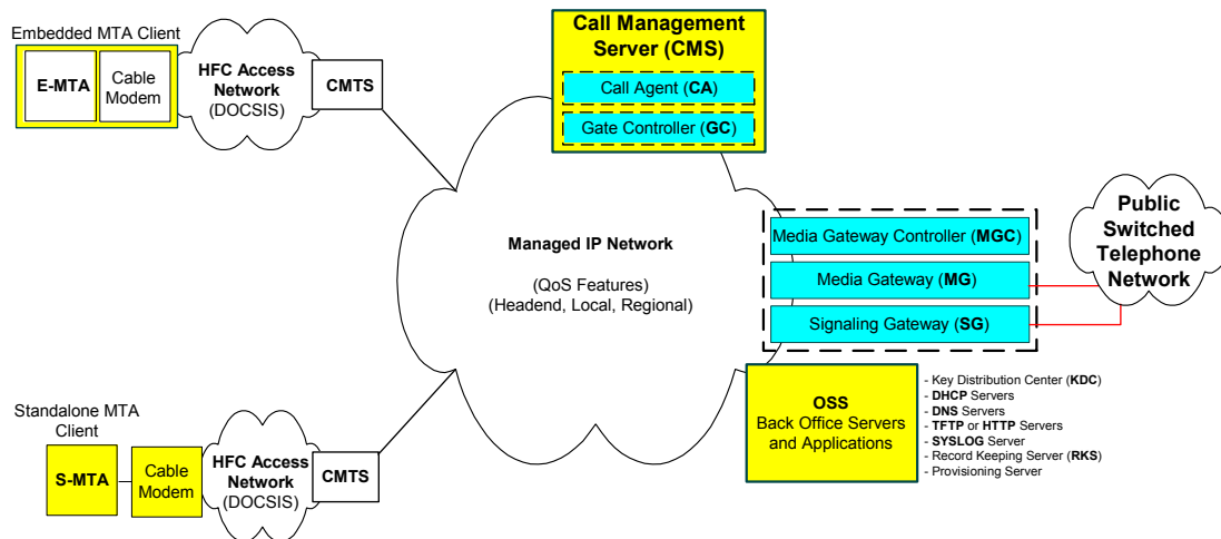
Figure 2. PacketCable 1.0 Network Component Reference Model
