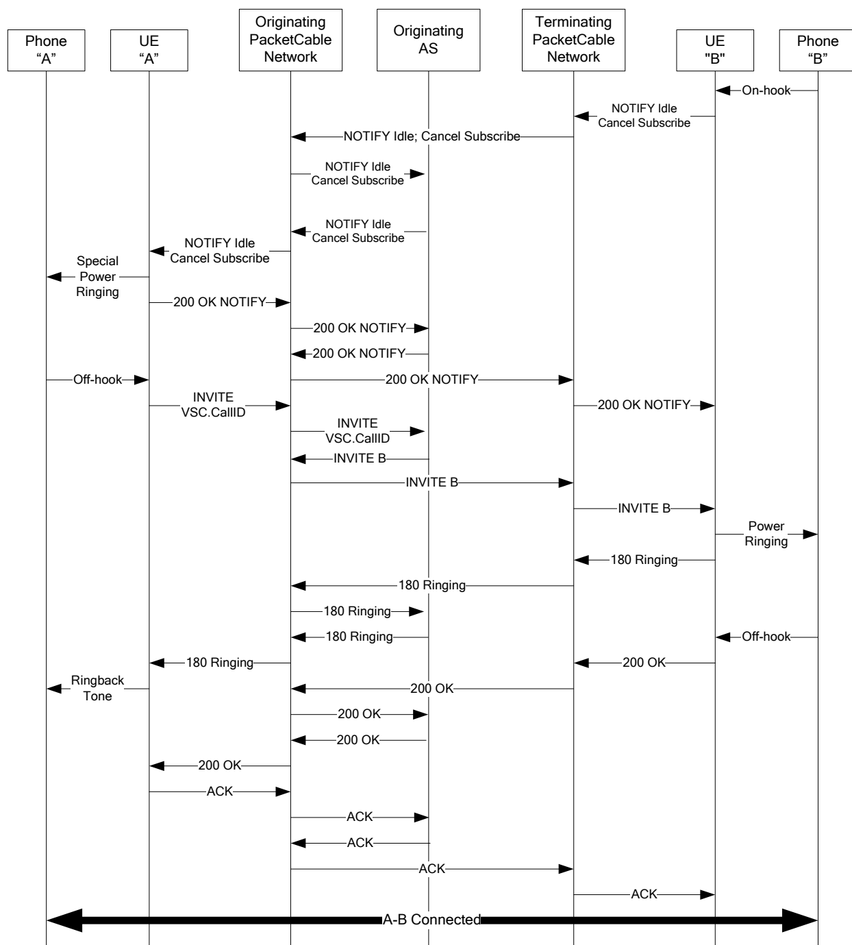
Figure 68 - AR; Anonymous target becomes idle
