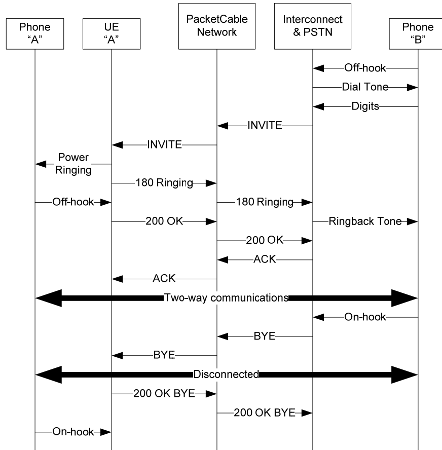
Figure 5 - Basic Call - PSTN Off-Net to On-Net
