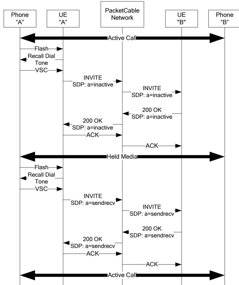
Figure 42 - Network Hold; Hold and Retrieve
