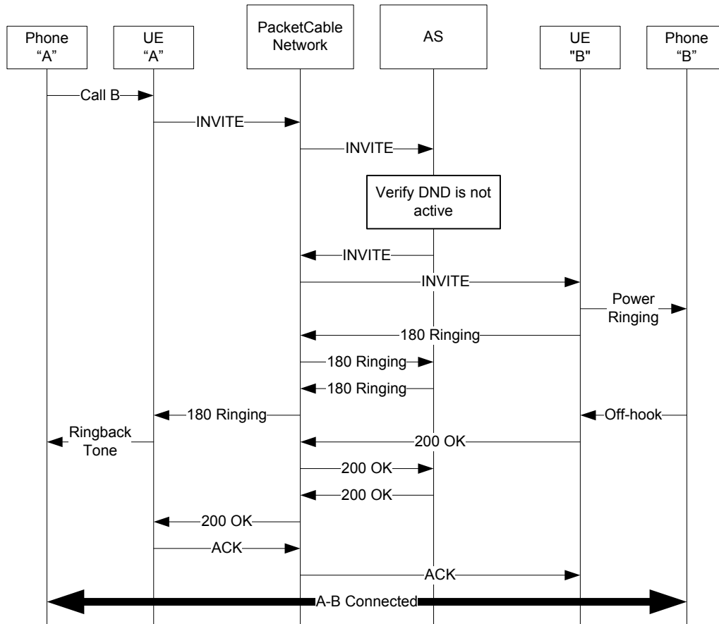
Figure 52 - Do Not Disturb (DND); Deactivated
