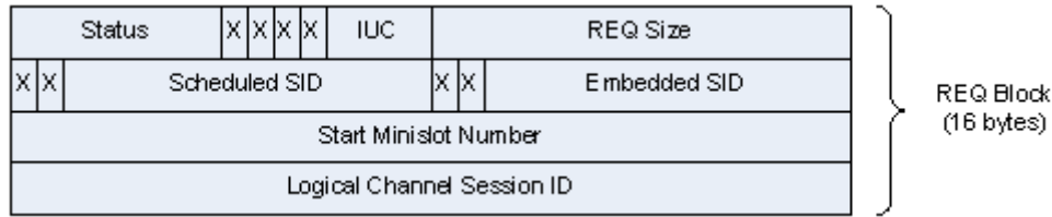
Figure 16 - UEPI REQ Block Format for an SC-QAM Channel
