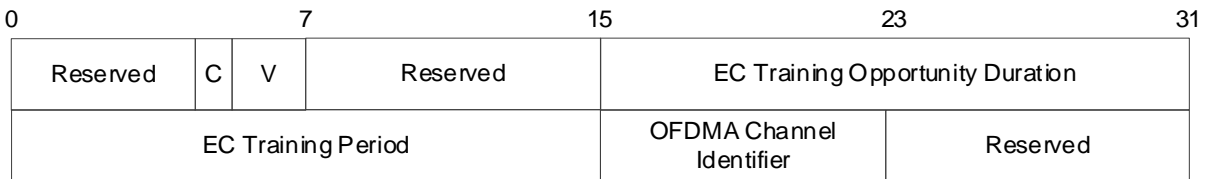
Figure 25 - UEPI EC-REQ Block Format
