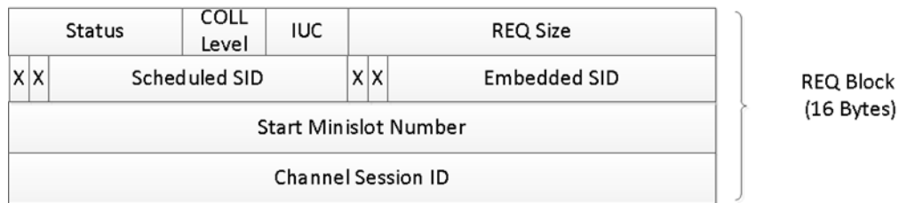
Figure 15 - UEPI REQ Block Format for an OFDMA Channel
