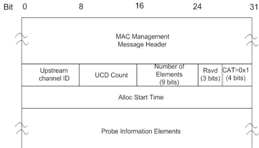
Figure 19 - Segment Format for the UEPI MAP Pseudowire for Version 5 Probe Frames
