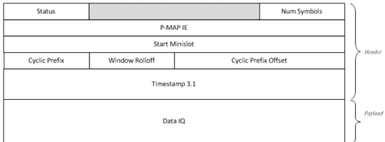
Figure 23 - Upstream Capture for Active and Quiet Probes Transmission Unit
