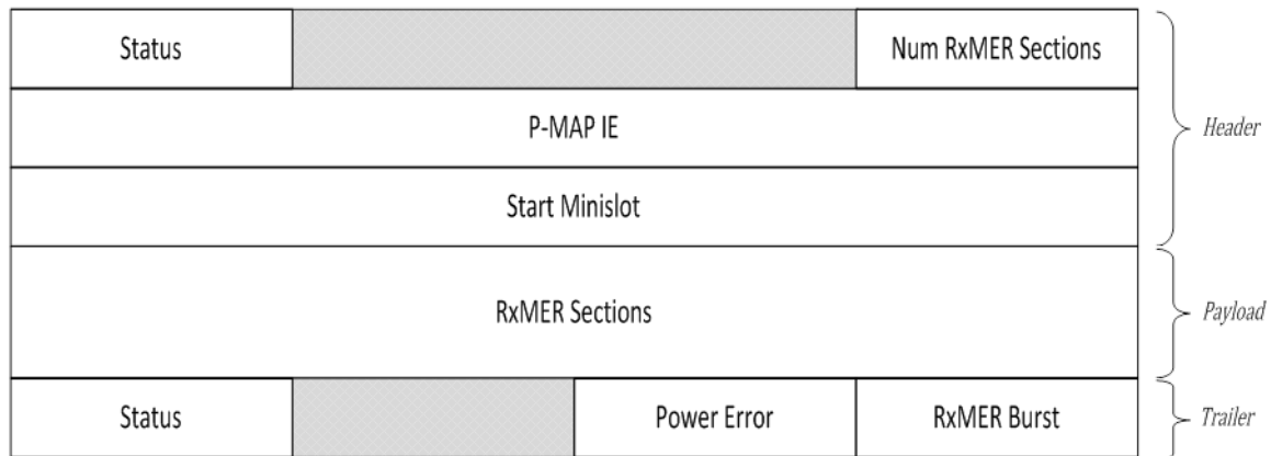
Figure 24 - RxMER Pseudowire Transmission Unit Format
