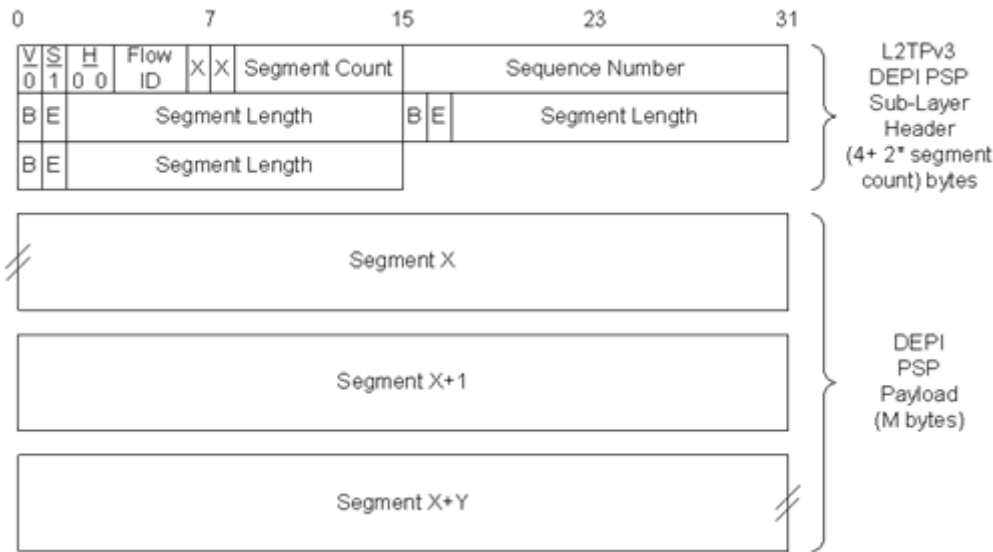
Figure 6 - Legacy PSP Sublayer Header and Payload
