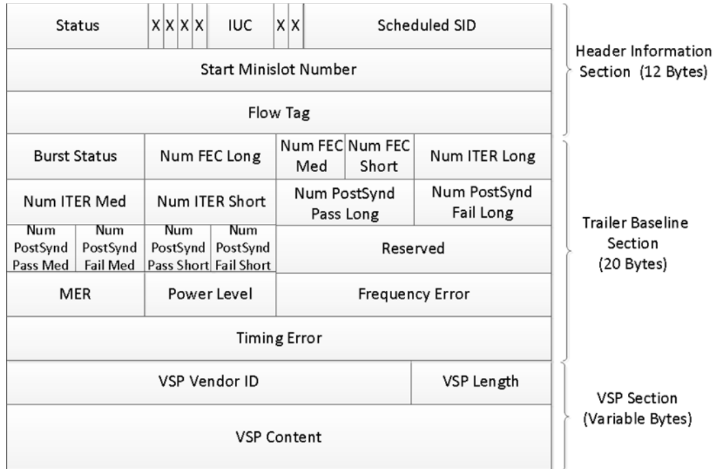
Figure 12 - UEPI Trailer Segment Format
