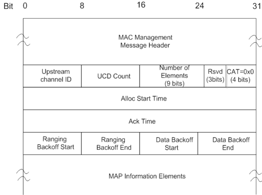
Figure 18 - Segment Format for the UEPI MAP Pseudowire (Version 5) Non-probe MAP Frames for an OFDMA Channel
