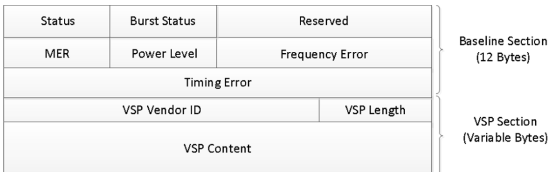
Figure 14 - UEPI RNG-REQ Trailer Segment Format
