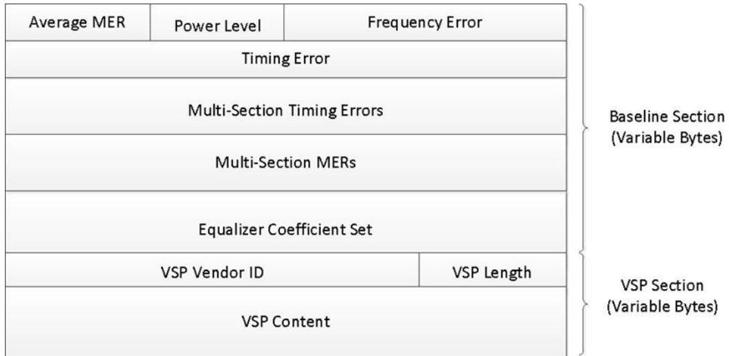
Figure 22 - UEPI Probe Payload Format
