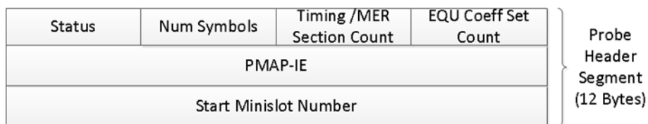
Figure 21 - UEPI Probe Pseudowire Header Segment
