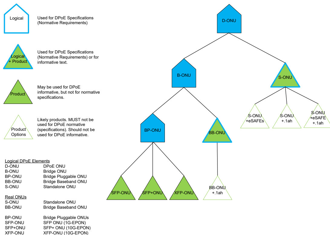
Figure 1 - D-ONU Types
