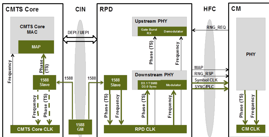
Figure 6 - R-DTI Node_Slave Architecture - RPD Slave / Core Slave / Common Master
