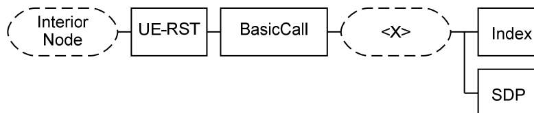
Figure 8 - Node BasicCall of UE-RST OMA Management Object
