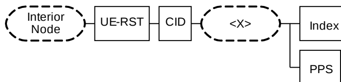
Figure 17 - Node CID of UE-RST OMA Management Object
