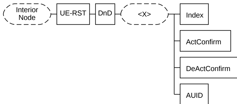
Figure 26 - Node DnD of UE-RST OMA Management Object
