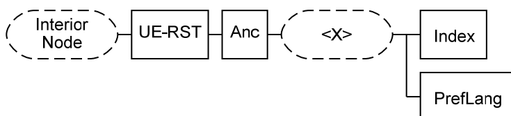
Figure 10 - Node Anc of UE-RST OMA Management Object
