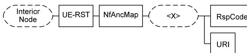
Figure 12 - Node NfAncMap of UE-RST OMA Management Object
