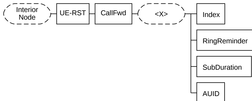
Figure 22 - Node CallFwd of UE-RST OMA Management Object
