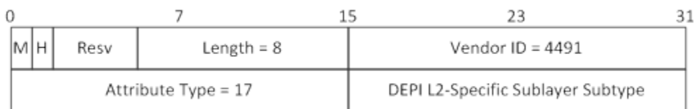
Figure 46 - DEPI L2-Specific Sublayer Subtype AVP
