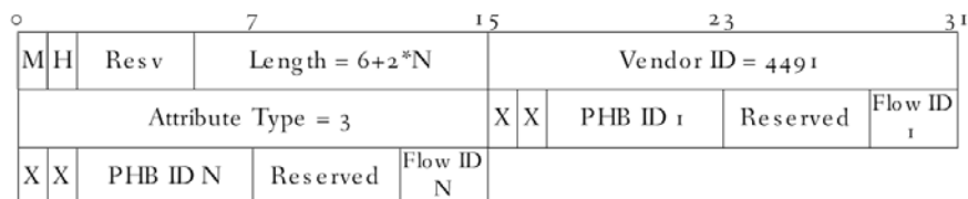
Figure 38 - DEPI Resource Allocation Reply AVP
