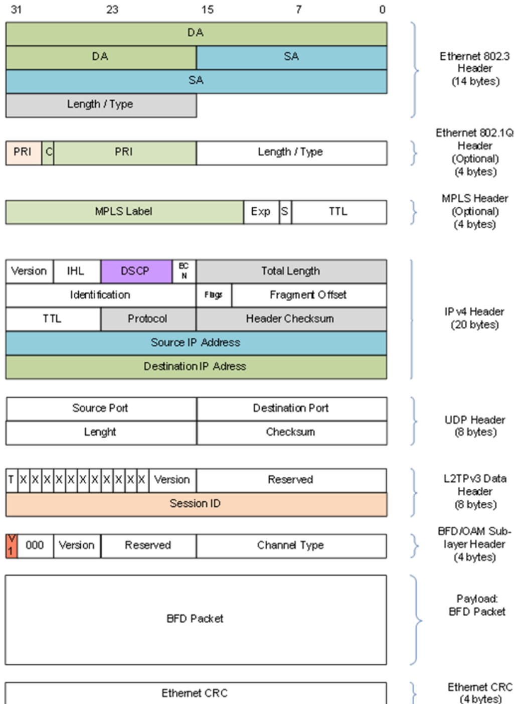
Figure 60 - BFD Sublayer (with UDP)
