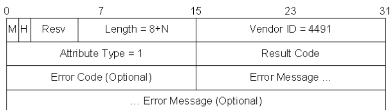
Figure 36 - DEPI Result and Error Code AVP
