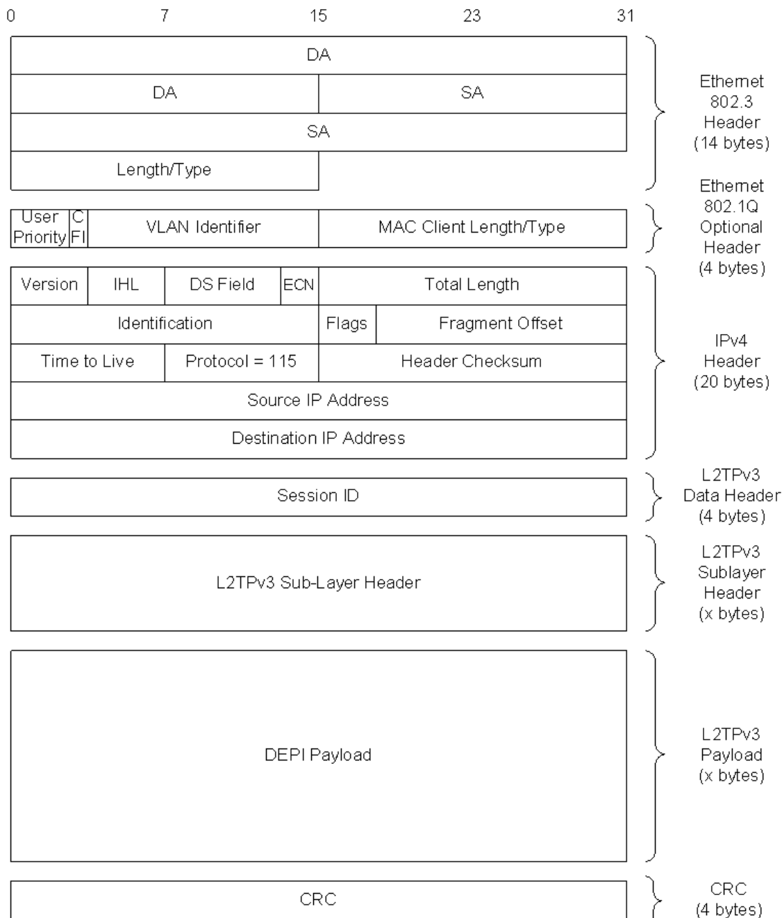
Figure 50 - L2TPv3 Data Packet Outer Encapsulation (without UDP)
