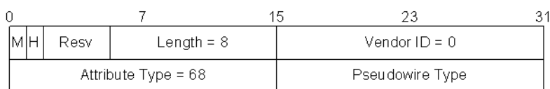
Figure 31 - Pseudowire Type AVP
