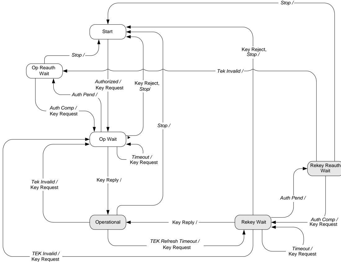
Figure 7-3 - TEK State Machine Flow Diagram
