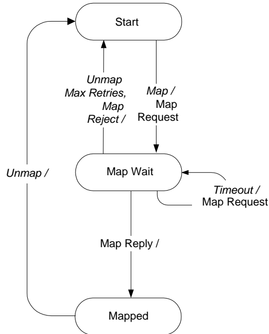
Figure C-1 - SA Mapping State Machine Flow Diagram
