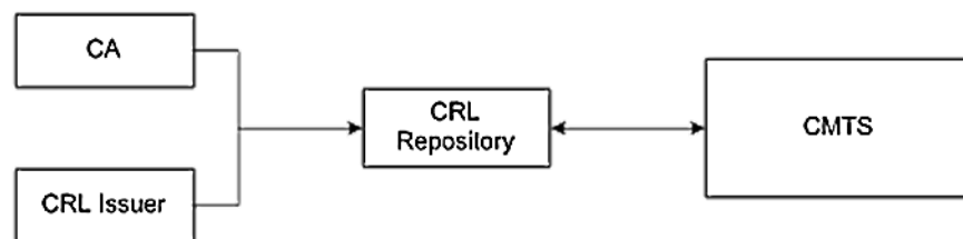
Figure 13 - CRL Framework
