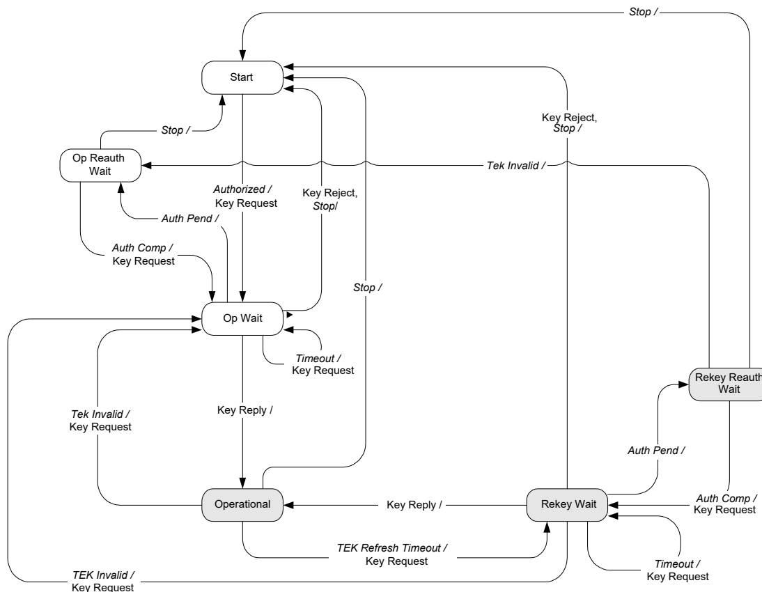
Figure 9 - TEK State Machine Flow Diagram
