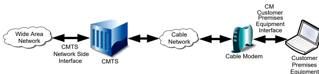
Figure 2 - Transparent IP Traffic through the Data-Over-Cable System
