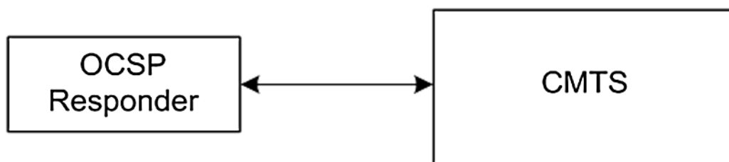
Figure 14 - OCSP Framework
