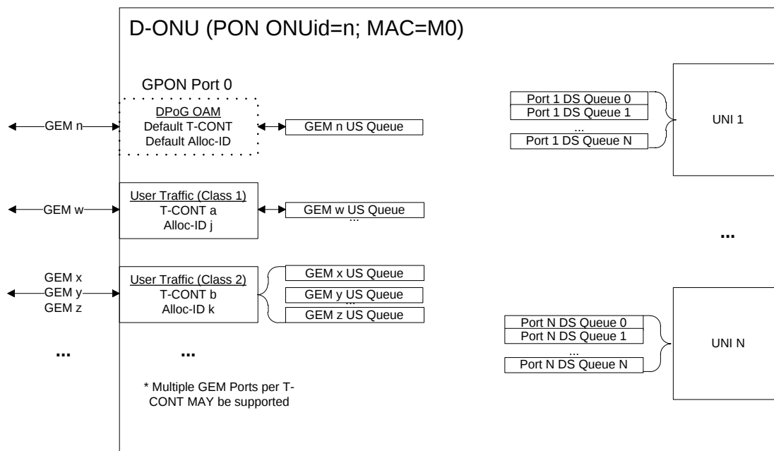
Figure 3 - D-ONU Model
