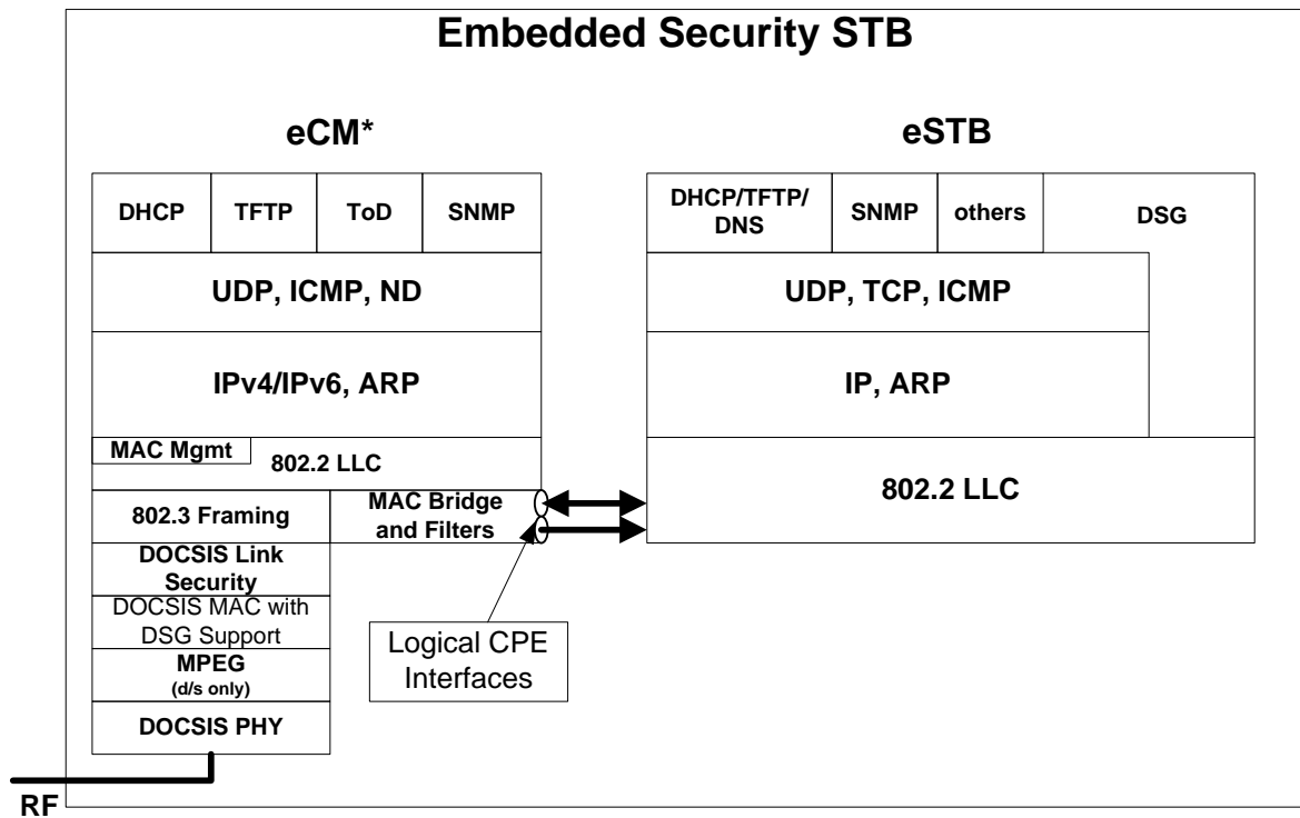
Figure 5–9 - eCM - eSTB Protocol Stacks - Embedded Security STB 24
