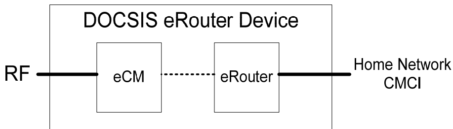
Figure 5–15 - DOCSIS eRouter eDOCSIS Device Reference Model 28
