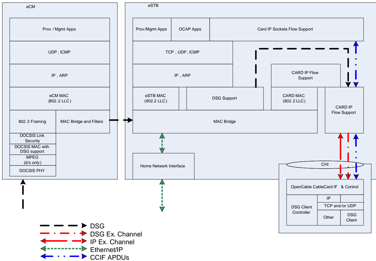
Figure 5-11 - Set-top Extender Bridge Client - Protocol Stack
