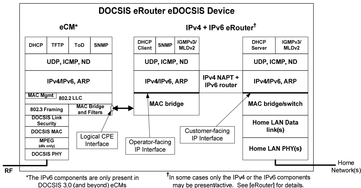
Figure 5–16 - eCM - eRouter eDOCSIS Protocol Stacks 29
