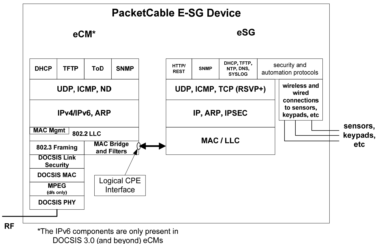
Figure 5–20 - eCM – eSG Protocol Stacks
