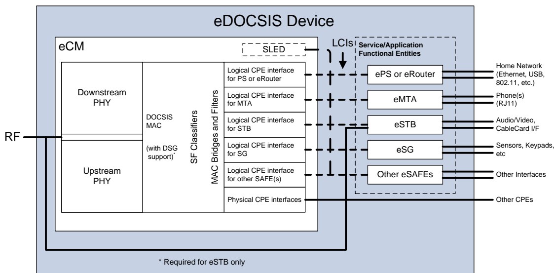
Figure 5–1 - eDOCSIS Reference Model 18
