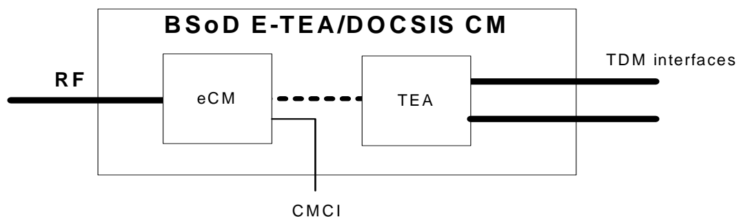
Figure 5-13 - BSoD eTEA (with DOCSIS CM) eDOCSIS Reference Model 26
