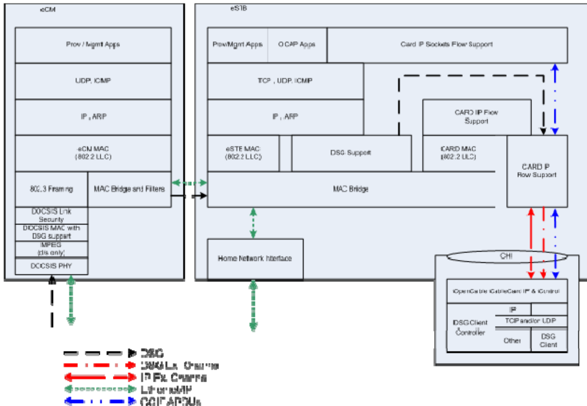
Figure 5-12 - Set-top Extender Bridge Server - Protocol Stack
