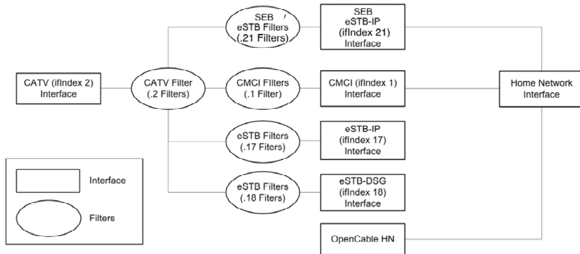
Figure 5-21 - eSTB Interface 42
