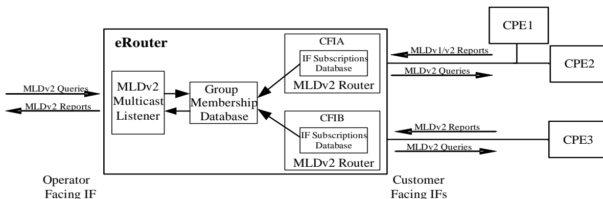
Figure 10-3 - IPv6 Multicast Forwarding Example 54
