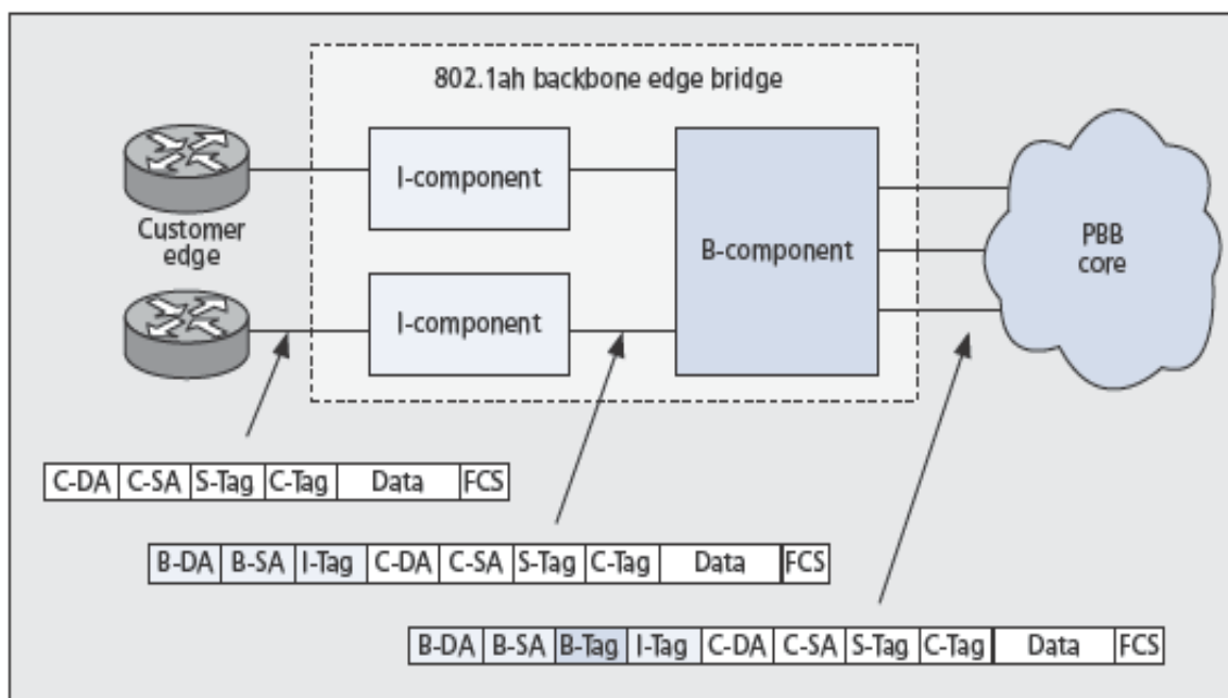
Figure 13 - [802.1ah] Provider Backbone Bridge Model [IEEE-Comm-PBB-MPLS]
