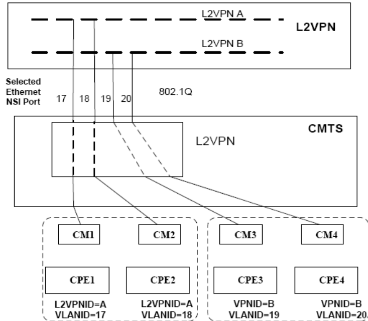
Figure 8 - Point-to-Point Forwarding [L2VPN]
