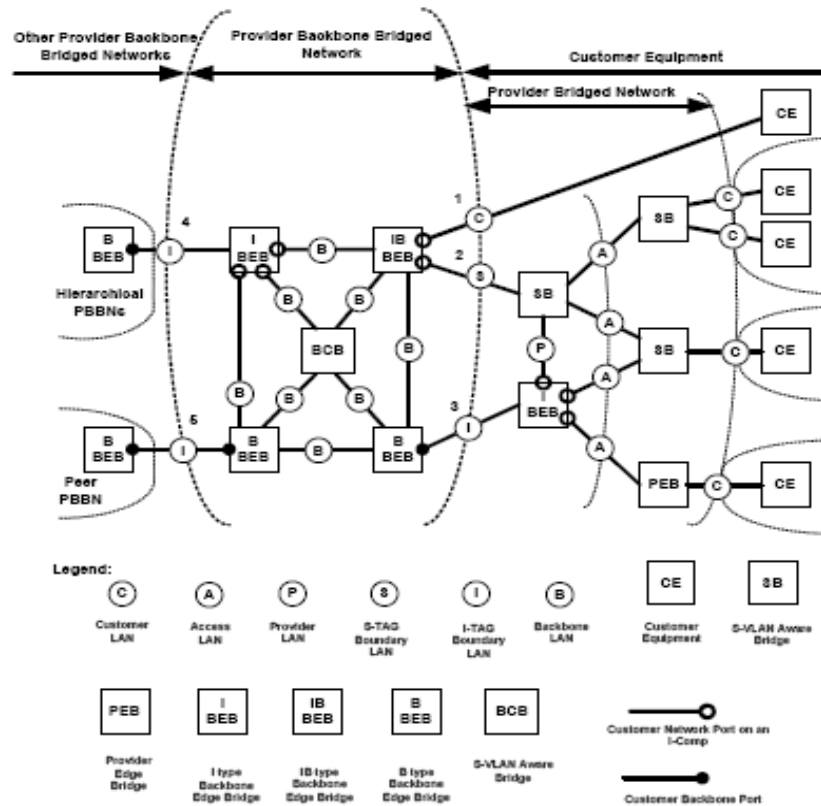
Figure 4 - [802.1ah] Networking Scenarios
