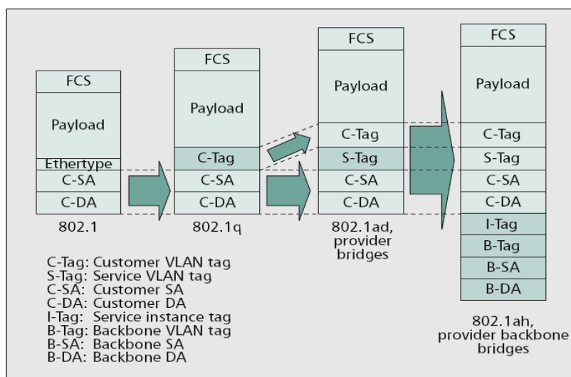
Figure 12 - [802.1ad] Provider Bridge Frame Formats [IEEE-Comm-CE-Dev]
