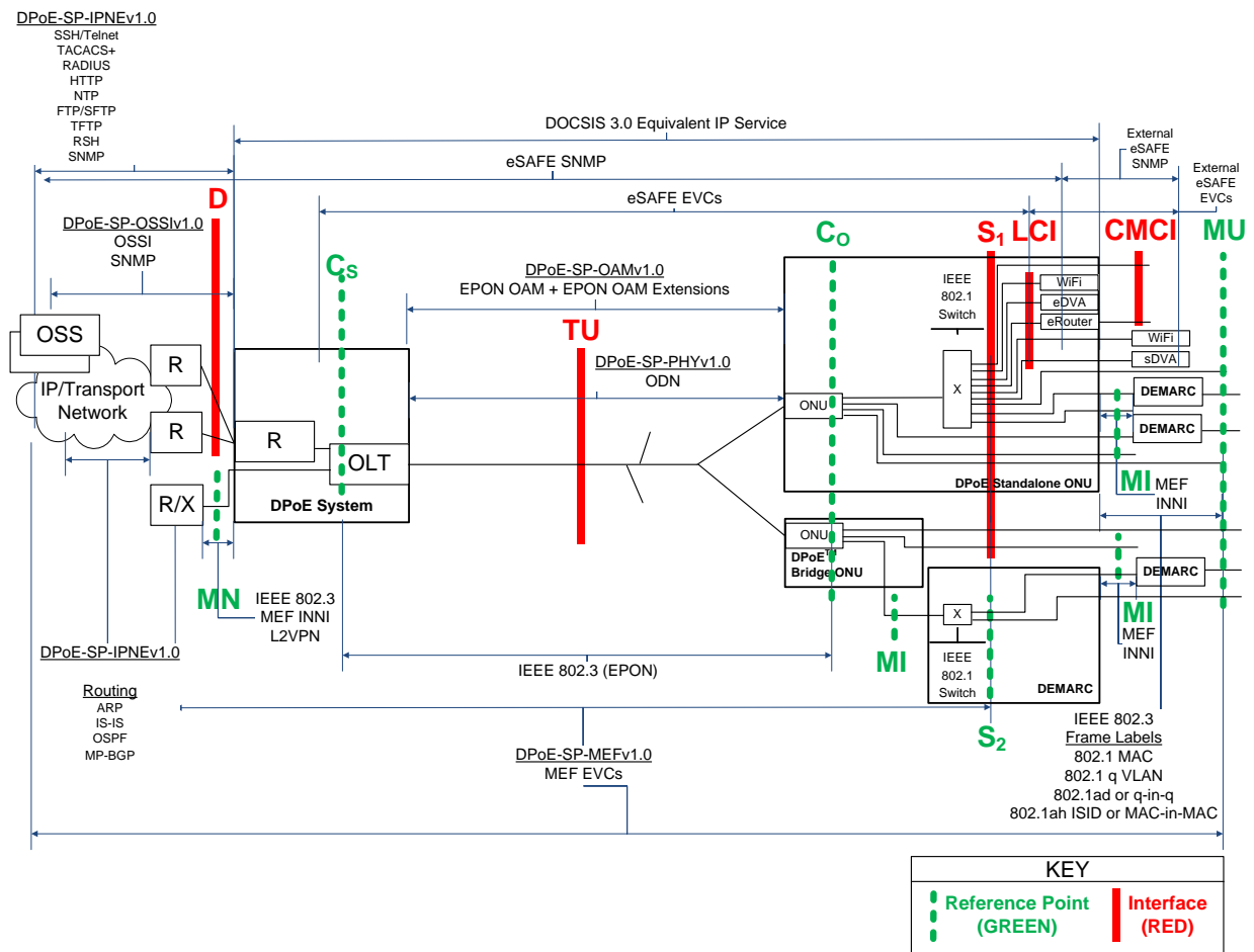
Figure 2 - DPoE Interfaces and Reference Points
