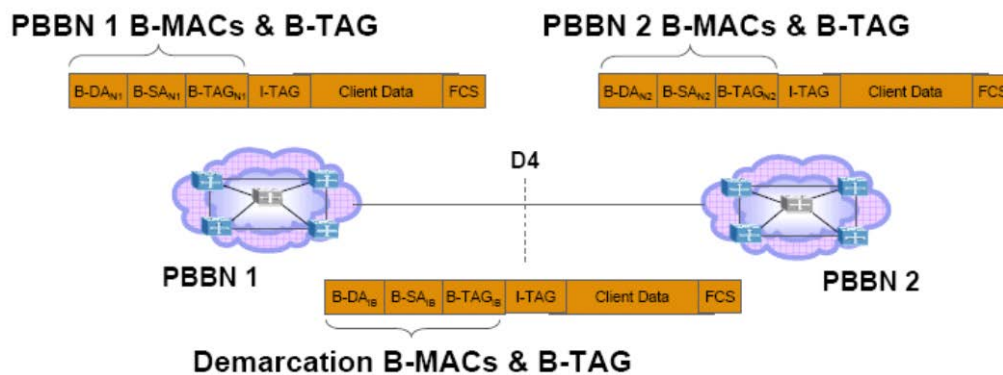
Figure 16 - Peer PBBNs [IEEE-802.1-PBB-Models]
