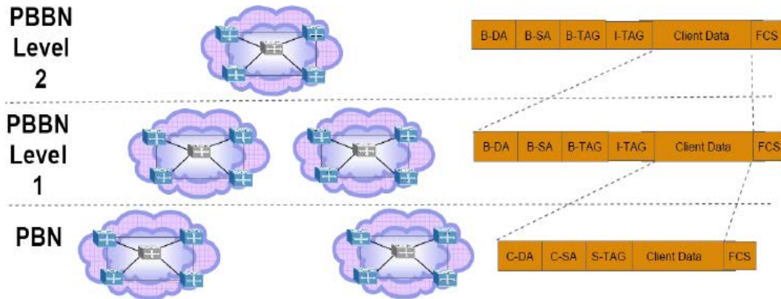
Figure 15 - Hierarchical PBB Model [IEEE-802.1-PBB-Models]
