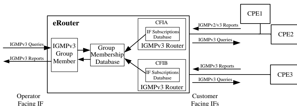
Figure 9-3 - IPv4 Multicast Forwarding Example 45
