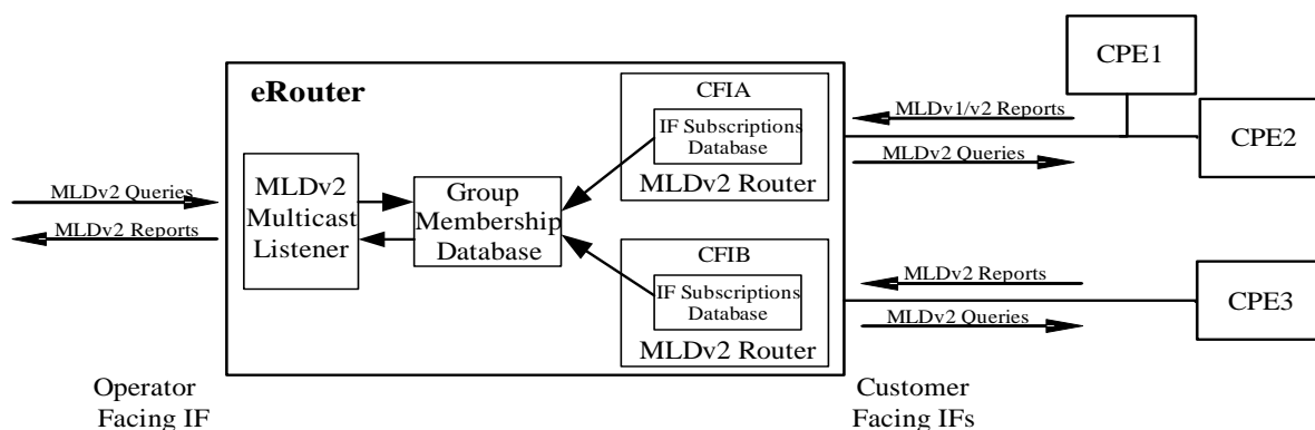
Figure 10-3 - IPv6 Multicast Forwarding Example 57
