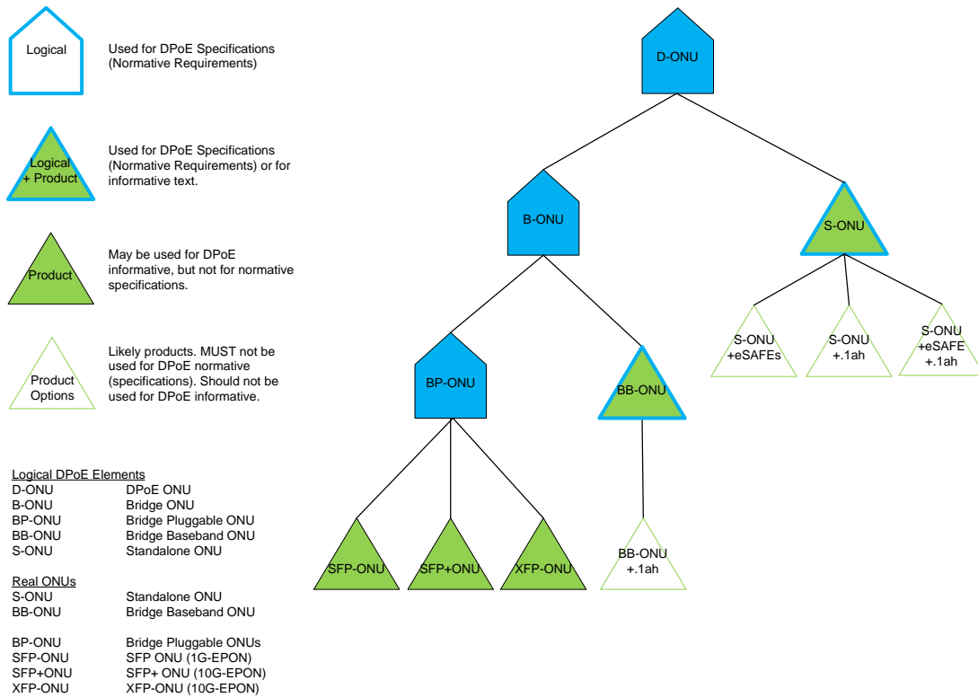
Figure 3 - D-ONU Types
