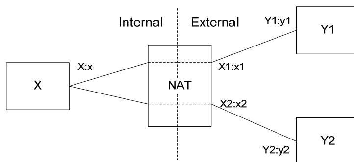
Figure 1 - Types of NATs (Address Mapping)
