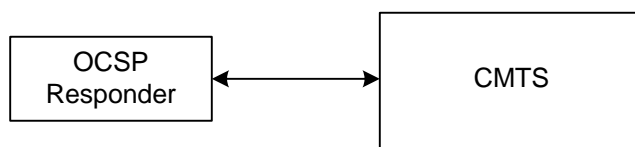
Figure 13-4 - OCSP Framework
