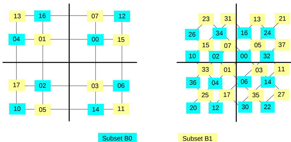
Figure 6-27 - 16 QAM and 32 QAM TCM Symbol Mapping
