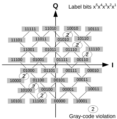
Figure 6-24 - 32 QAM Symbol Mapping
