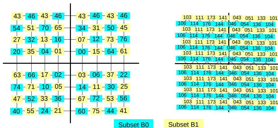
Figure 6-28 - 64 QAM and 128 QAM TCM Symbol Mapping
