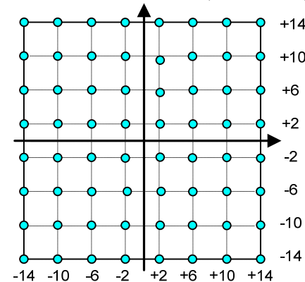
Figure 6-20 - Symbol Constellations
