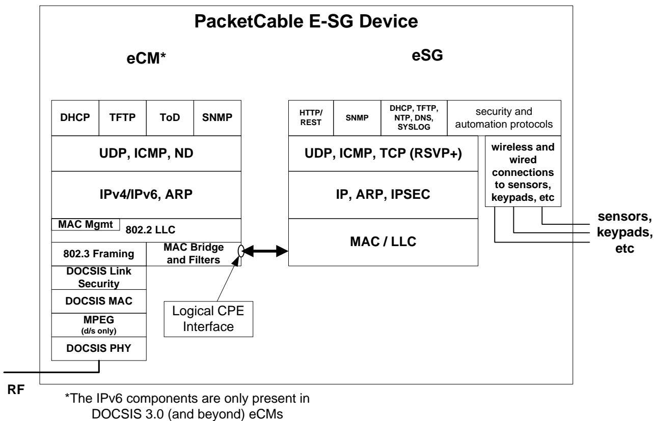
Figure 5–17 - eCM – eSG Protocol Stacks
