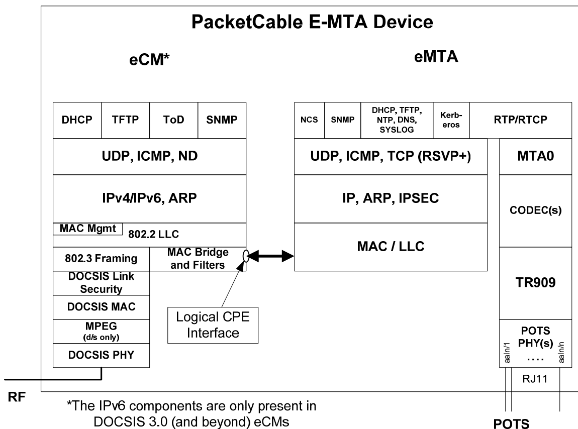
Figure 5–5 - eCM - eMTA Protocol Stacks 19
