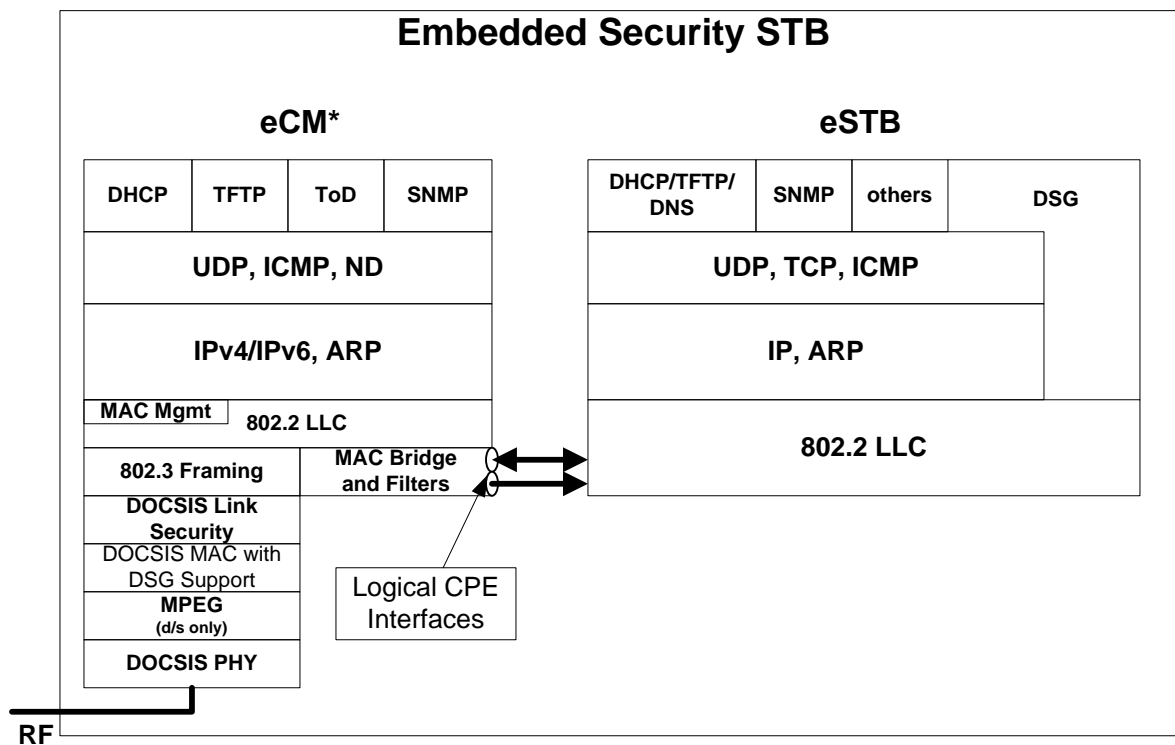
Figure 5–9 - eCM - eSTB Protocol Stacks - Embedded Security STB 24
