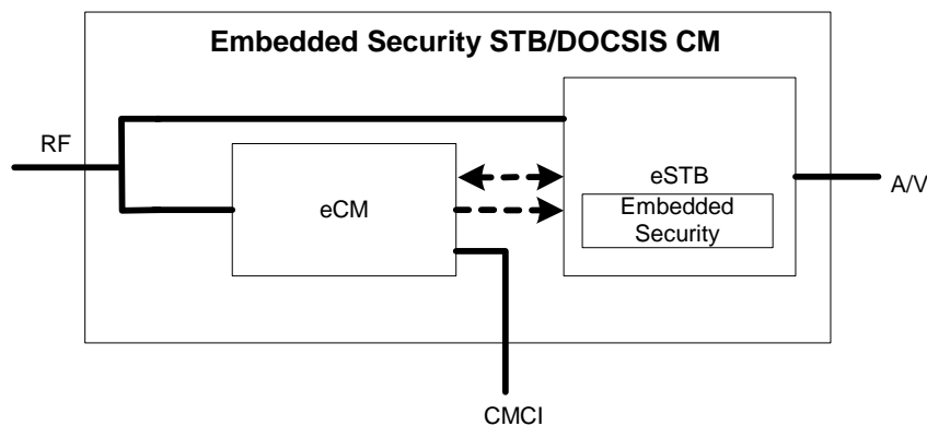
Figure 5–8 - Embedded Security STB eDOCSIS Reference Model 23
