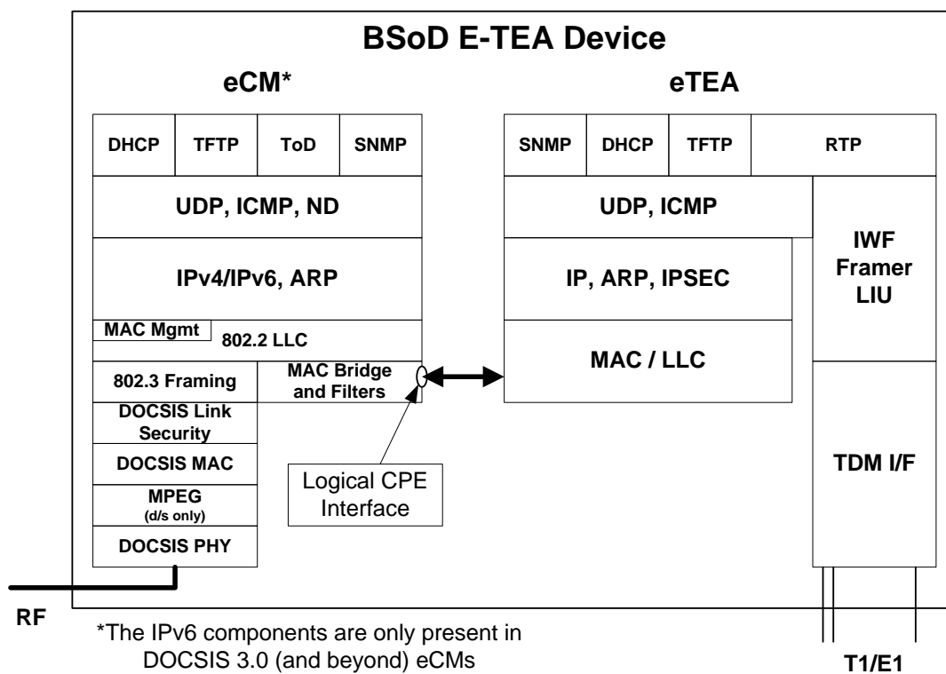
Figure 5–11 - eCM - eTEA Protocol Stacks 26
