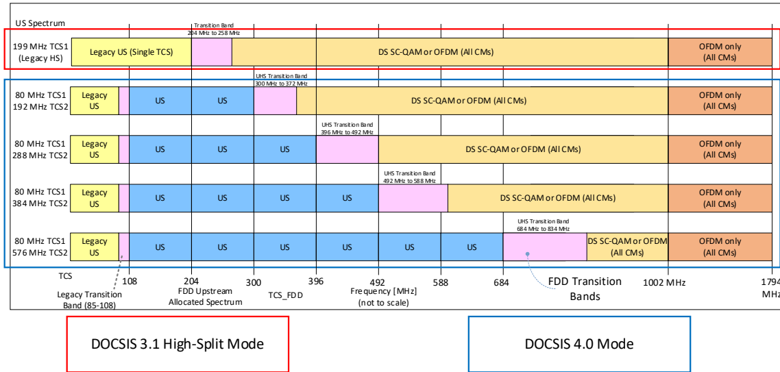
Figure 25 - Configurable FDD Upstream Allocated Spectrum Bandwidths
