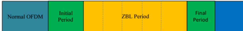
Figure 21 - ZBL Block for Echo Cancellation
