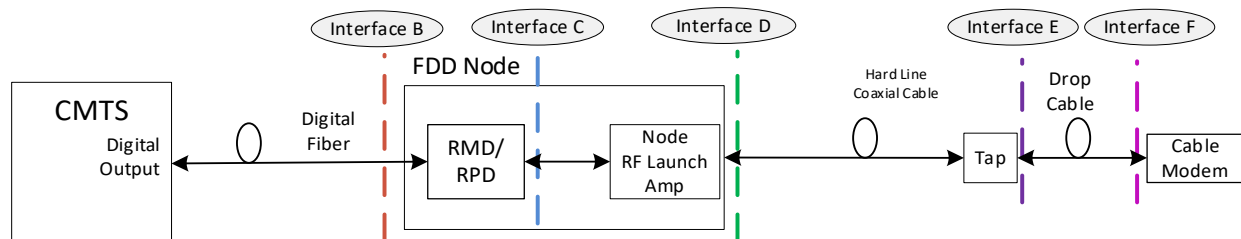
Figure 24 - FDD Node Reference Interfaces
