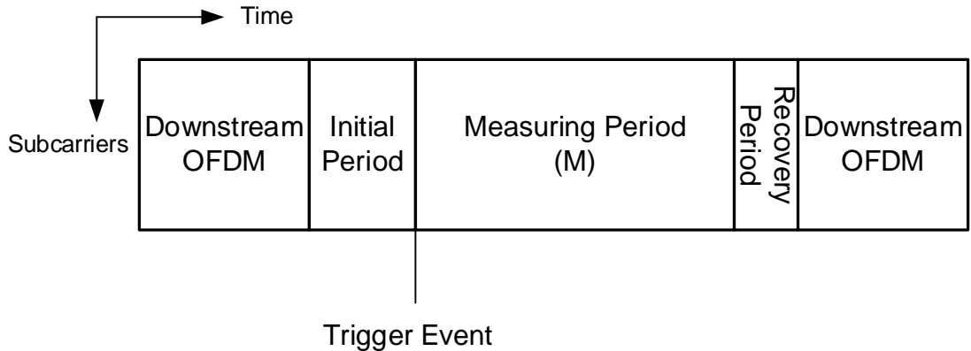
Figure 23 - Generic Triggered Measurement
