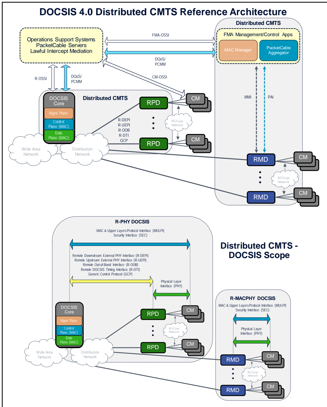
Figure 3 - DOCSIS 4.0 Distributed CMTS Reference Architecture
