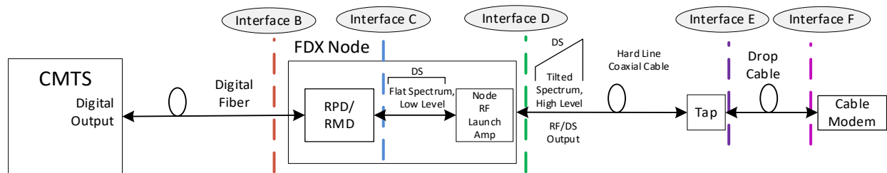
Figure 4 - Full Duplex Node Reference Interfaces
