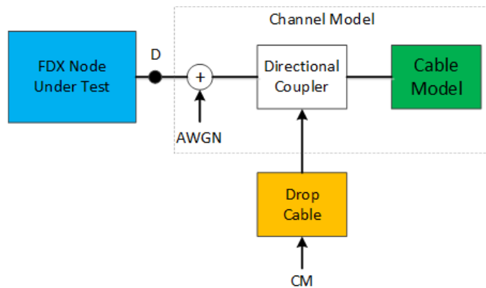
Figure 7 - Set-up for the FDX Node Packet-Error-Ratio Performance Test
