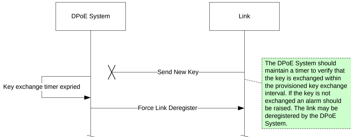
Figure 12 - Key Exchange Failure Detected By DPoE System
