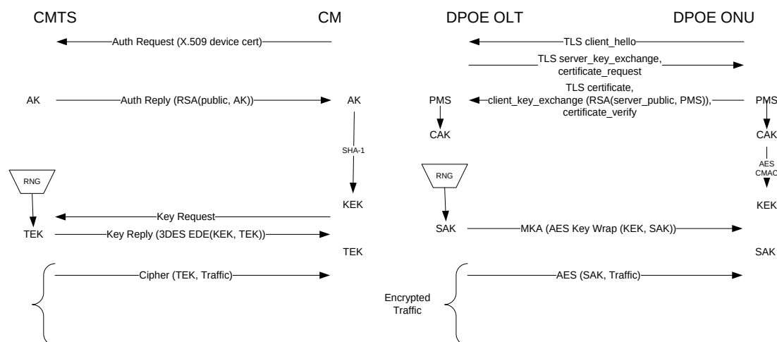
Figure 16 - Authentication in Bidirectional Methods
