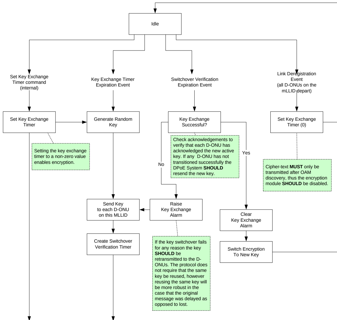
Figure 14 - mLLID Key Exchange DPoE System State Machine
