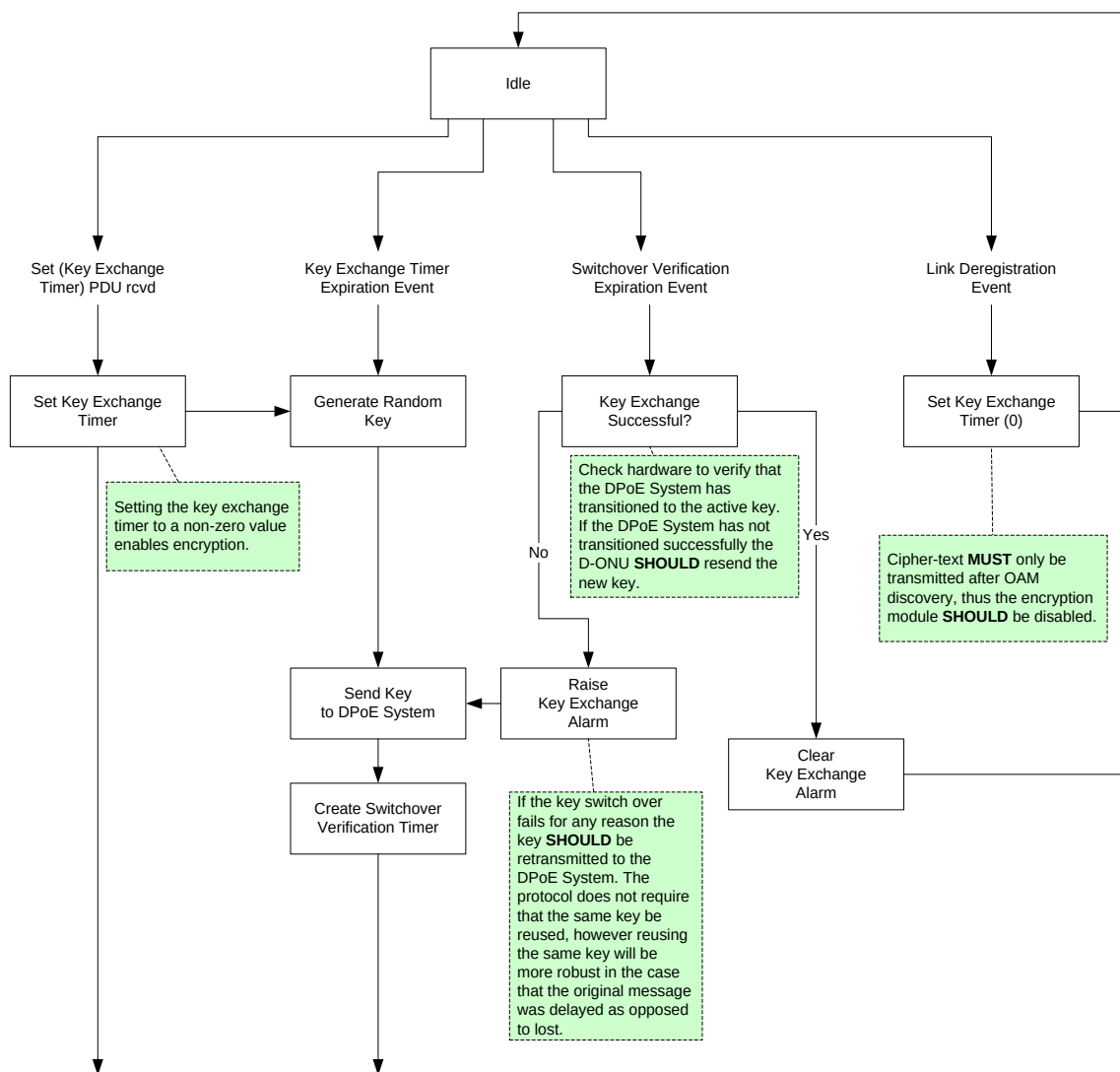
Figure 7 - D-ONU Key Exchange State Machine
