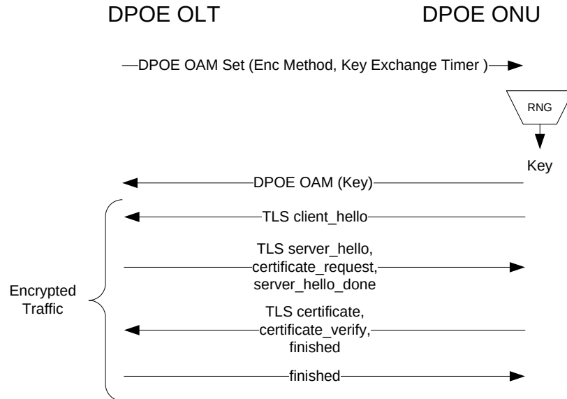
Figure 17 - Authentication in Downstream-Only Methods
