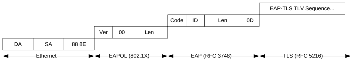
Figure 19 - EAP-TLS Frame Format
