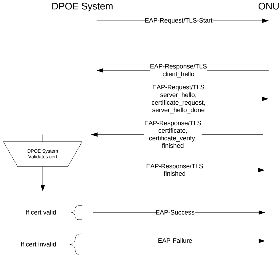
Figure 18 - EAP-TLS Message Sequence
