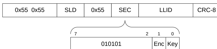
Figure 4 - Security Octet (1Down)
