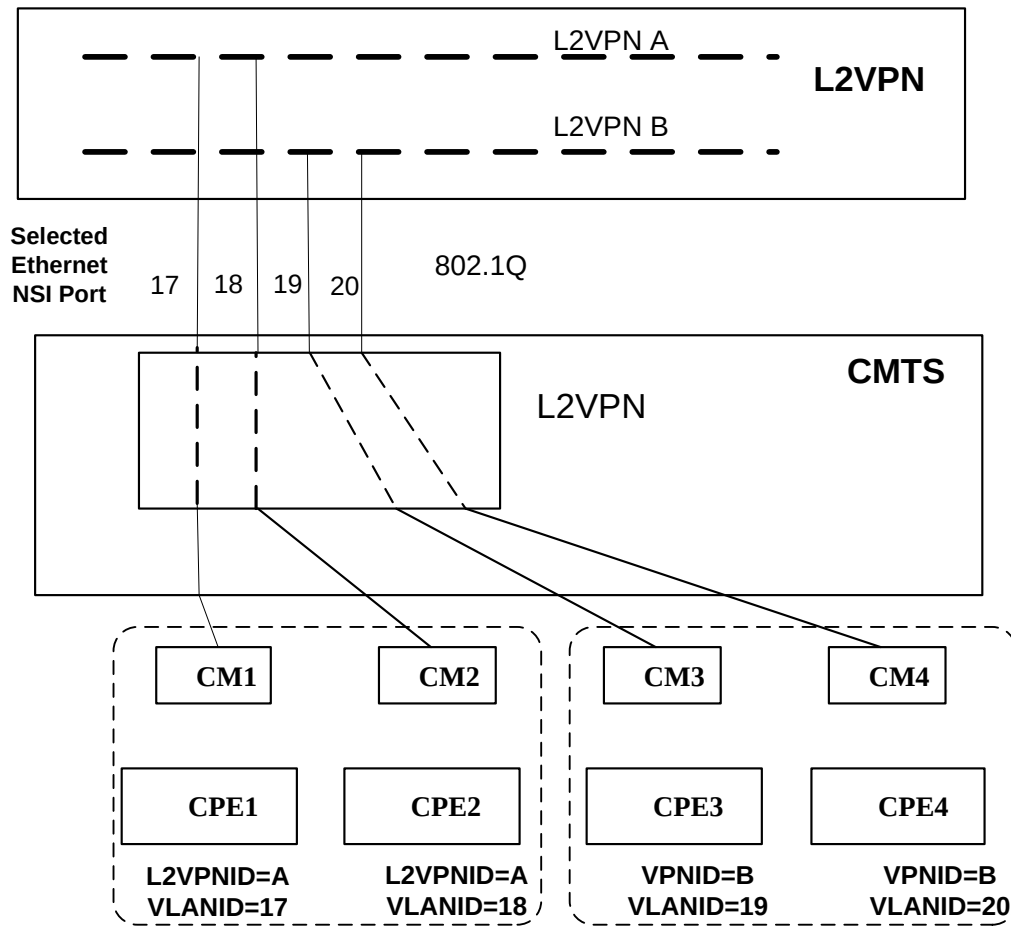
Figure 5–3 - Point-to-Point Forwarding Mode
