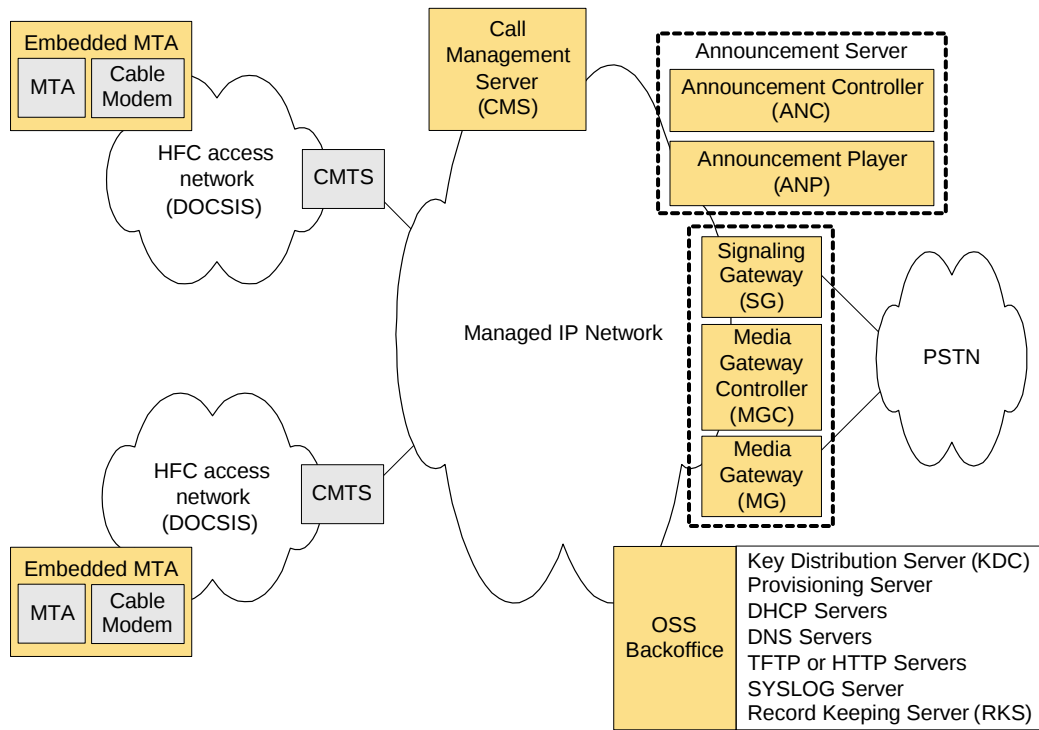
Figure 2 - PacketCable Reference Architecture
