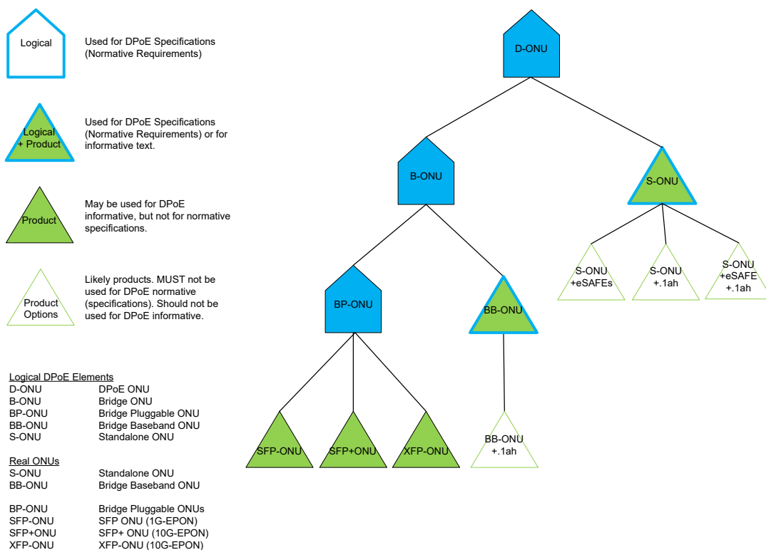
Figure 1 - D-ONU Types
