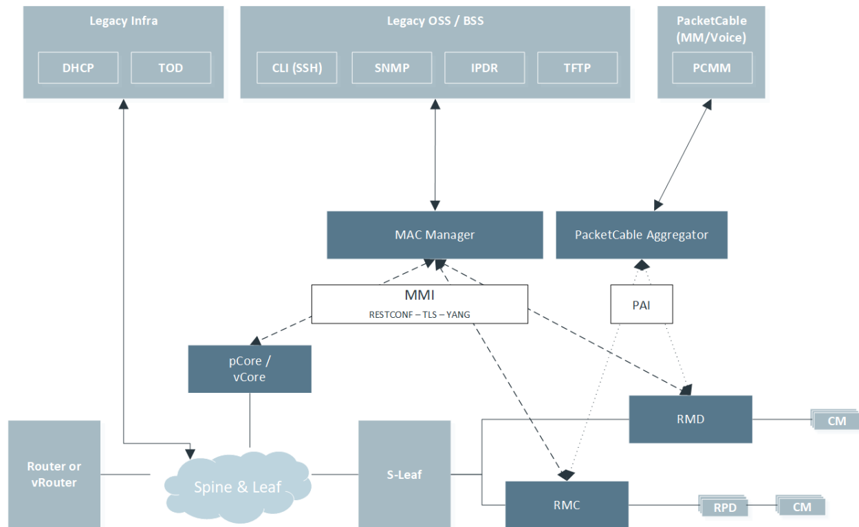
Figure 1 - FMA-MMI Overview Architecture
