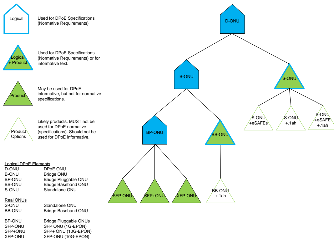
Figure 3 - D-ONU Types
