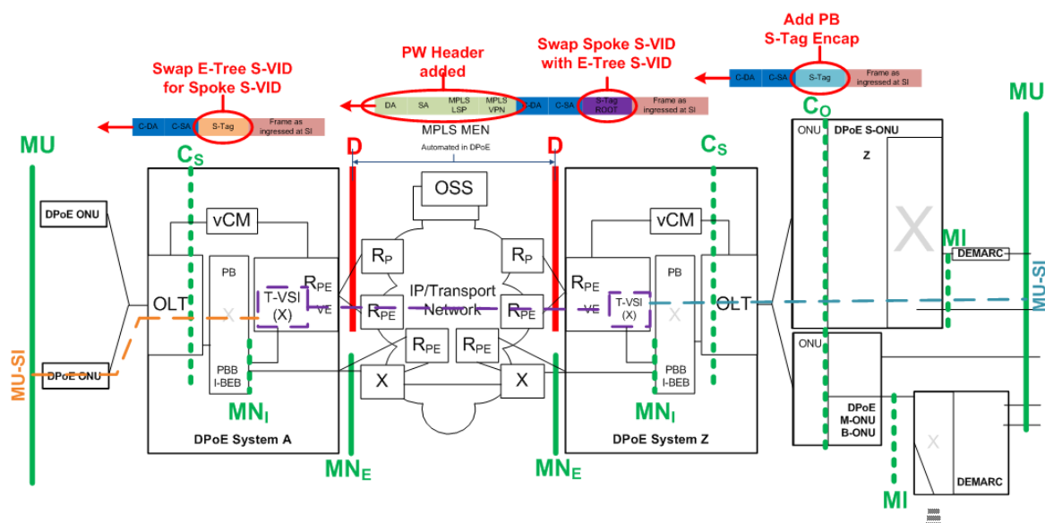
Figure 15 - E-Tree Forwarding
