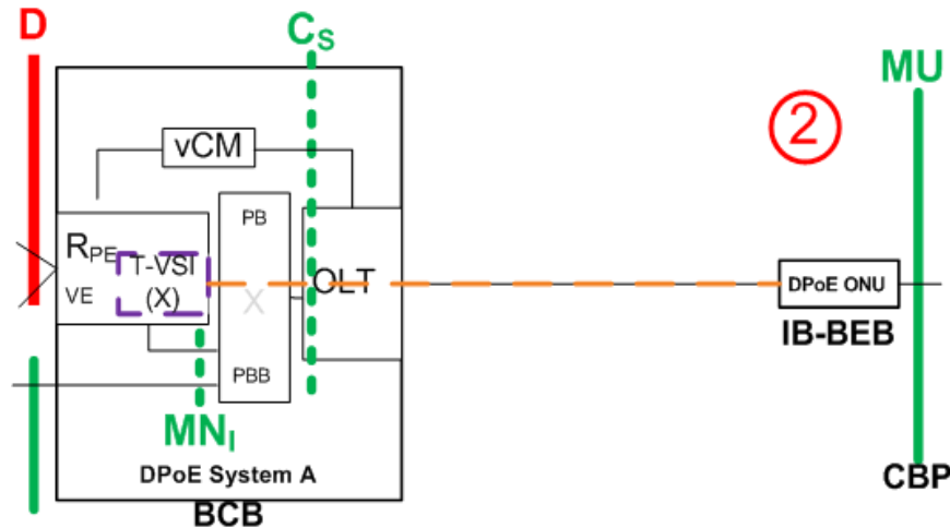
Figure 17 - PBB-D-ONU
