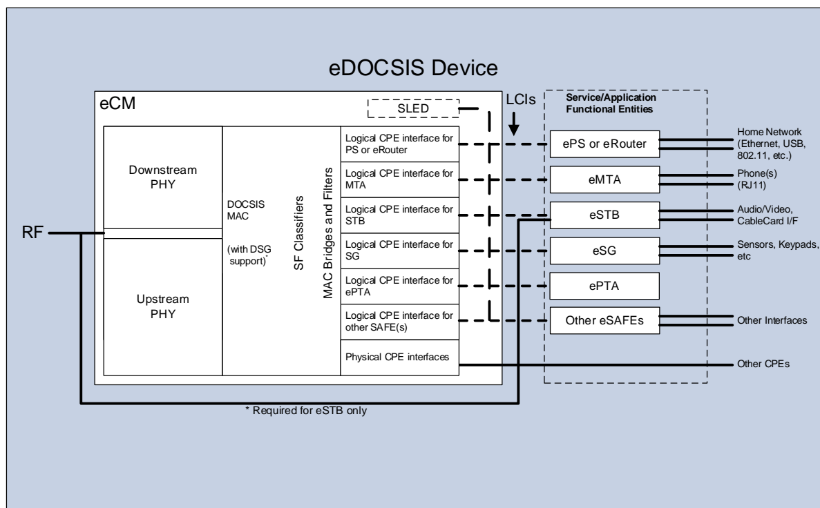
Figure 5 - eDOCSIS Reference Model (from Figure 5-1 of [eDOCSIS])
