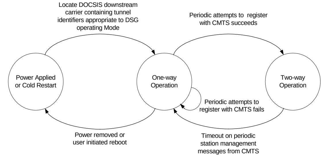
Figure 5-1 – DSG eCM State Transition Diagram
