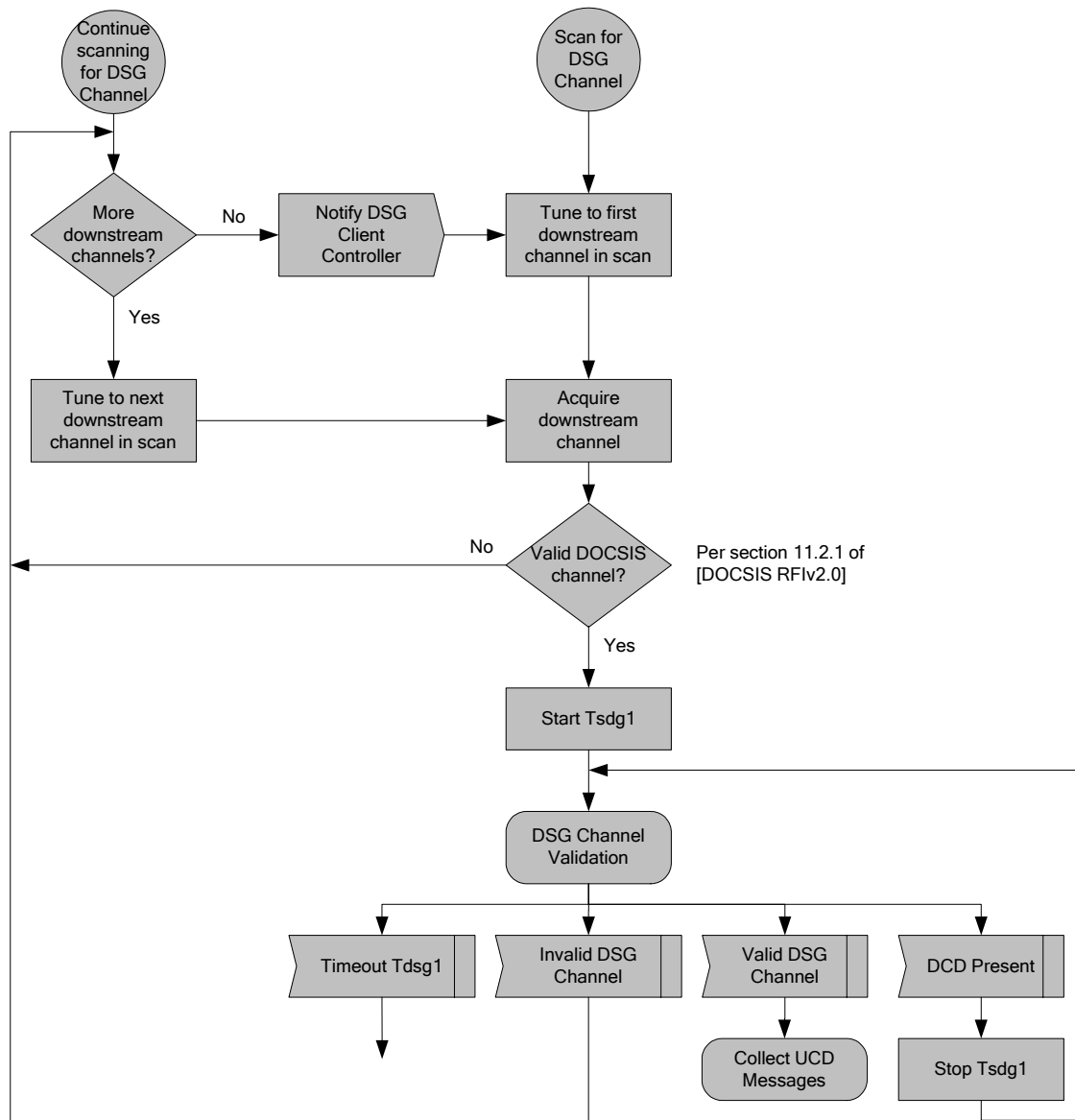
Figure 5-4 – DSG eCM Scan for Downstream DSG Channel 30
