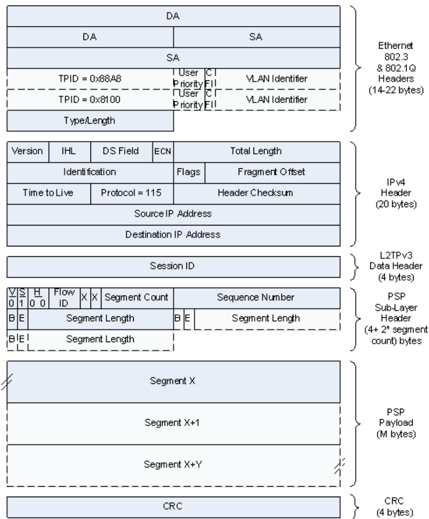
Figure 4 - UEPI IPv4 Packet with L2TPv3 Encapsulation
