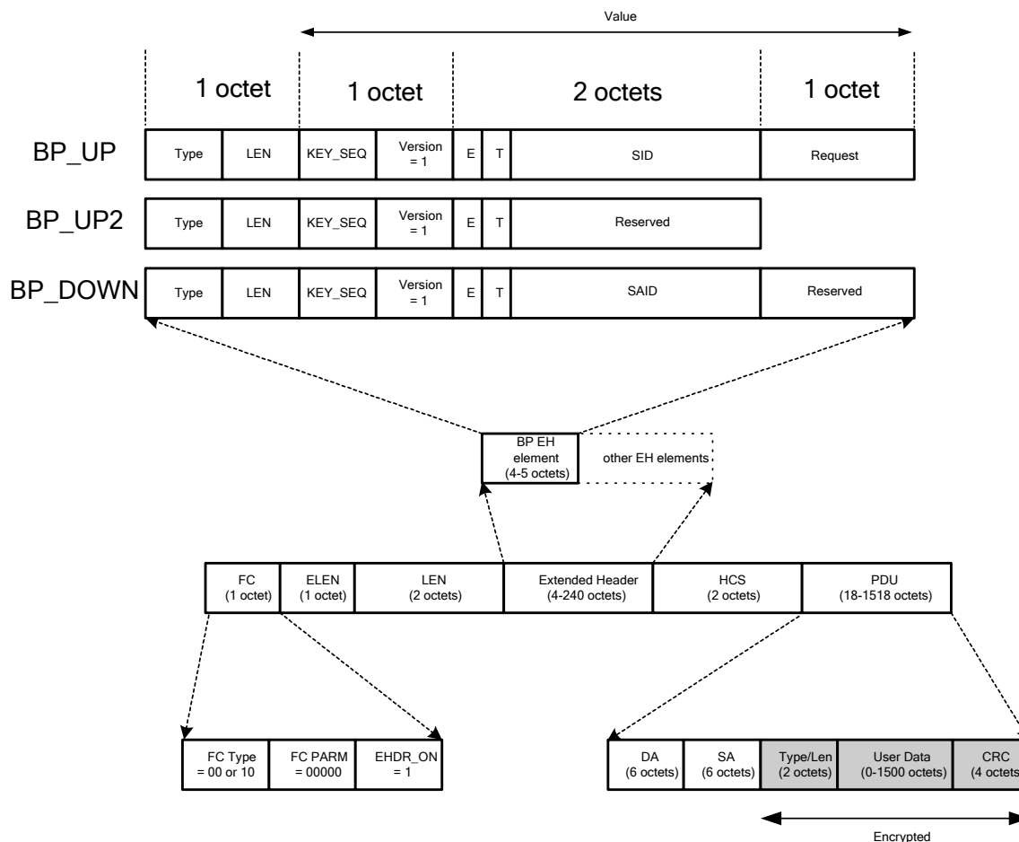
Figure 6-1 - Format of DOCSIS Variable-length PDU with Privacy EH Element 11
