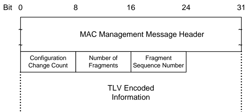
Figure 5–2 - DCD Message Fragment Structure
