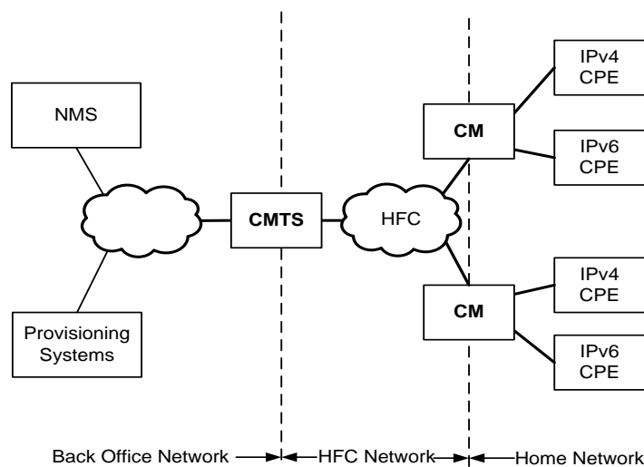
Figure 1-1 - The DOCSIS Network
