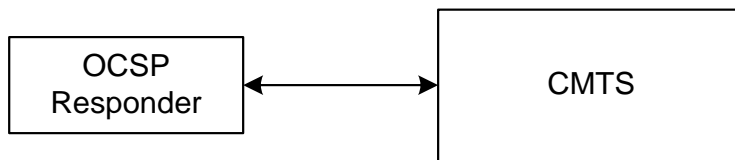
Figure 13-4 - OCSP Framework
