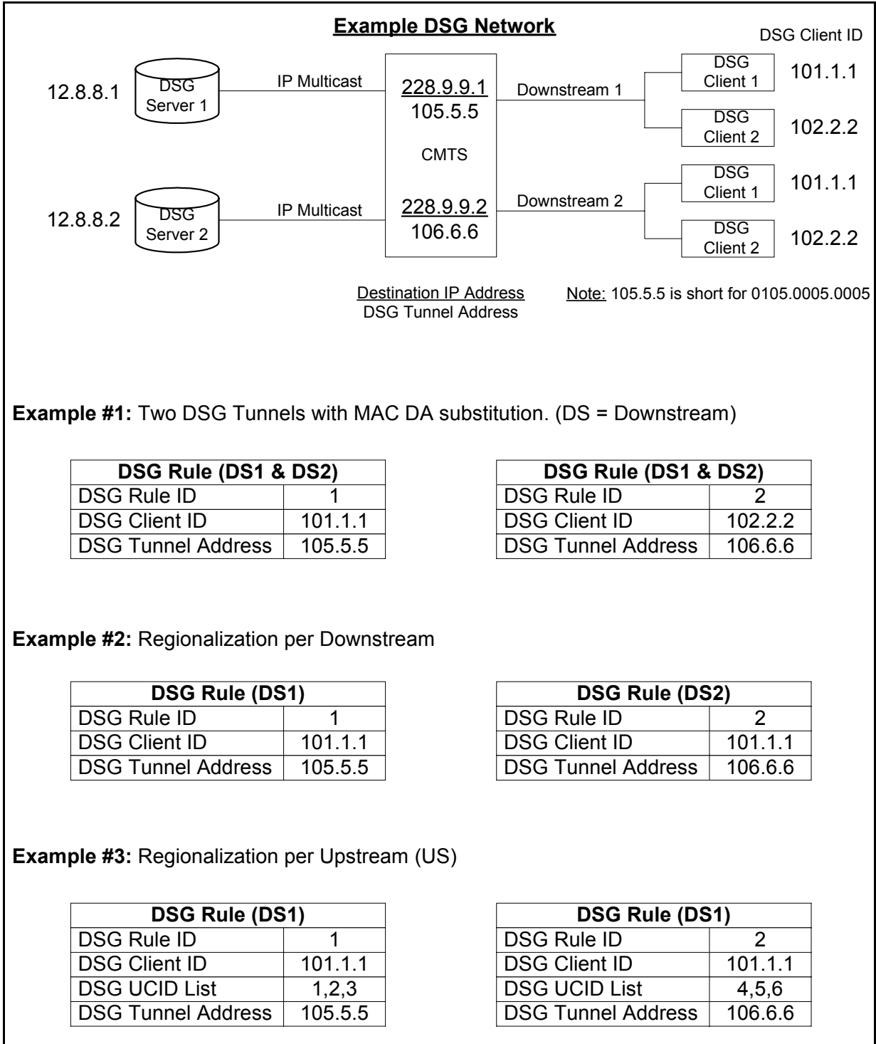
Figure 5-12 – Example DSG Configurations
