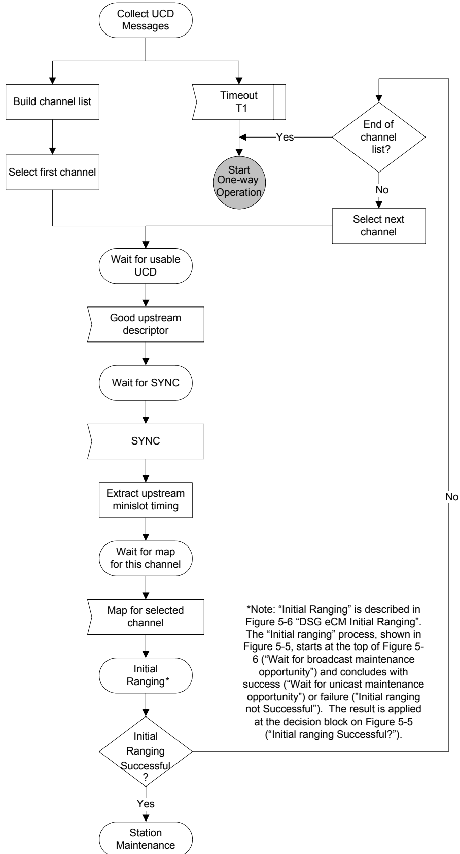
Figure 5-5 – DSG eCM Obtaining Upstream Parameters
