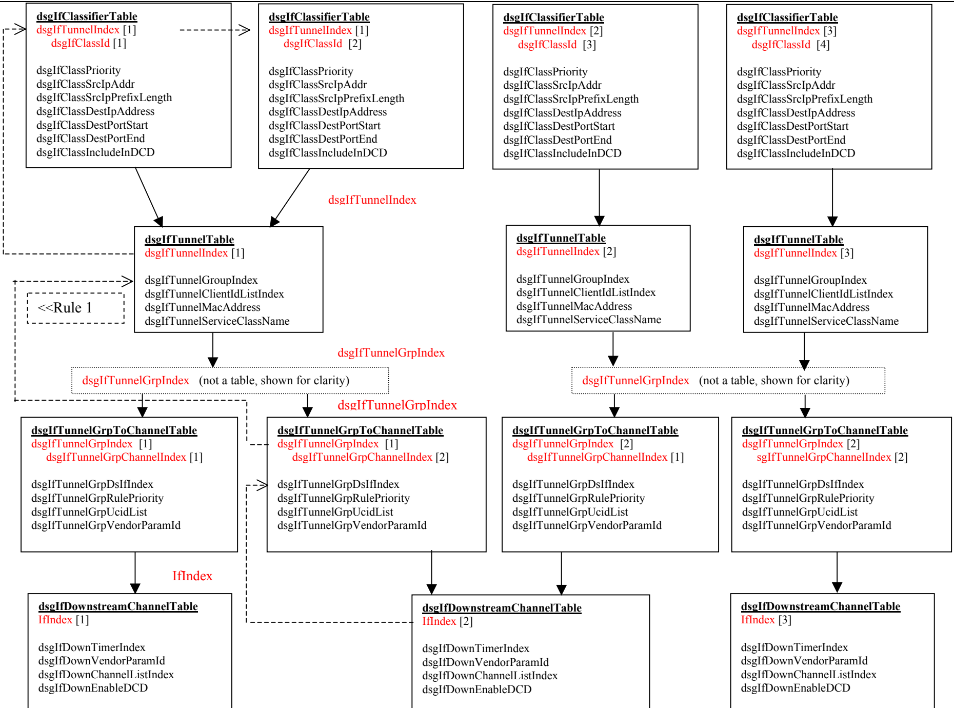
Figure I-4 – DS 2, Rule 1
