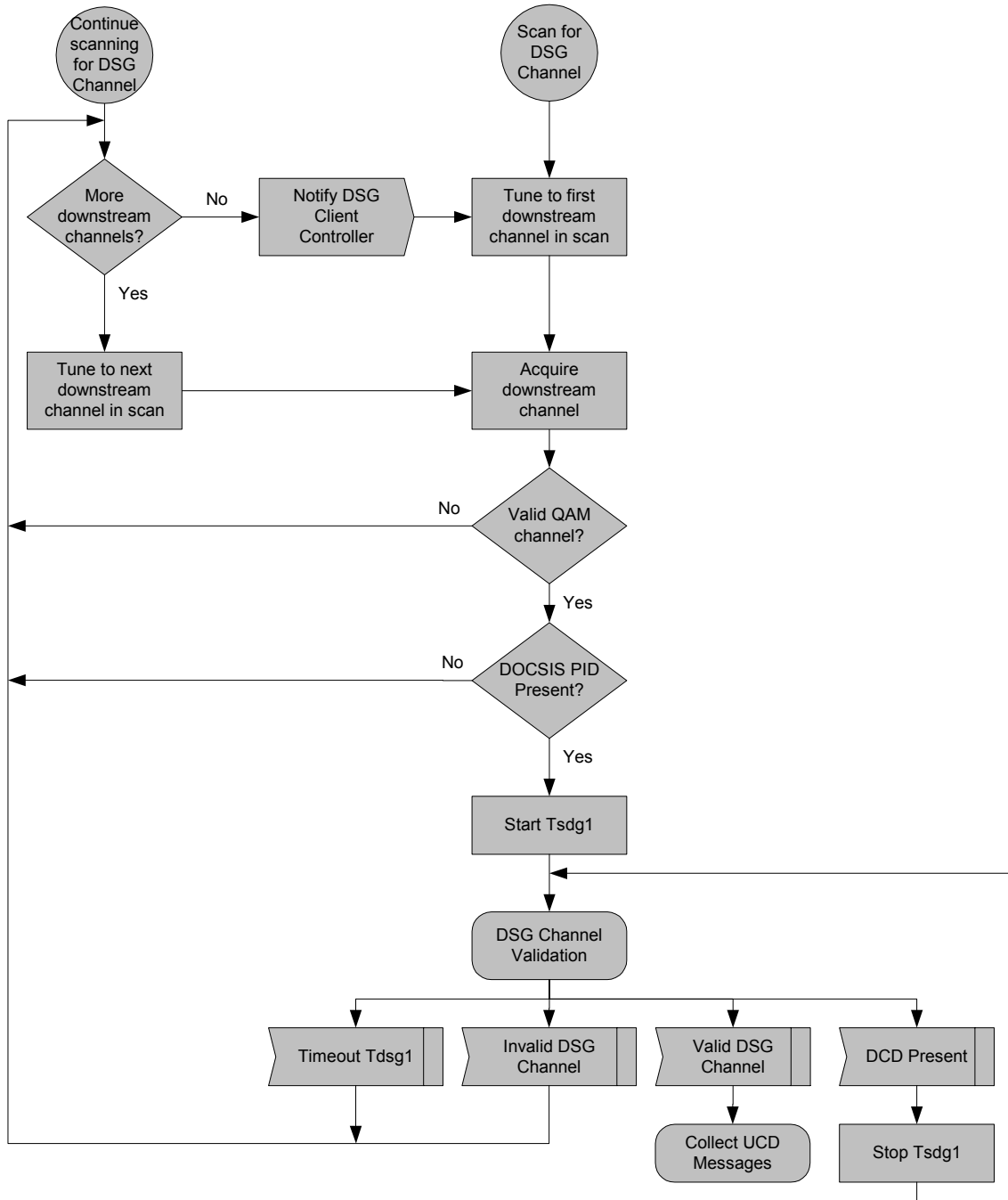
Figure 5-4 – DSG eCM Scan for Downstream DSG Channel
