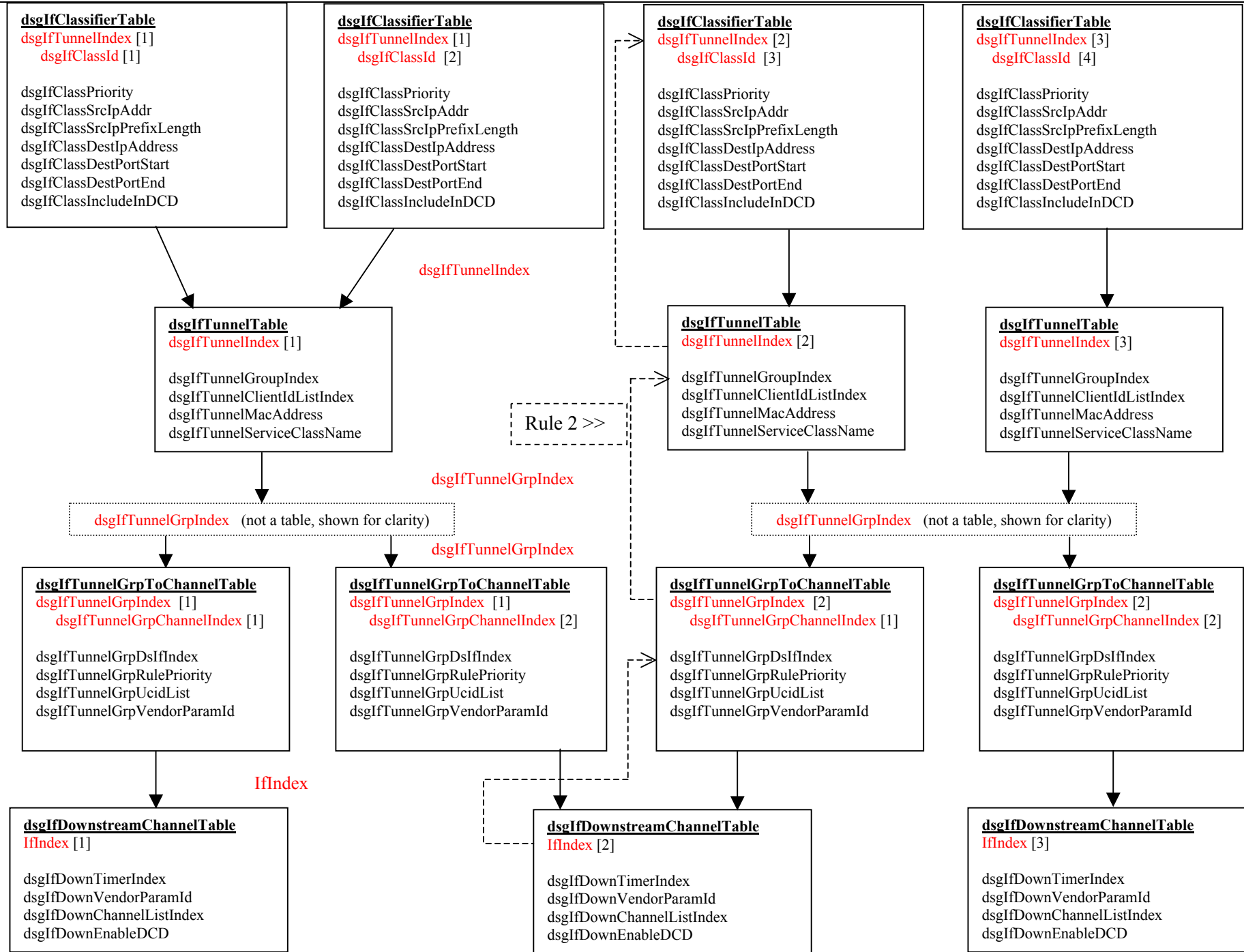
Figure I-5 – DS 2, Rule 2
