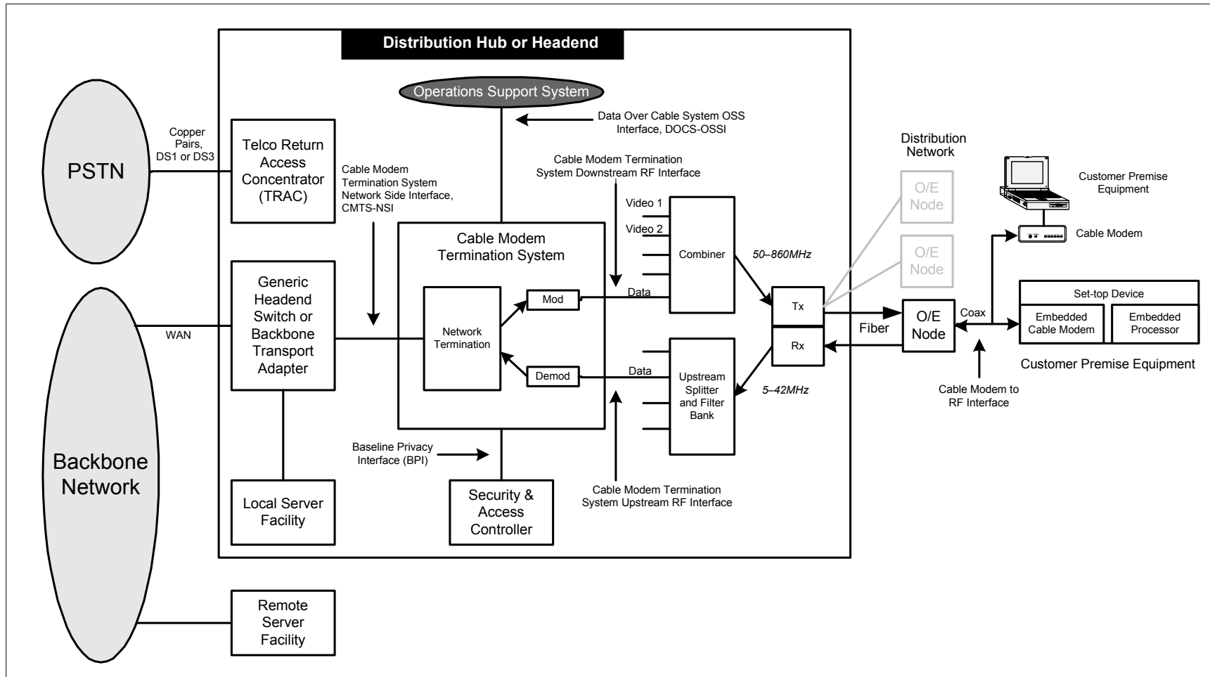
Figure 1-2 – Data-Over-Cable Reference Architecture
