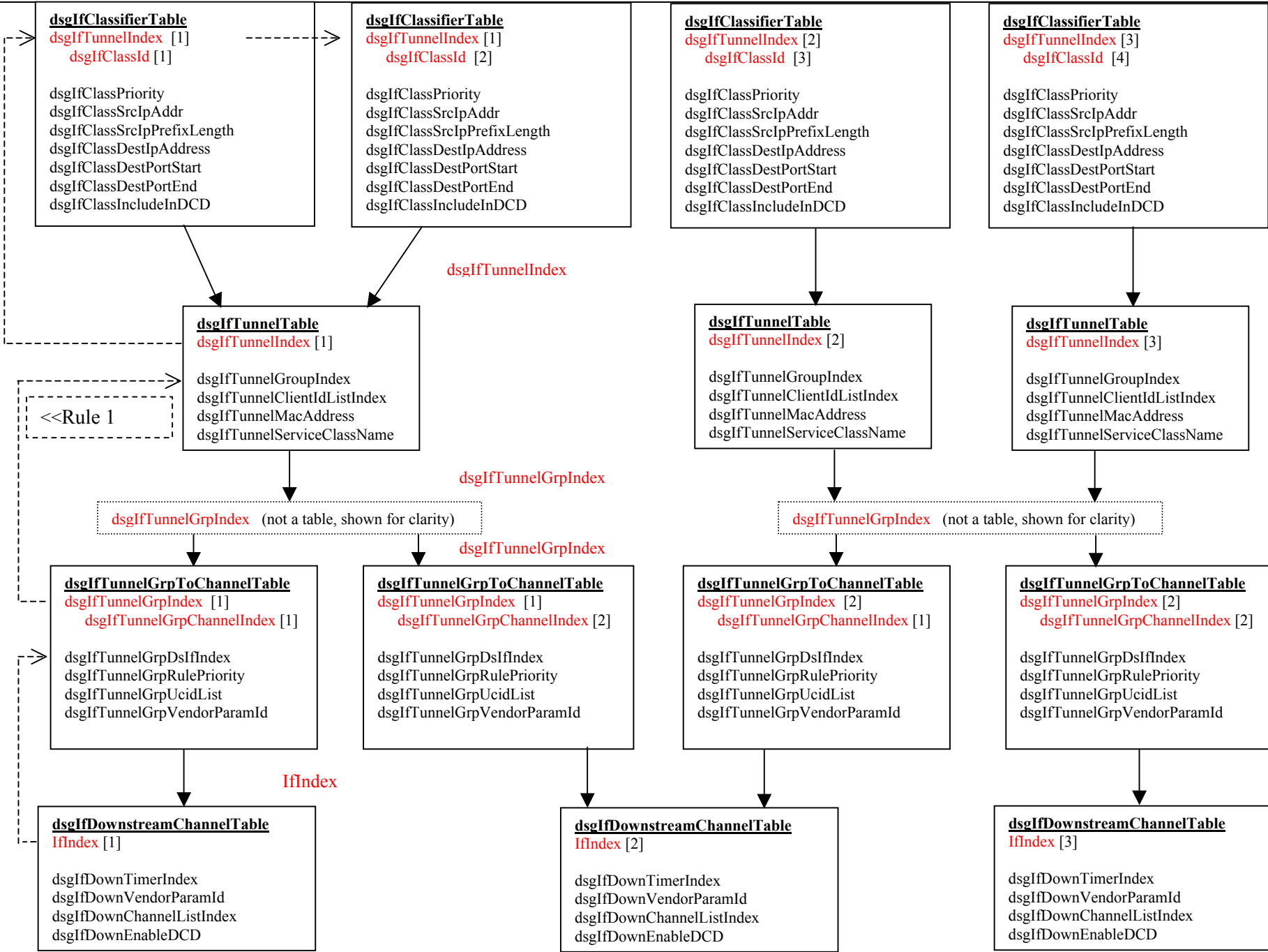
Figure I-3 – DS 1, Rule 1
