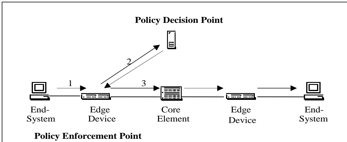
Figure 19 - COPS Protocol
