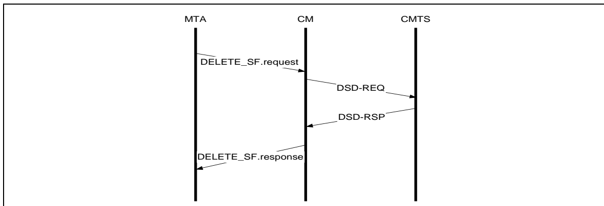
Figure 8 - Reservation Deletion
