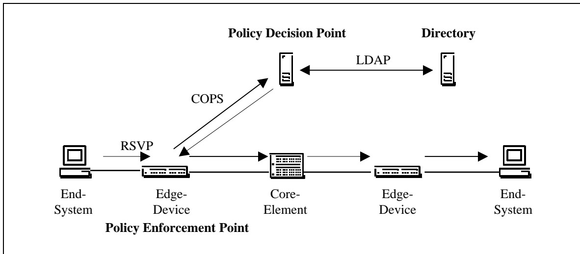
Figure 20 - COPS and LDAP model
