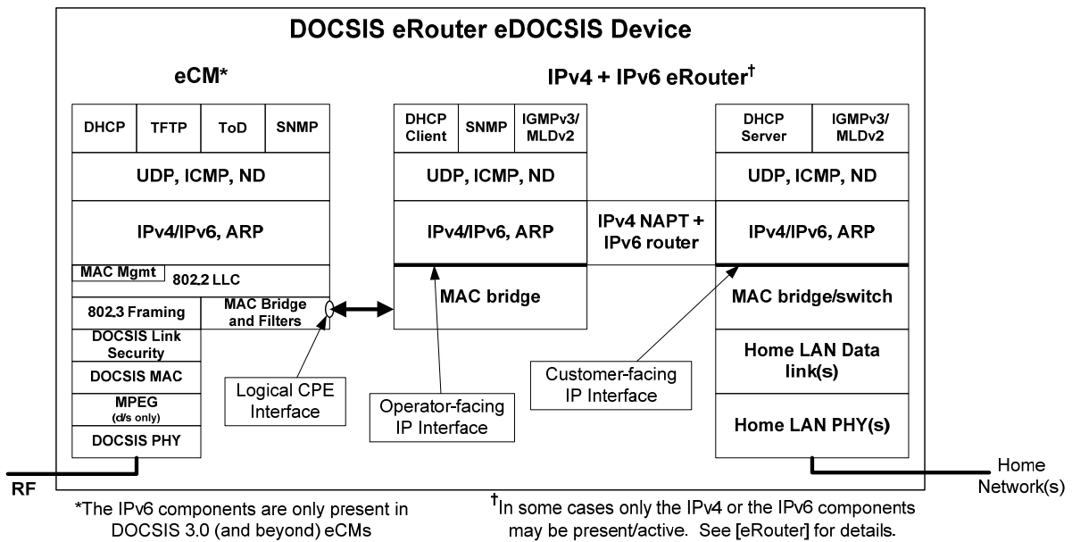
Figure 5–13 - eCM - eRouter eDOCSIS Protocol Stacks 28
