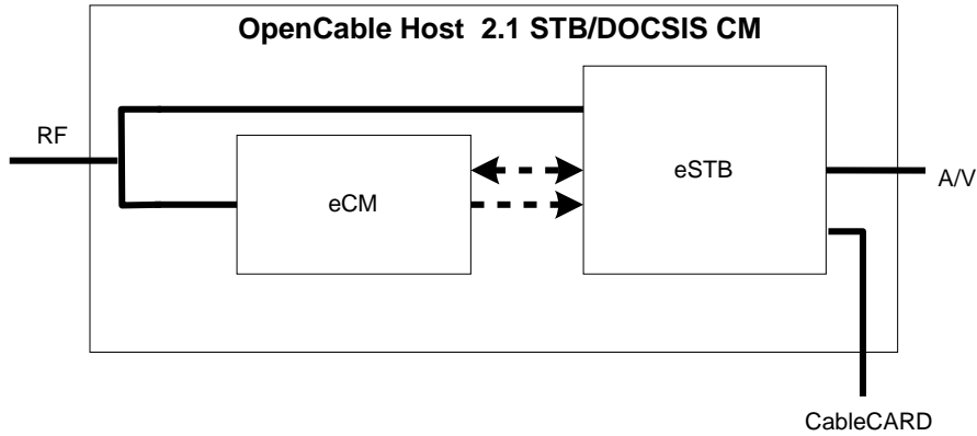
Figure 5–6 - OpenCable Host 2.1 eDOCSIS Reference Model 21
