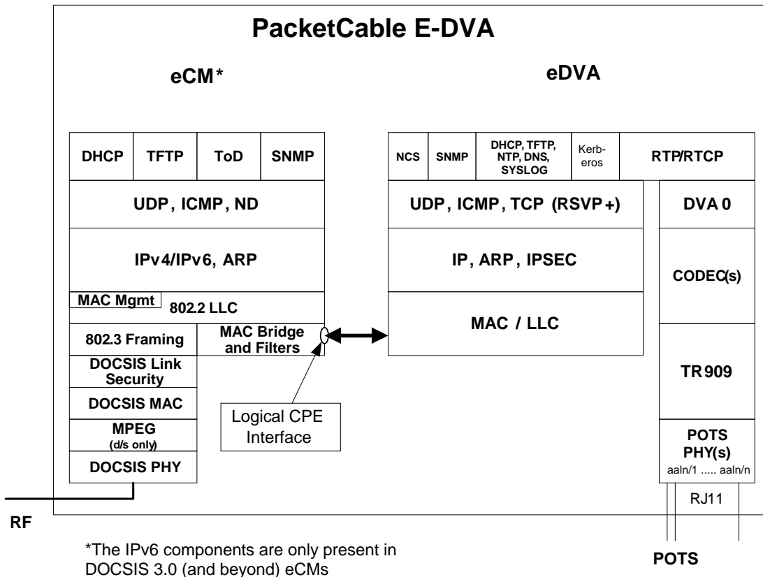
Figure 5–15 - eCM - eDVA Protocol Stacks 29
