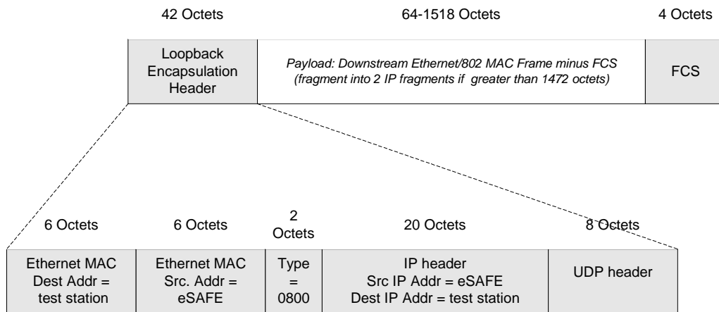
Figure 5–19 - SLED Packet Loopback Encapsulation
