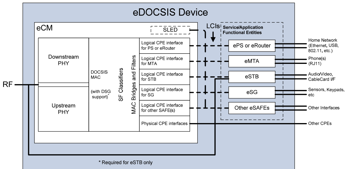
Figure 5–1 - eDOCSIS Reference Model 18
