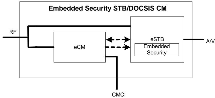
Figure 5–8 - Embedded Security STB eDOCSIS Reference Model 23
