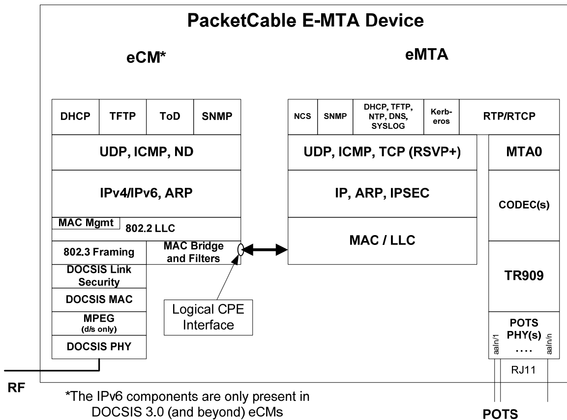
Figure 5–5 - eCM - eMTA Protocol Stacks 19
