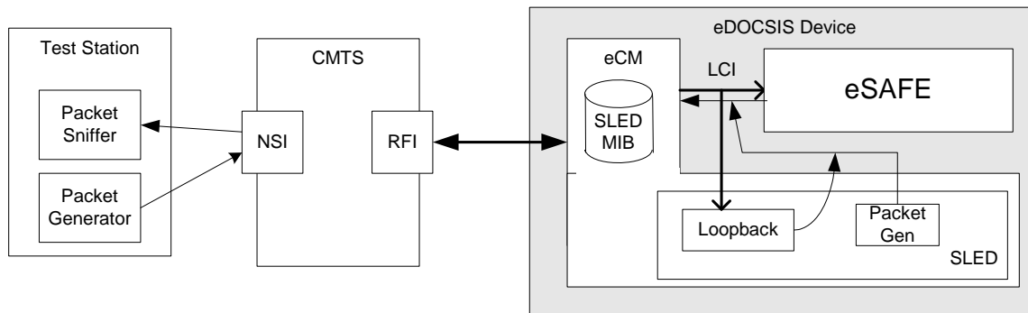
Figure 5–18 - SLED Reference Model
