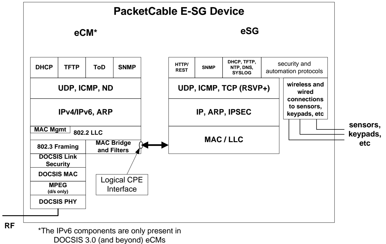
Figure 5–17 - eCM – eSG Protocol Stacks
