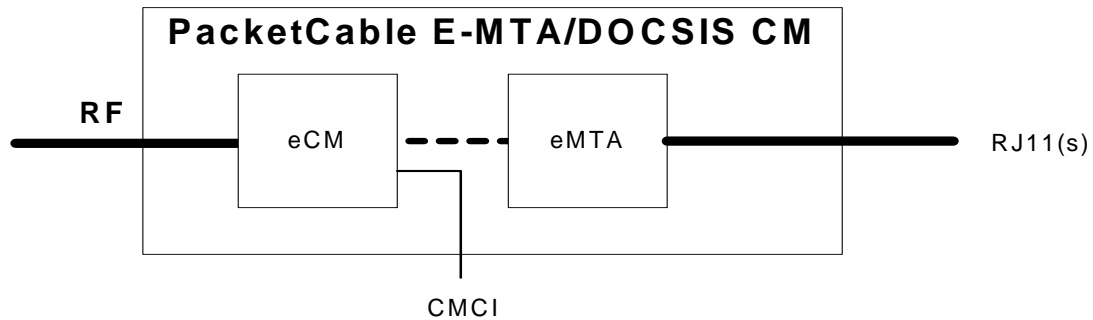
Figure 5–4 - PacketCable E-MTA (with DOCSIS CM) eDOCSIS Reference Model
