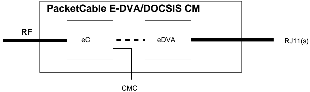
Figure 5–14 - PacketCable E-DVA (with DOCSIS CM) eDOCSIS Reference Model
