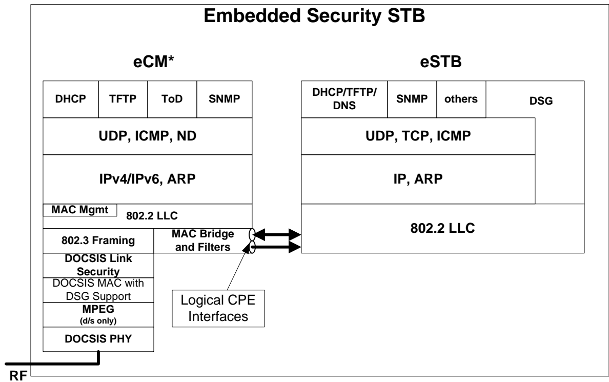
Figure 5–9 - eCM - eSTB Protocol Stacks - Embedded Security STB 24
