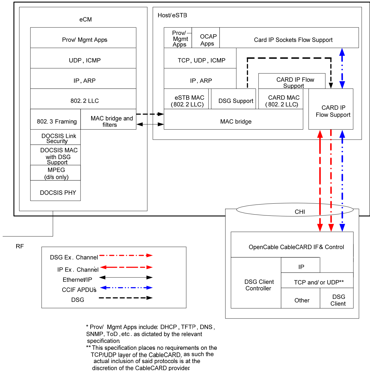
Figure 5-7 - eCM - eSTB Protocol Stacks - OpenCable Host 2.1 - Unicast IP Flow 22
