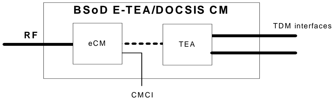
Figure 5–10 - BSoD eTEA (with DOCSIS CM) eDOCSIS Reference Model 25
