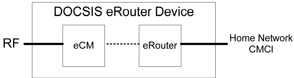
Figure 5–12 - DOCSIS eRouter eDOCSIS Device Reference Model 27
