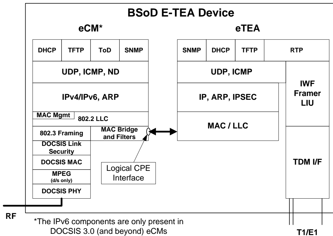
Figure 5–11 - eCM - eTEA Protocol Stacks 26
