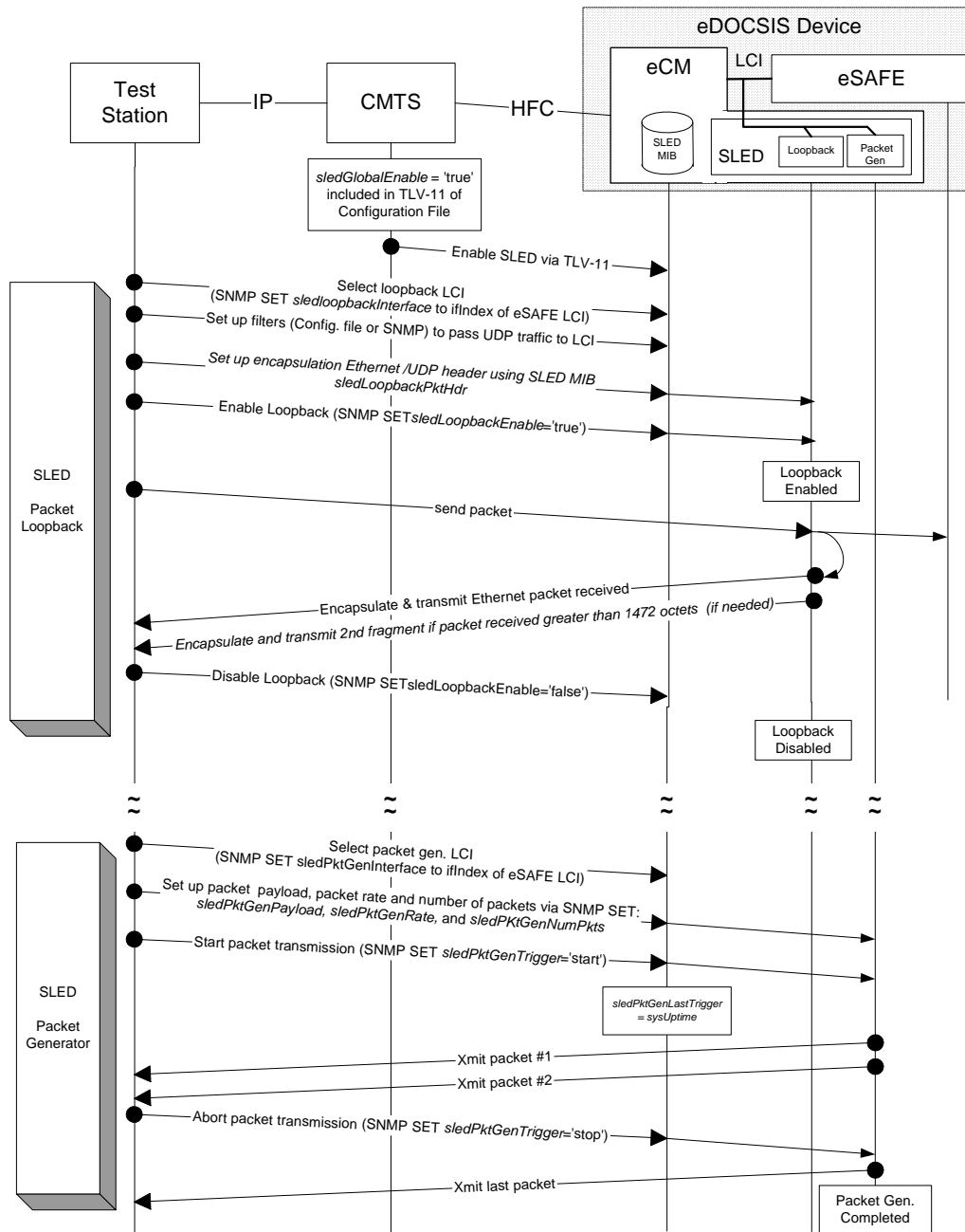
Figure 5-20 - SLED Packet Loopback And Generation Sequences
