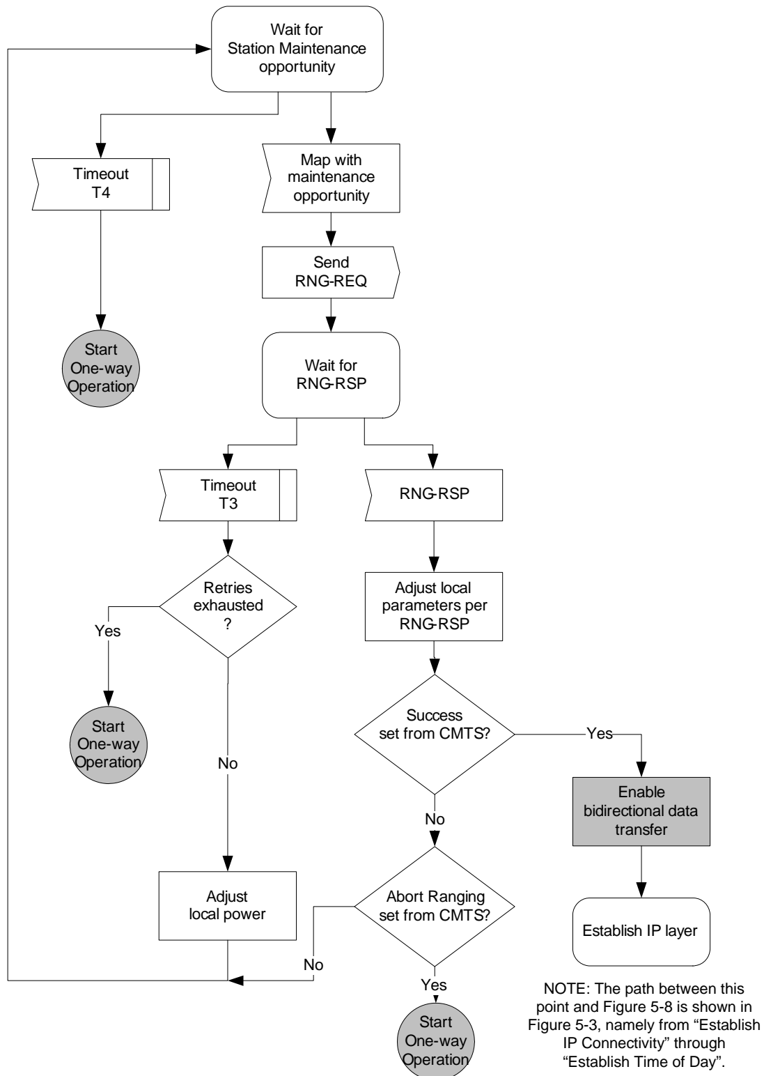
Figure 5-7 – DSG eCM Unicast Station Maintenance Ranging
