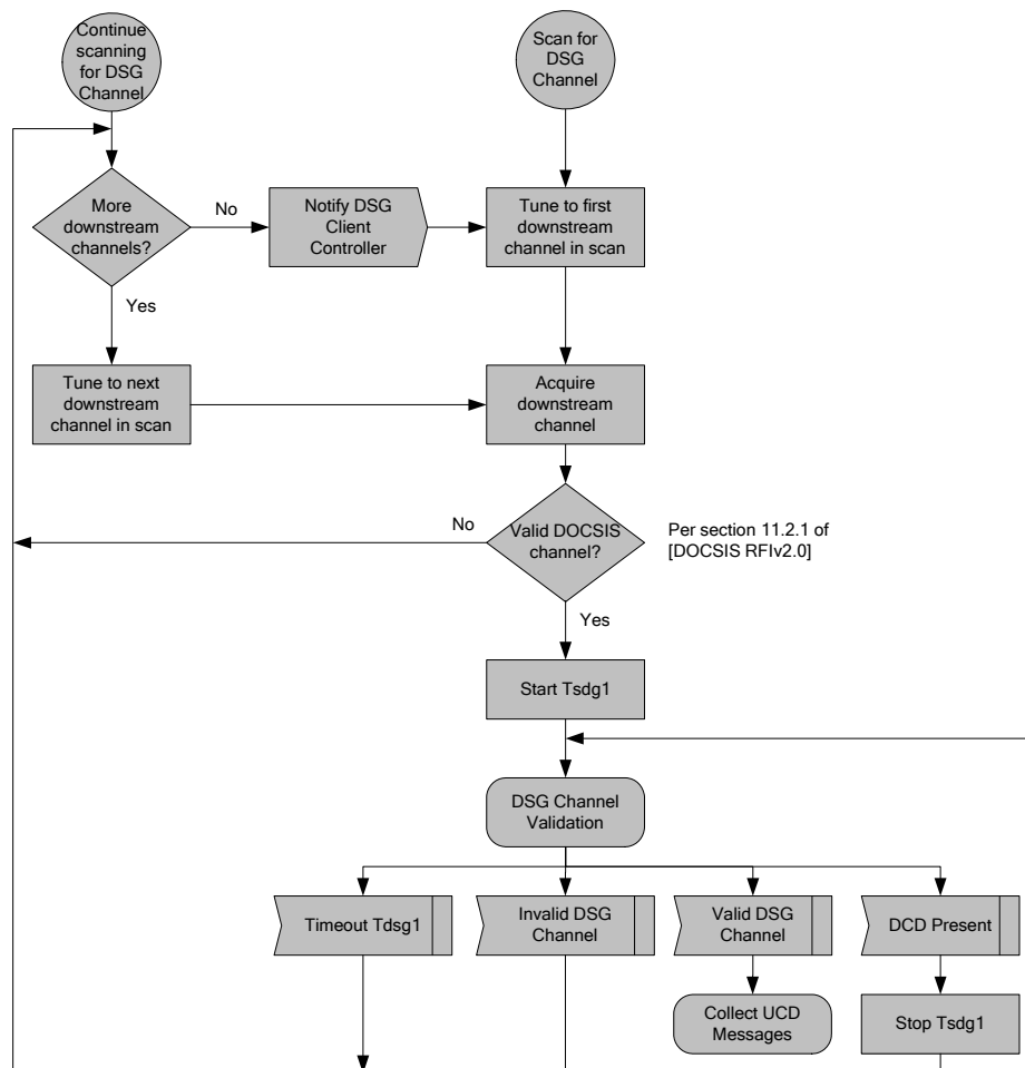
Figure 5-4 – DSG eCM Scan for Downstream DSG Channel 41
