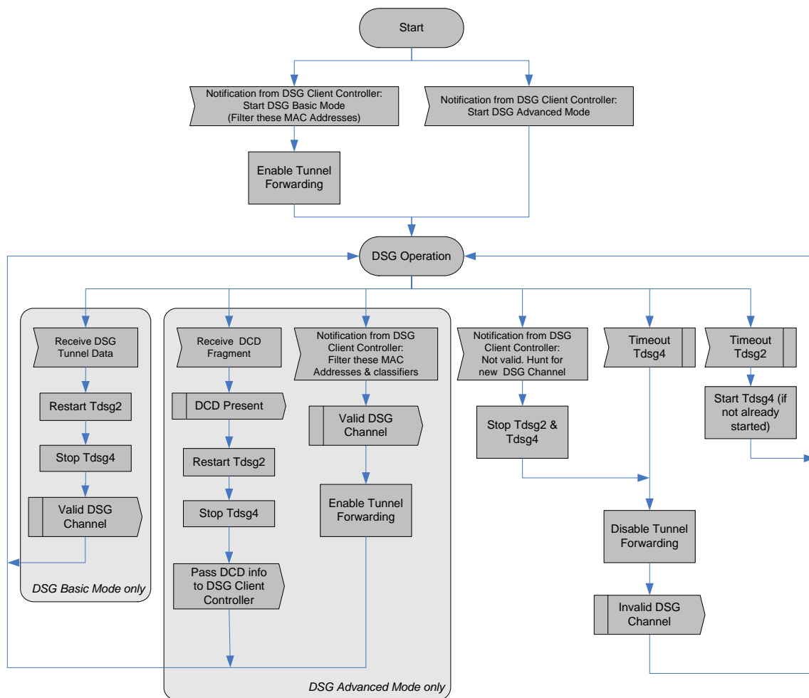
Figure 5-11 – DSG Operation
