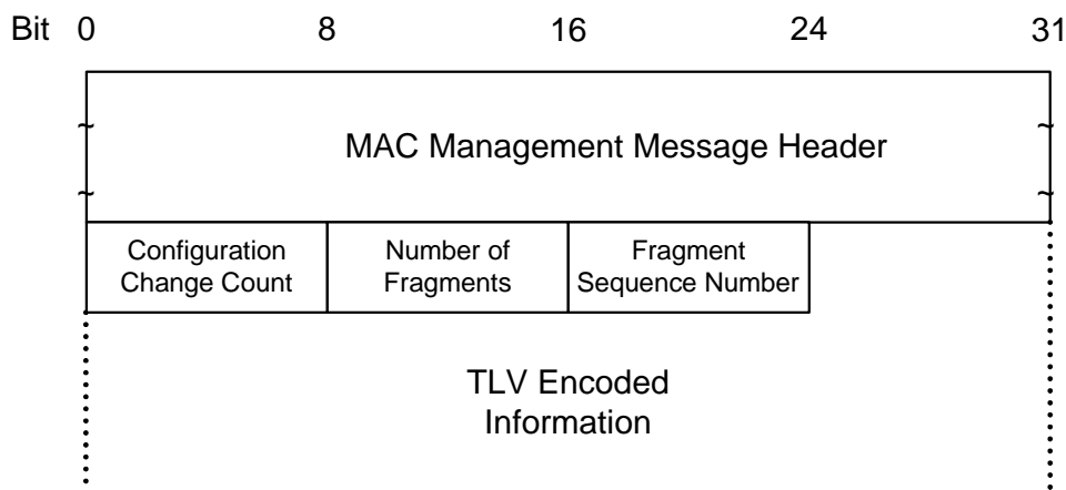
Figure 5-2 – DCD Message Fragment Structure
