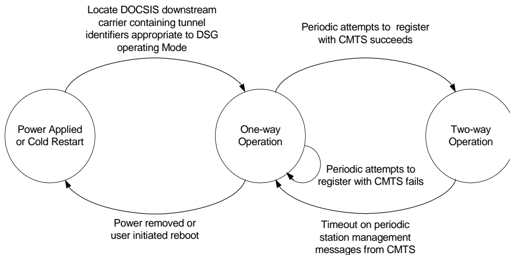
Figure 5-1 – DSG eCM State Transition Diagram
