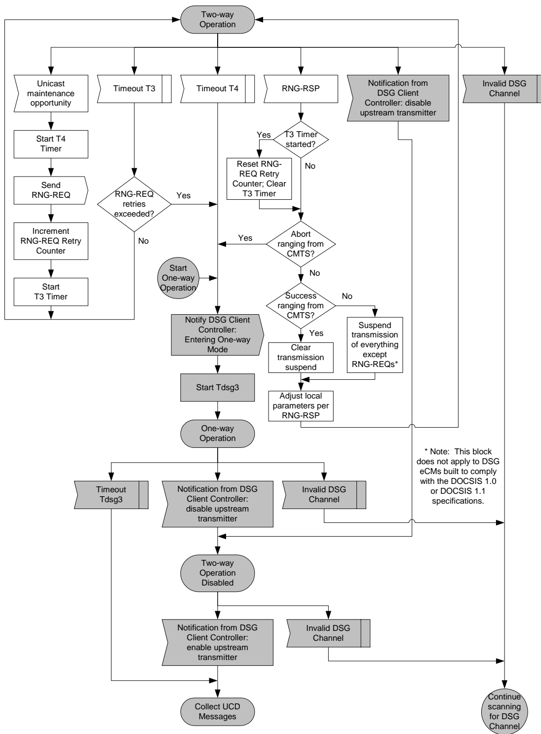
Figure 5-10 – DSG eCM Operation
