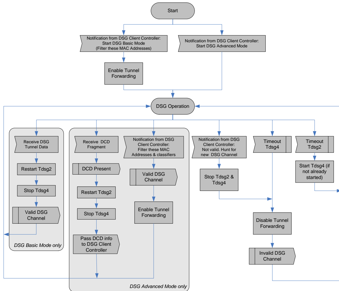
Figure 5-11 – DSG Operation
