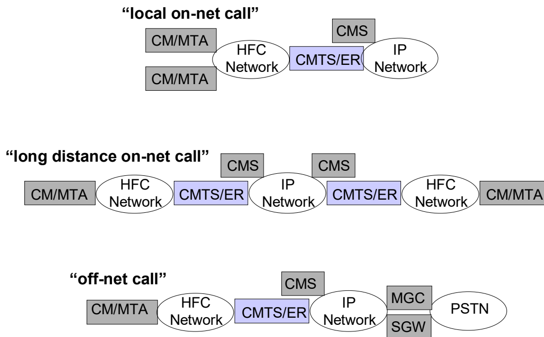
Figure 2. Critical Signaling Path Network Elements
