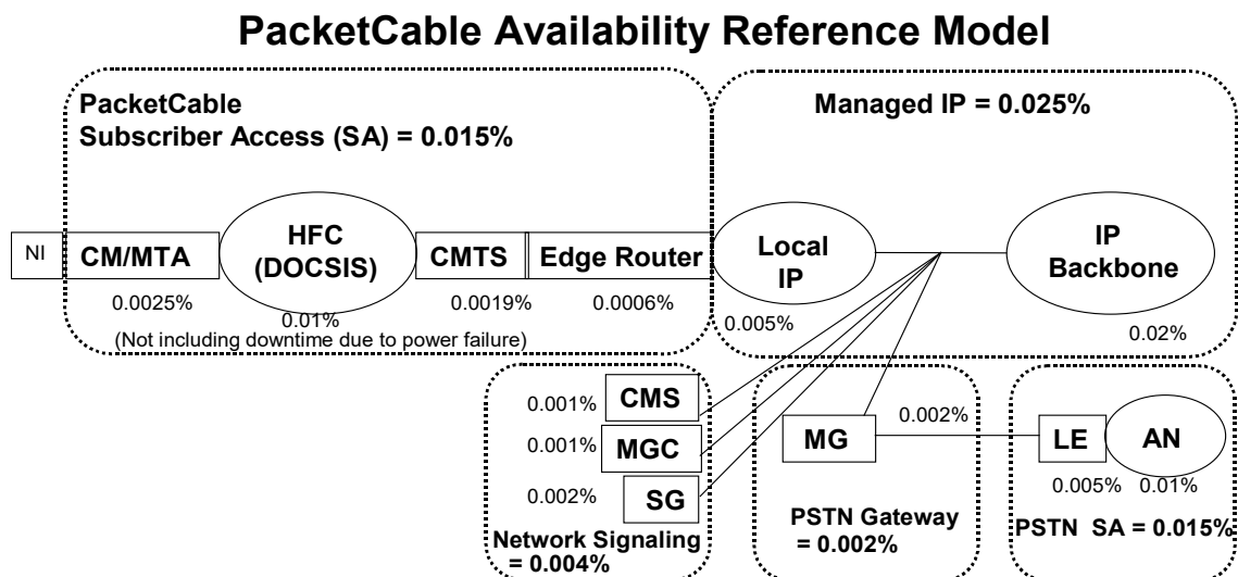
Figure 6. PacketCable Availability Model
