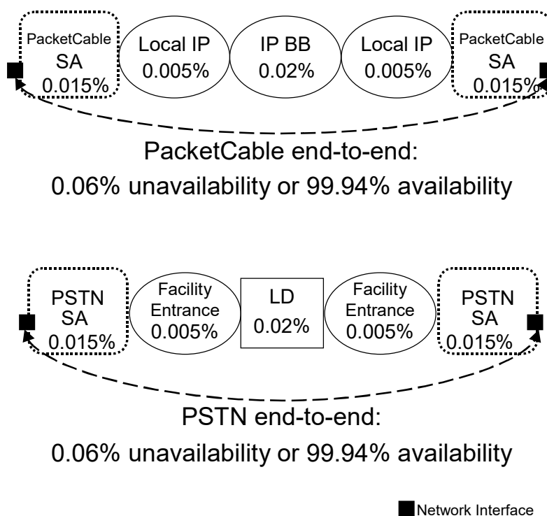
Figure 7. PacketCable End-To-End Reference Model
