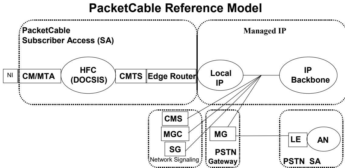
Figure 4. PacketCable Reference Model
