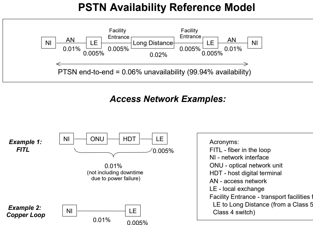
Figure 3. PSTN Reference Model
