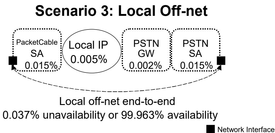
Figure 10. Scenario 3: Local Off-net Availability
