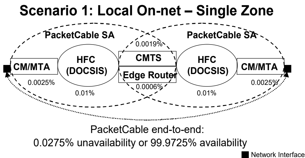
Figure 8. Scenario 1: Local On-net Single Zone Availability
