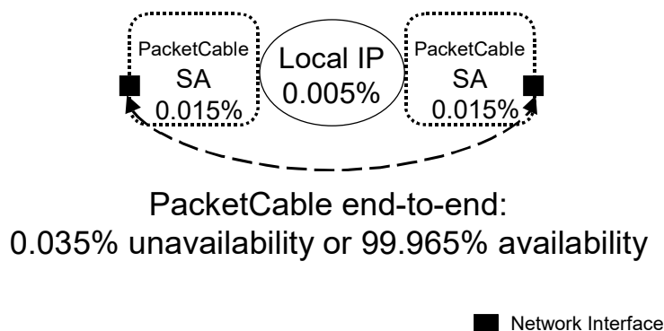
Figure 9. Scenario 2: Local On-net Multi-zone Availability
