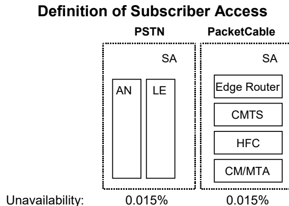
Figure 5. Definition of Subscriber Access
