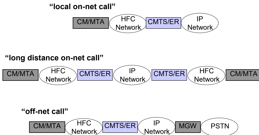
Figure 1. Critical Bearer Path Network Elements
