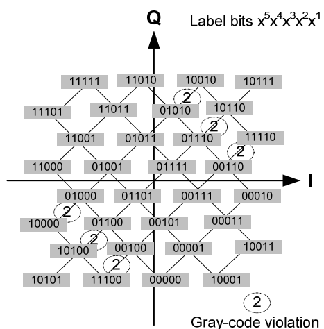
Figure 6-24 - 32-QAM Symbol Mapping 9
